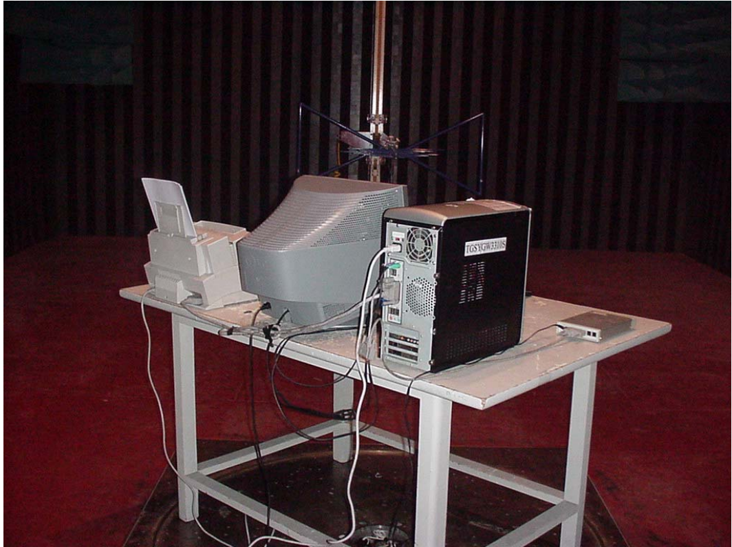
SETUP WITH MAXIMUM DETECTED EMISSION AT HORIZONTAL POLARIZATION (1024*768@85Hz)
