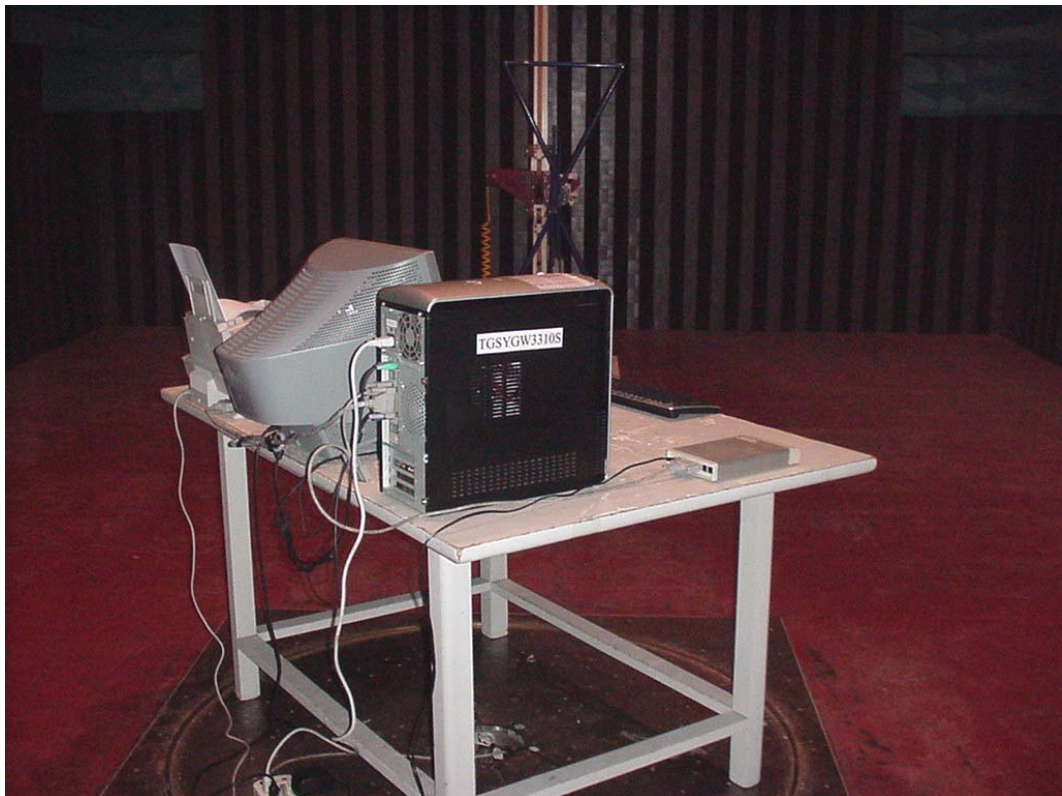
SETUP WITH MAXIMUM DETECTED EMISSION AT VERTICAL POLARIZATION (800*600@60Hz)
