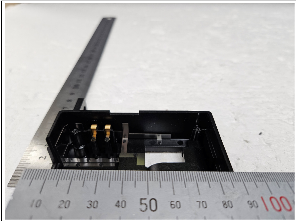
<Internal Antenna 1>
