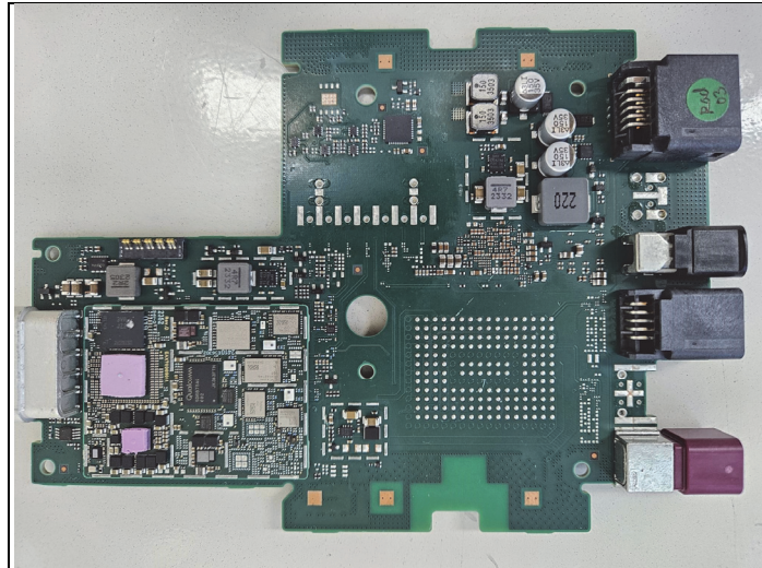
Bottom view of Main PCB (without Shielding)
