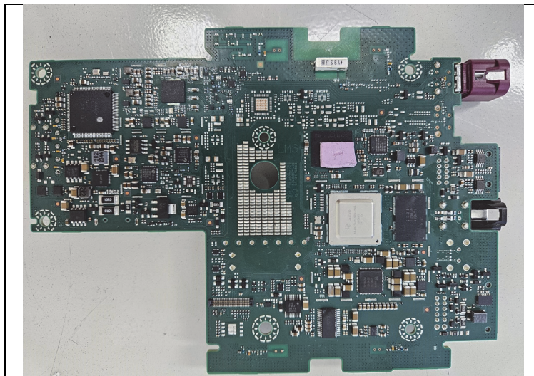
Bottom view of Main PCB (without Shielding)
