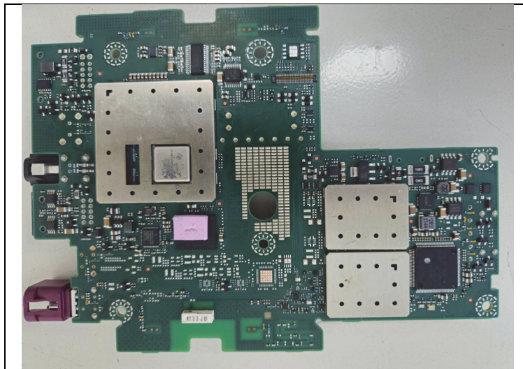
Bottom view of Main PCB
