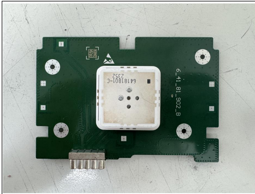
Top view of Sub PCB 1
