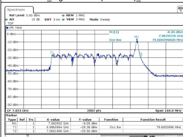
Port 1_High Channel (7 025 MHz)_36 RU
