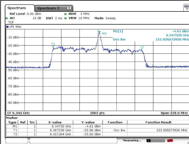
Port 1_High Channel (6 345 MHz)_0 RU
