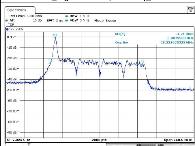
Port 2_High Channel (7 025 MHz)_0 RU
