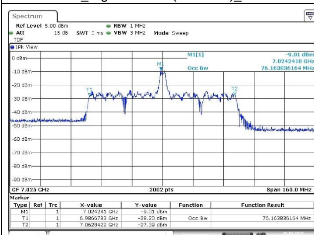
Port 1_High Channel (7 025 MHz)_18 RU
