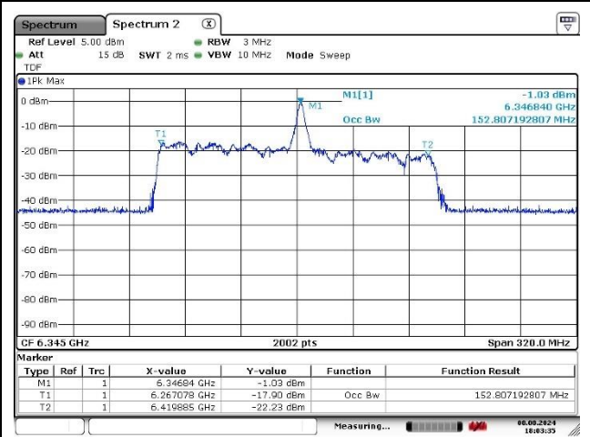
Port 2_High Channel (6 345 MHz)_0 RU
