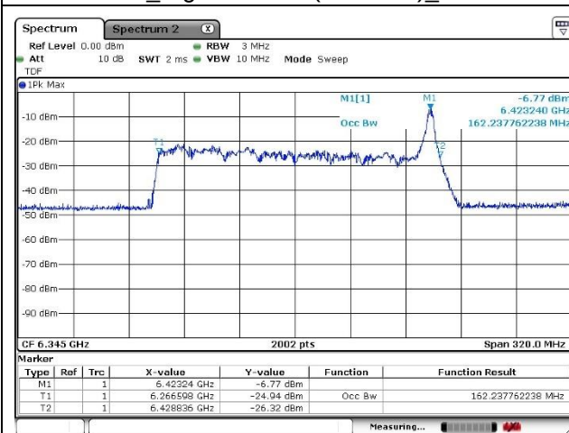
Port 1_High Channel (6 345 MHz)_36 RU
