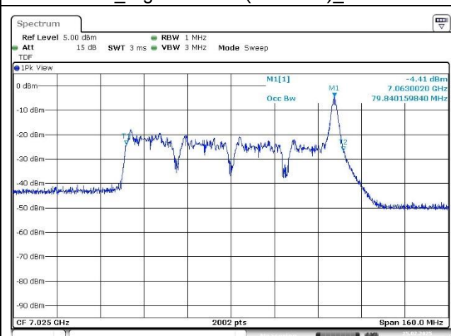
Port 2_High Channel (7 025 MHz)_36 RU
