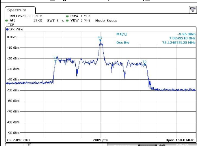
Port 2_High Channel (7 025 MHz)_18 RU
