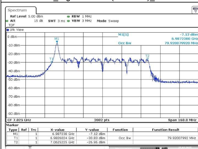
Port 1_High Channel (7 025 MHz)_0 RU
