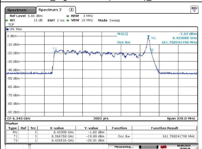
Port 2_High Channel (6 345 MHz)_36 RU
