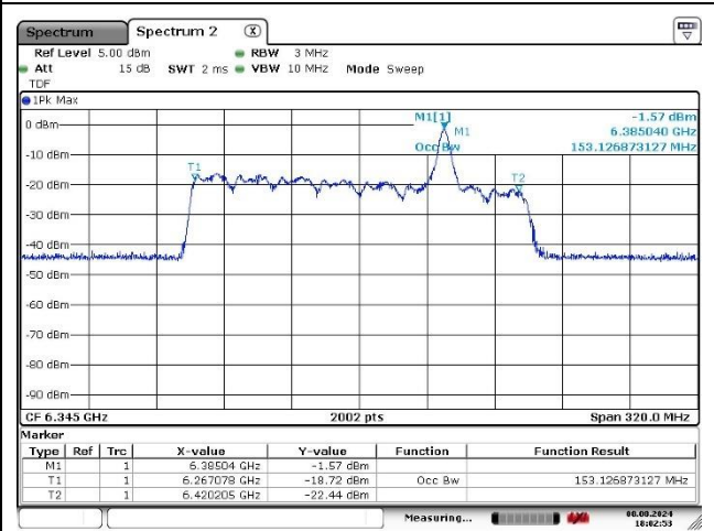
Port 2_High Channel (6 345 MHz)_36 RU
