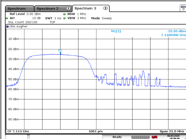
Port 1_High Channel -2 (7 115 MHz)_53 RU
