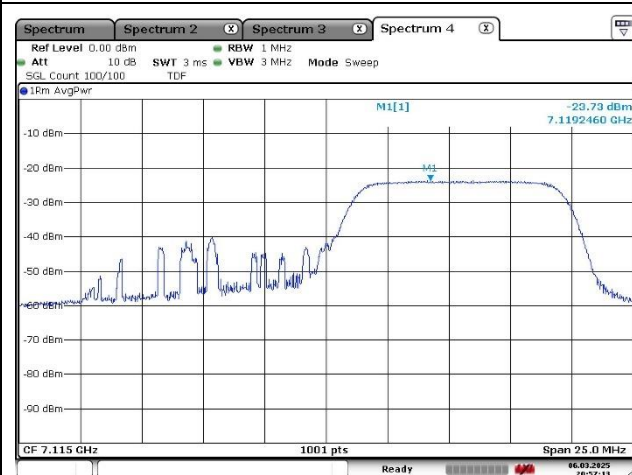
Port 2_High Channel -2 (7 115 MHz)_54 RU
