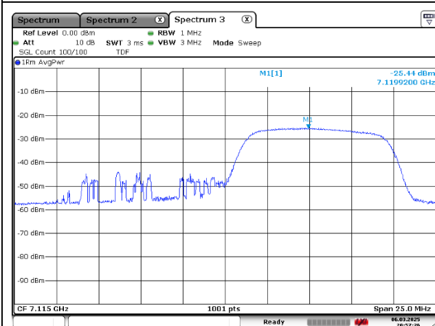
Port 1_High Channel -2 (7 115 MHz)_54 RU
