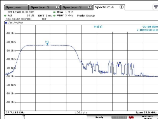
Port 2_High Channel -2 (7 115 MHz)_53 RU
