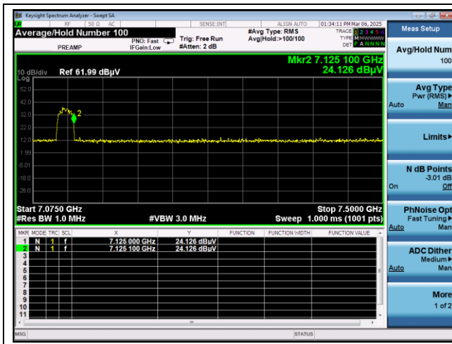
High channel -2 Band edge (Peak) - Band 8
