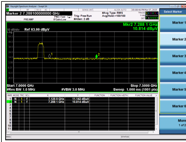
High channel -1 Band edge (Peak) - Band 8
