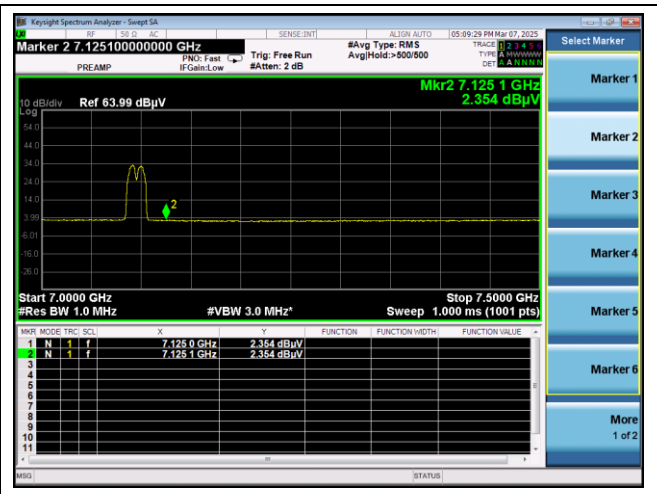
High channel -1 Band edge (Average) - Band 8
