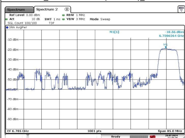
Port 1_Middle Channel (6 705 MHz)_60 RU
