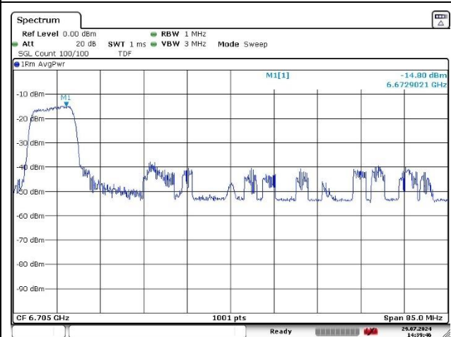
Port 2_Middle Channel (6 705 MHz)_53 RU
