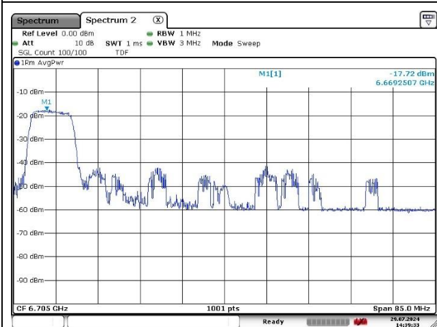
Port 1_Middle Channel (6 705 MHz)_53 RU
