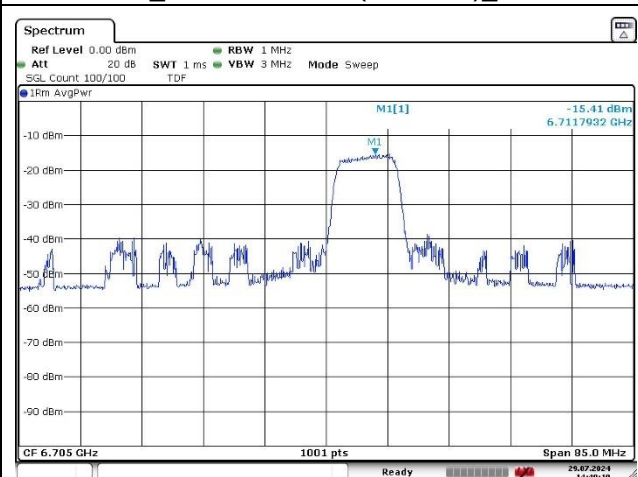
Port 2_Middle Channel (6 705 MHz)_57 RU
