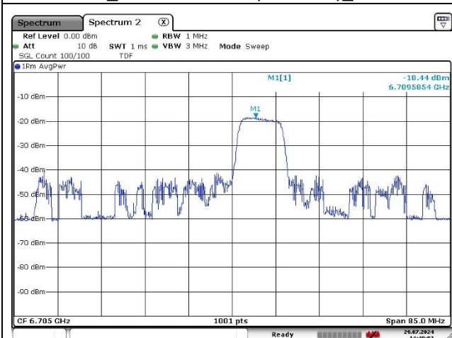
Port 1_Middle Channel (6 705 MHz)_57 RU
