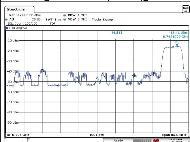
Port 2_Middle Channel (6 705 MHz)_60 RU
