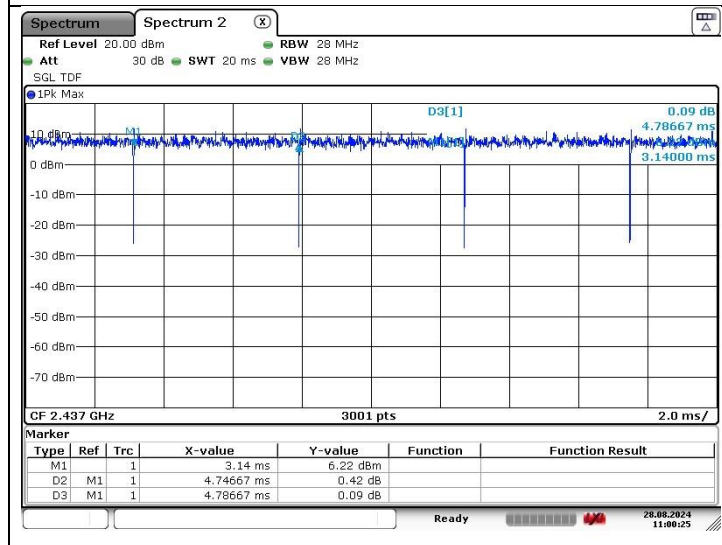
11ax_HE20 106T
