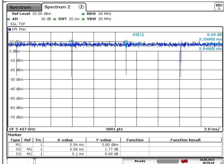
11ax_HE20 52T
