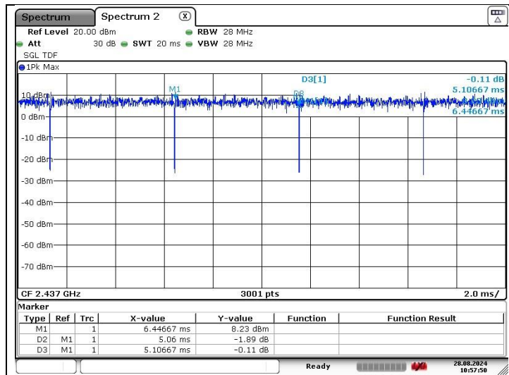
11ax_HE20 26T
