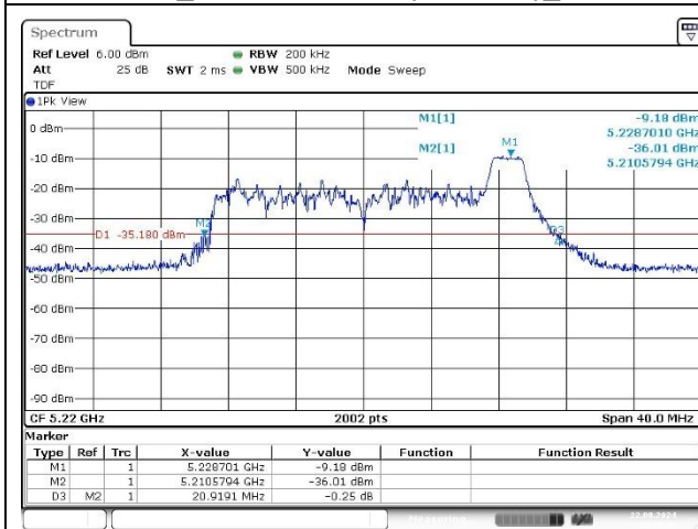
Port 1_Middle Channel (5 220 MHz)_8 RU
