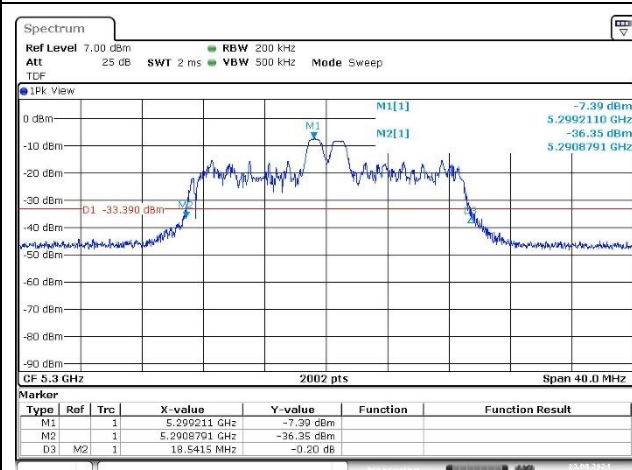
Port 2_Middle Channel (5 300 MHz)_4 RU
