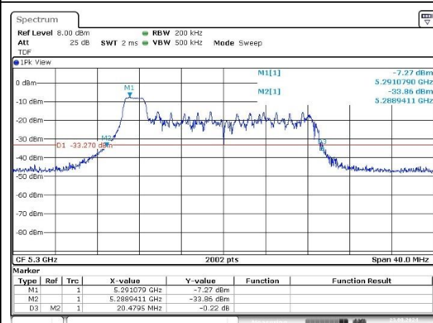
Port 2_Middle Channel (5 300 MHz)_0 RU
