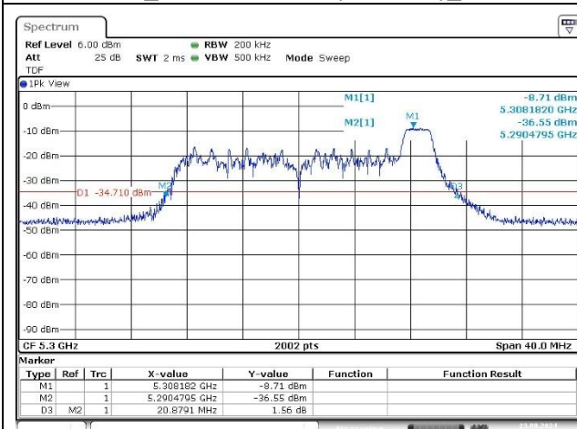
Port 1_Middle Channel (5 300 MHz)_8 RU
