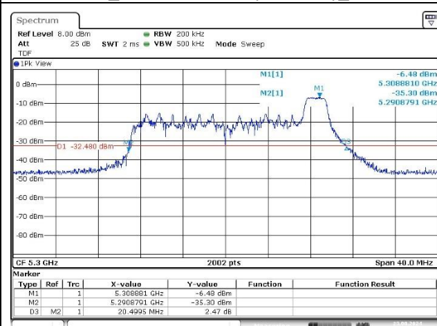
Port 2_Middle Channel (5 300 MHz)_8 RU
