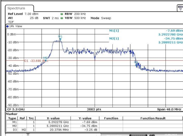
Port 1_Middle Channel (5 300 MHz)_0 RU
