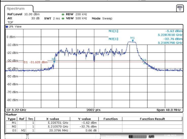
Port 2_Middle Channel (5 220 MHz)_8 RU
