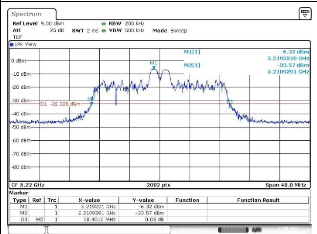
Port 2_Middle Channel (5 220 MHz)_4 RU
