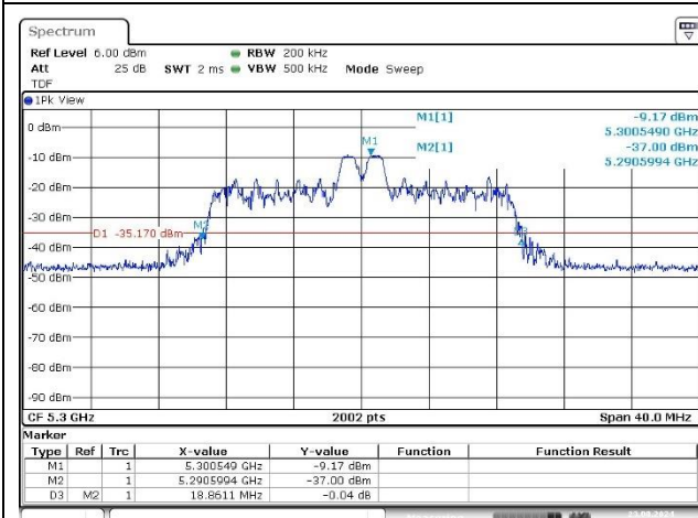
Port 1_Middle Channel (5 300 MHz)_4 RU
