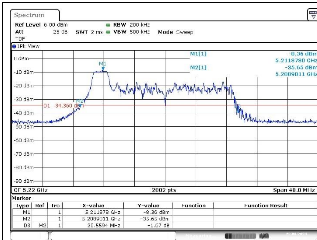
Port 1_Middle Channel (5 220 MHz)_4 RU
