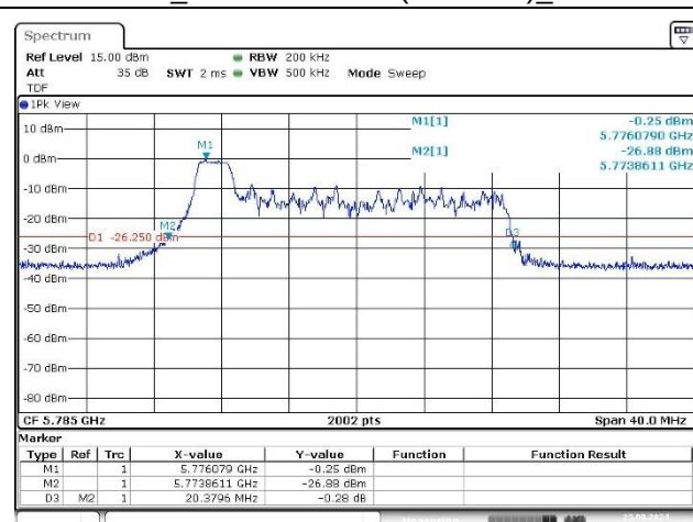
Port 2_Middle Channel (5 785 MHz)_0 RU
