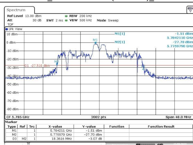
Port 2_Middle Channel (5 785 MHz)_4 RU
