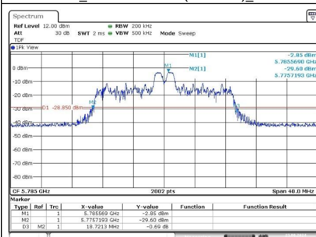
Port 1_Middle Channel (5 785 MHz)_4 RU
