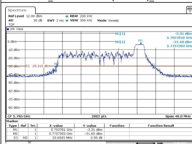
Port 1_Middle Channel (5 785 MHz)_8 RU
