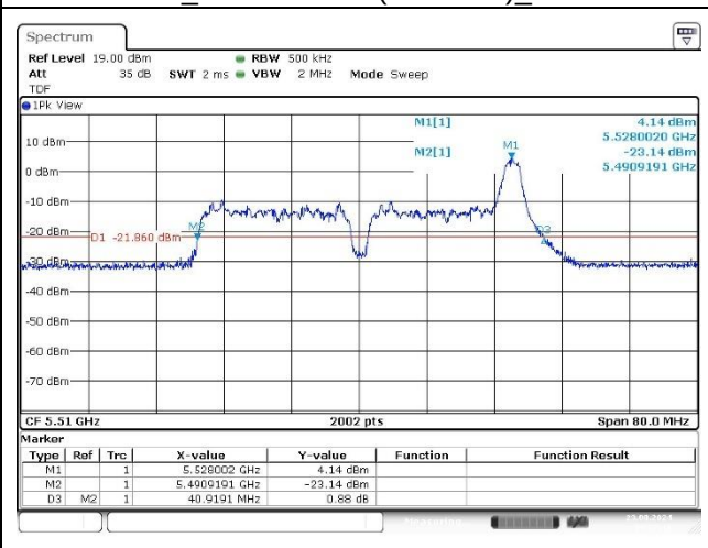
Port 2_Low Channel (5 510 MHz)_17 RU
