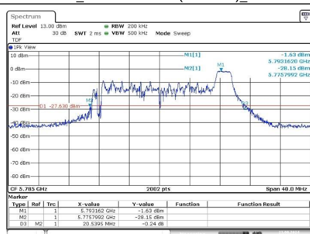
Port 2_Middle Channel (5 785 MHz)_8 RU
