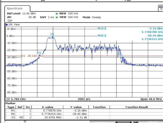
Port 1_Middle Channel (5 785 MHz)_0 RU
