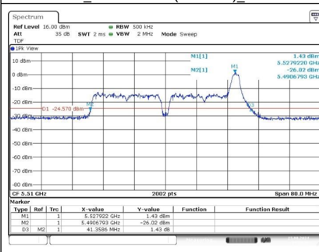
Port 1_Low Channel (5 510 MHz)_17 RU
