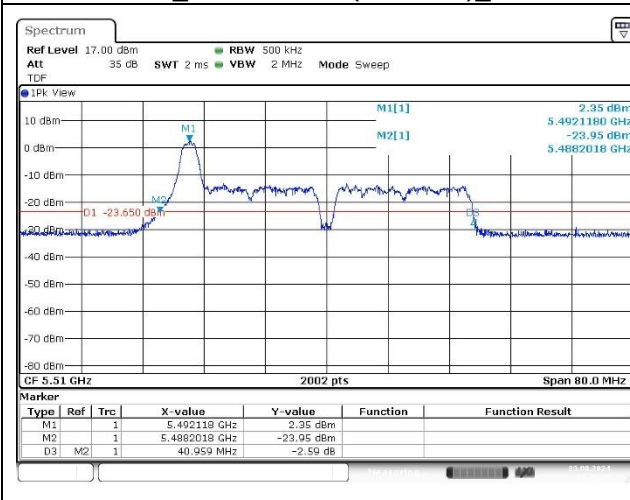
Port 1_Low Channel (5 510 MHz)_9 RU
