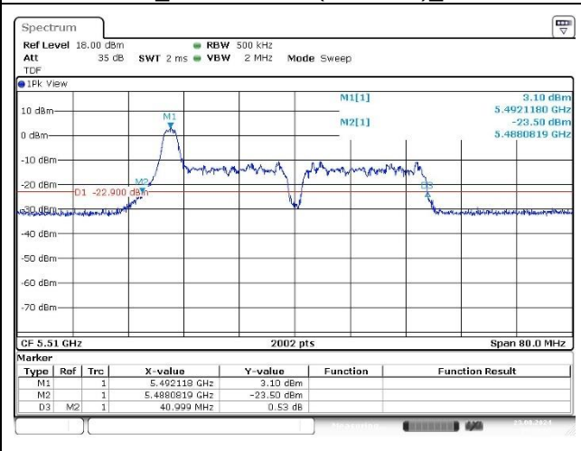
Port 2_Low Channel (5 510 MHz)_9 RU
