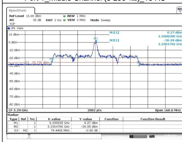
Port 1_Middle Channel (5 290 MHz)_36 RU
