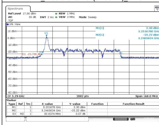
Port 1_Middle Channel (5 290 MHz)_18 RU
