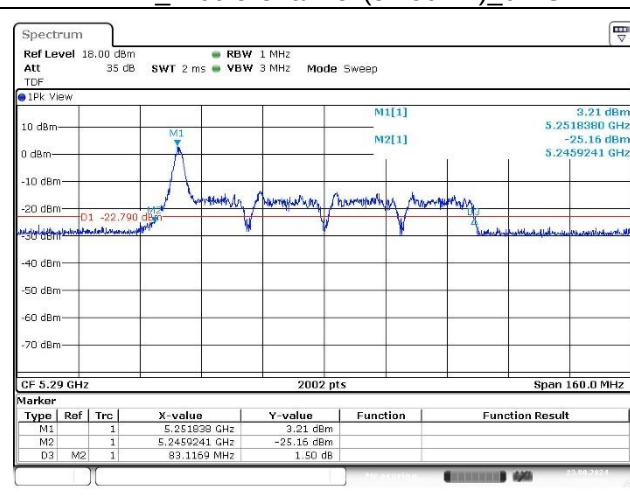
Port 2_Middle Channel (5 290 MHz)_18 RU
