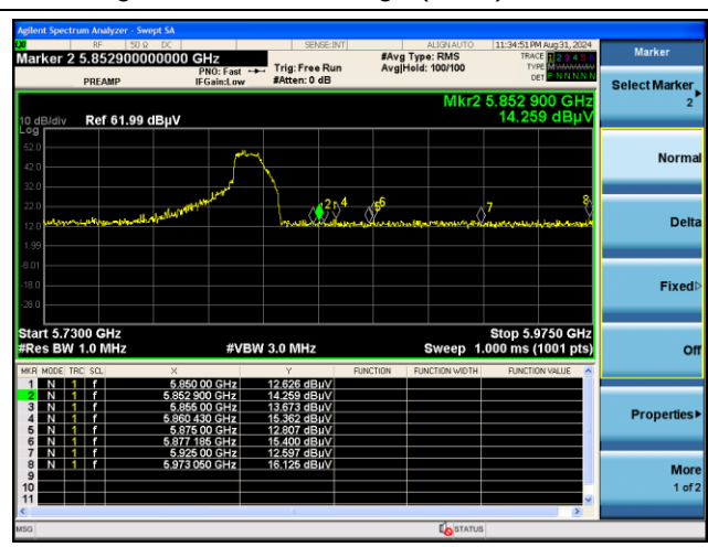
High channel Band edge (Peak) - Band 3
