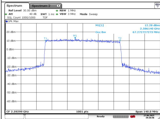
70 MHz_ Middle Channel_CP-OFDM 16QAM_Port 1
