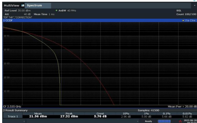
30 MHz Middle Channel - DFT-S-OFDM 16QAM
