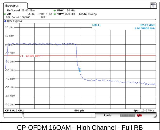
CP-OFDM 16QAM - High Channel - Full RB
