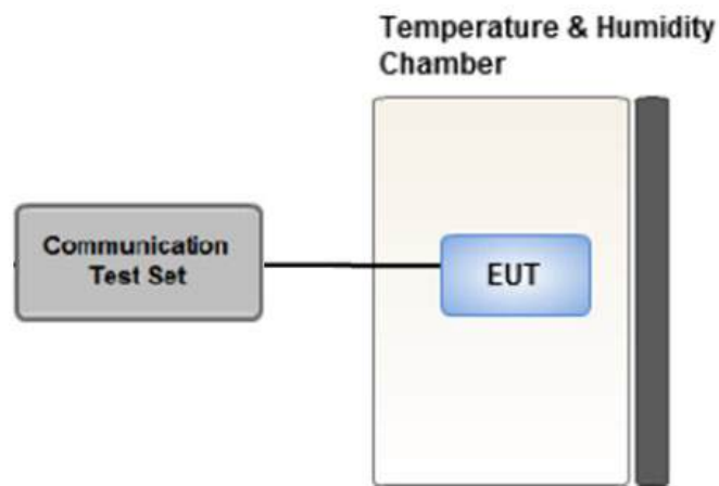
Test setup
