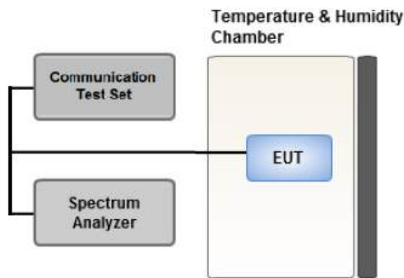
Test setup
