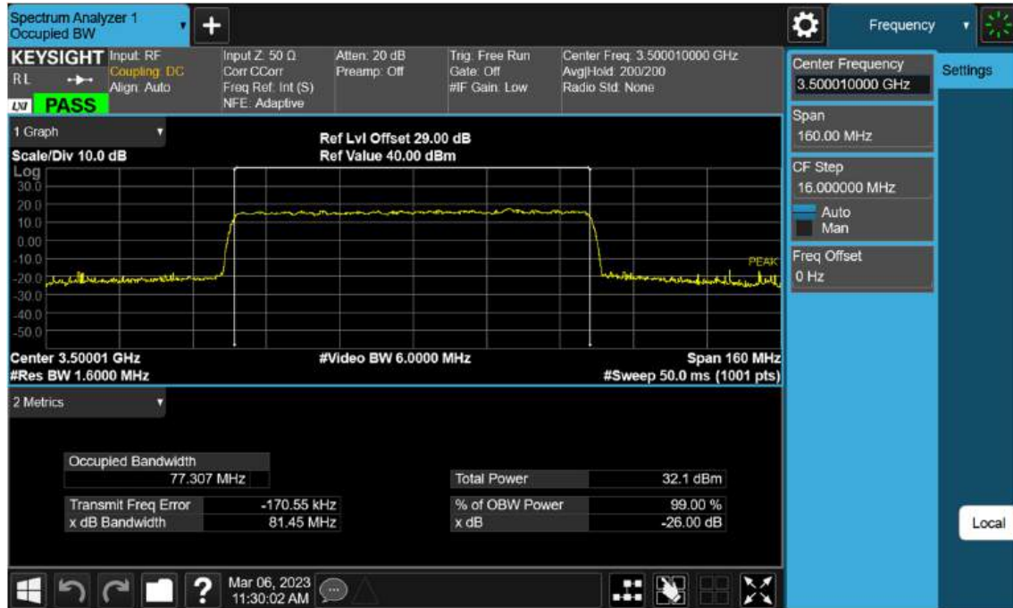
Sub6 n77(78). Occupied Bandwidth Plot (80 M BW Ch.633334 64 QAM )
