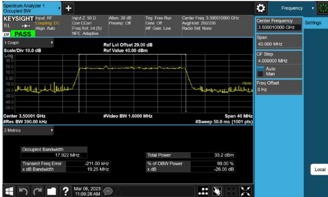
Sub6 n77(78). Occupied Bandwidth Plot (20 M BW Ch.633334 BPSK )
