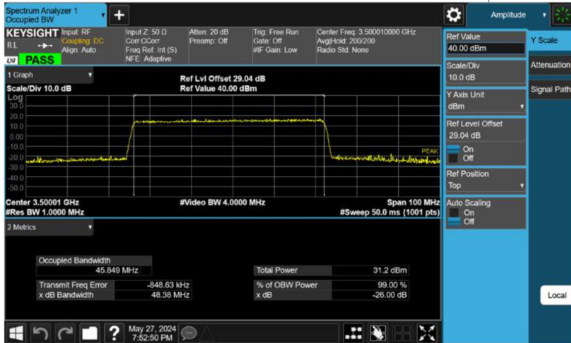
Sub6 n77(78). Occupied Bandwidth Plot (50 M BW Ch.633334 256 QAM)
