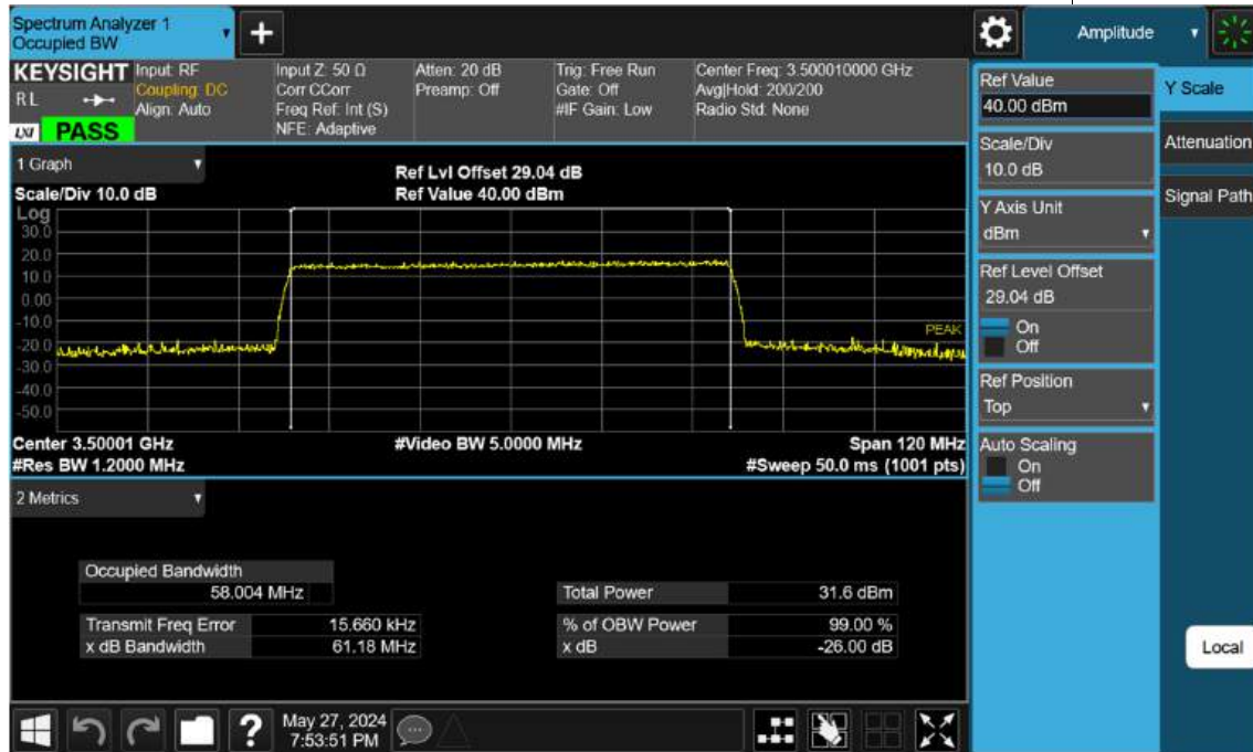
Sub6 n77(78). Occupied Bandwidth Plot (60 M BW Ch.633334 256 QAM)
