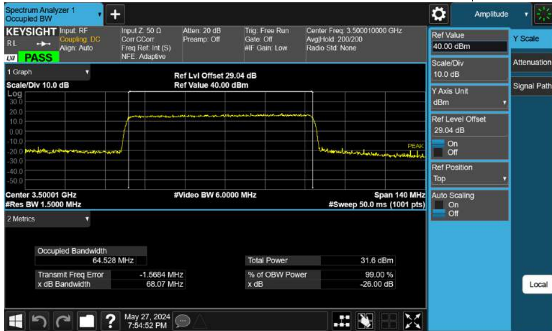
Sub6 n77(78). Occupied Bandwidth Plot (70 M BW Ch.633334 256 QAM )
