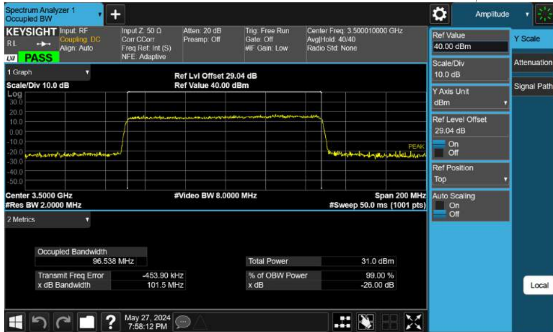
Sub6 n77(78). Occupied Bandwidth Plot (100 M BW Ch.633334 256 QAM)
