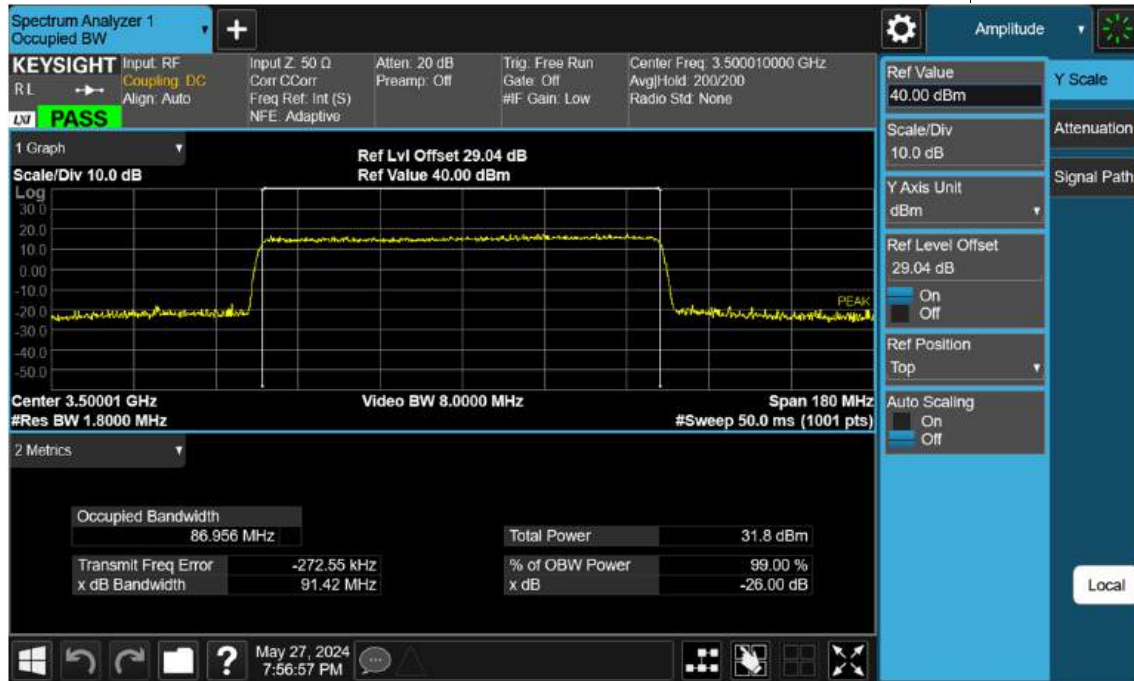
Sub6 n77(78). Occupied Bandwidth Plot (90 M BW Ch.633334 256 QAM )
