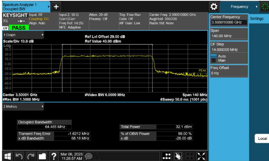
Sub6 n77(78). Occupied Bandwidth Plot (70 M BW Ch.633334 64 QAM )
