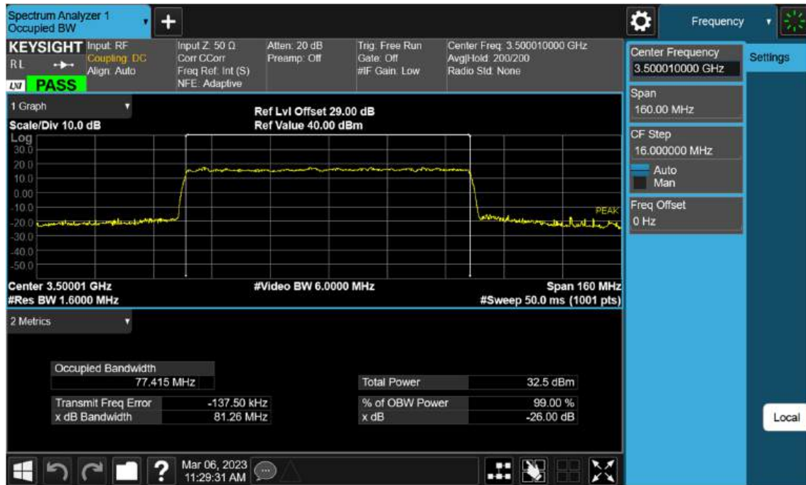
Sub6 n77(78). Occupied Bandwidth Plot (80 M BW Ch.633334 16QAM )
