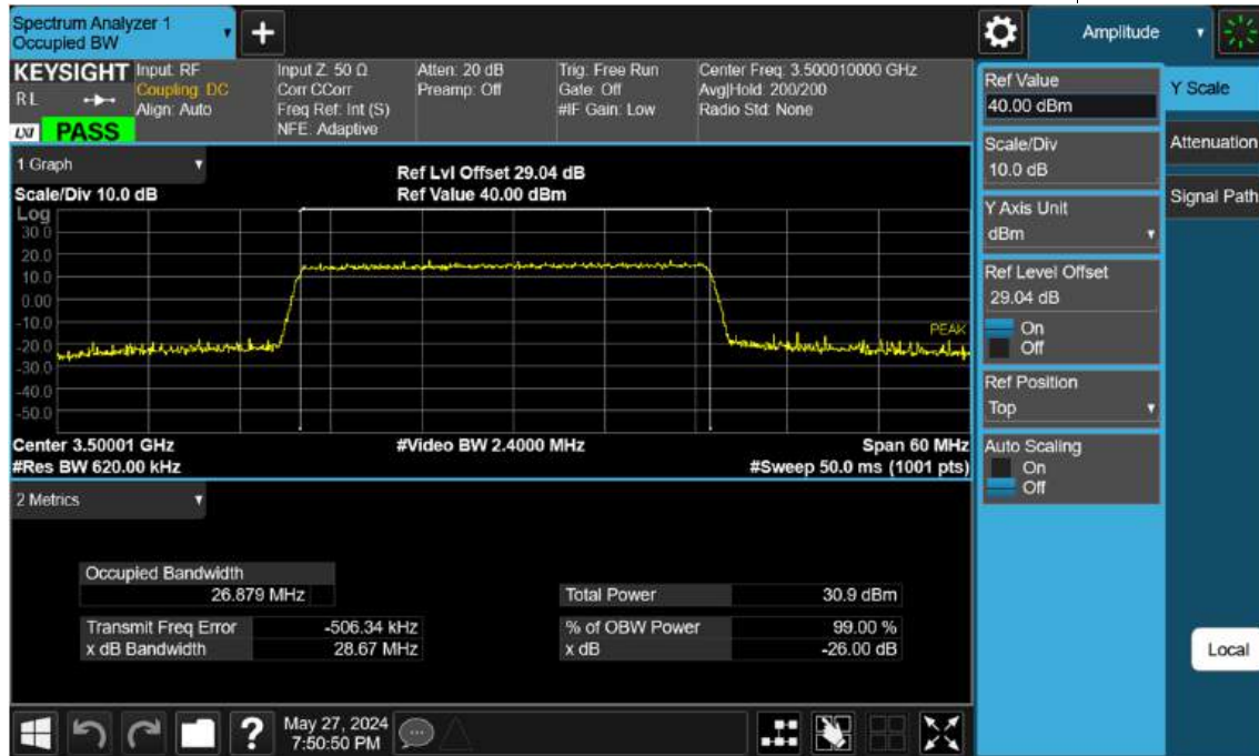
Sub6 n77(78). Occupied Bandwidth Plot (30 M BW Ch.633334 256 QAM )
