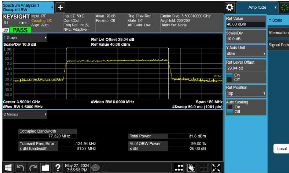
Sub6 n77(78). Occupied Bandwidth Plot (80 M BW Ch.633334 256 QAM )
