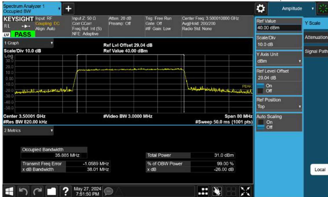
Sub6 n77(78). Occupied Bandwidth Plot (40 M BW Ch.633334 256 QAM)
