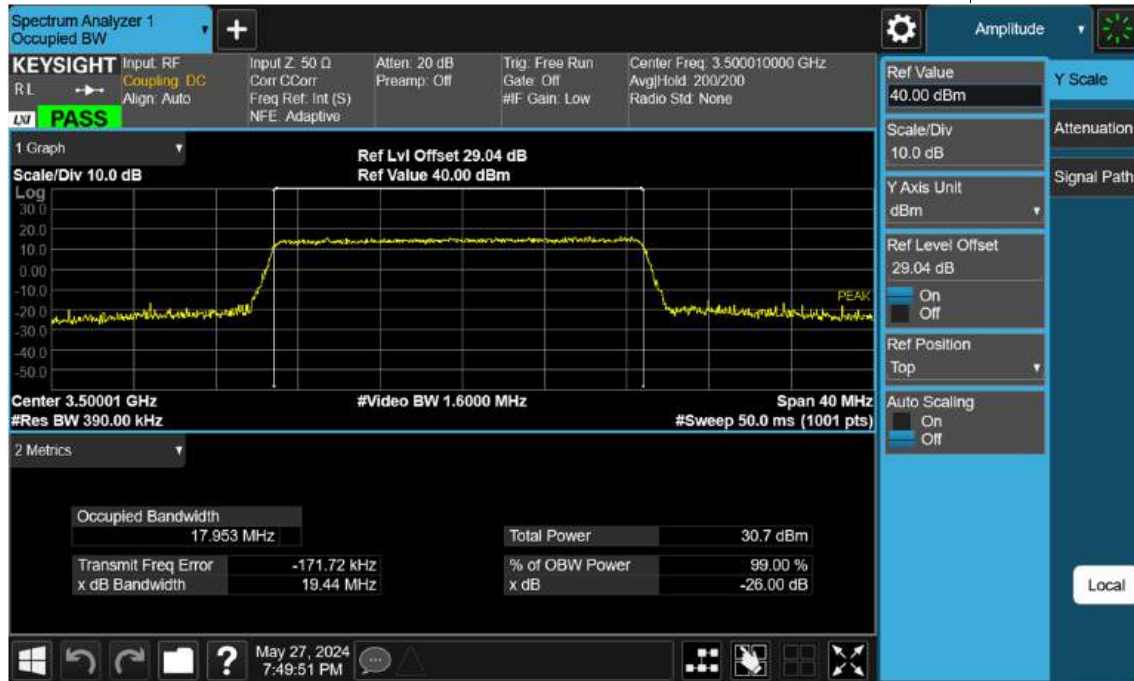
Sub6 n77(78). Occupied Bandwidth Plot (20 M BW Ch.633334 256 QAM )
