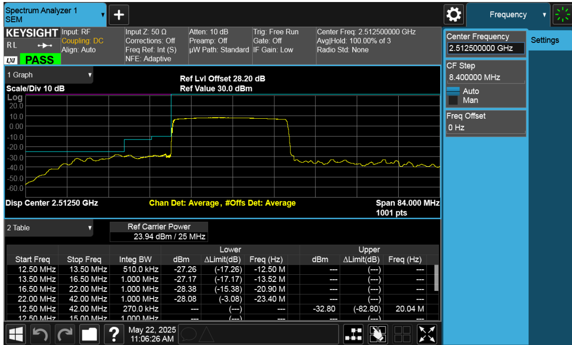
Low Channel Edge Plot (25 MHz BPSK)-1
