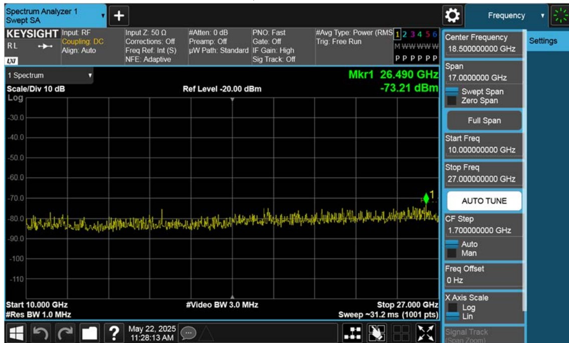
NR7_30 M_Conducted Spurious(Above10 G)_Low_BPSK_1RB
