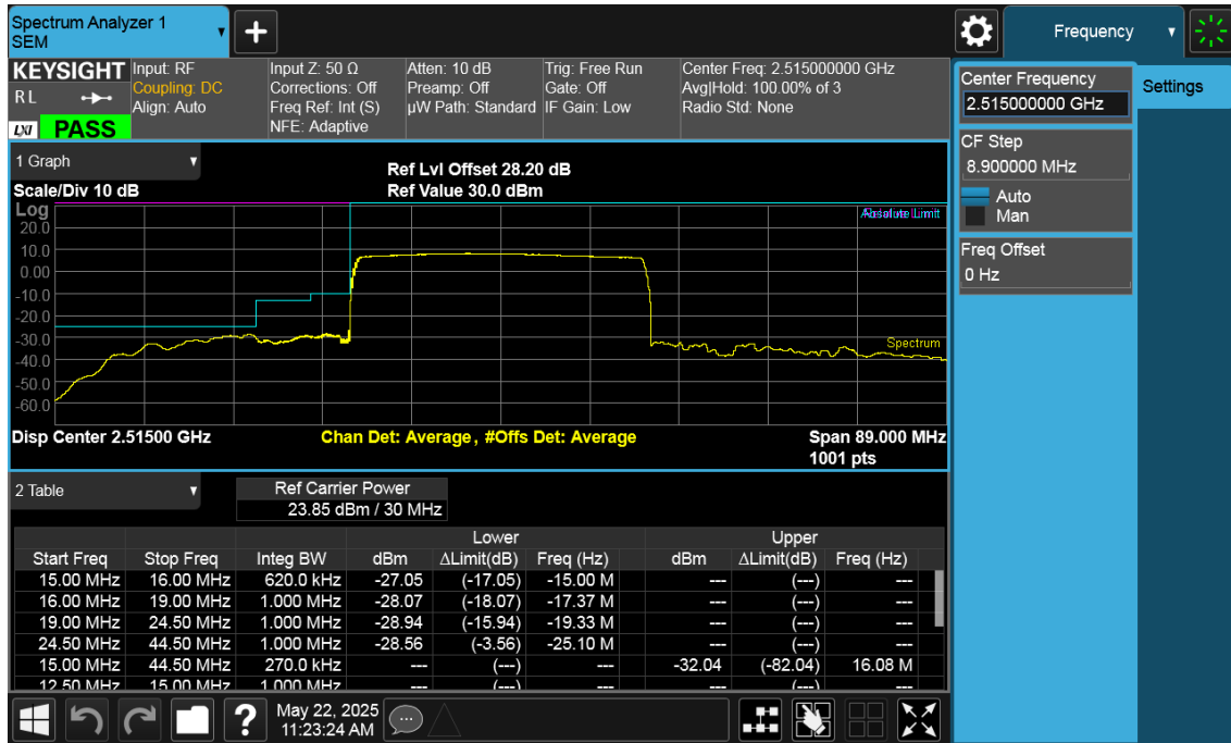
Low Channel Edge Plot (30 MHz BPSK)-1
