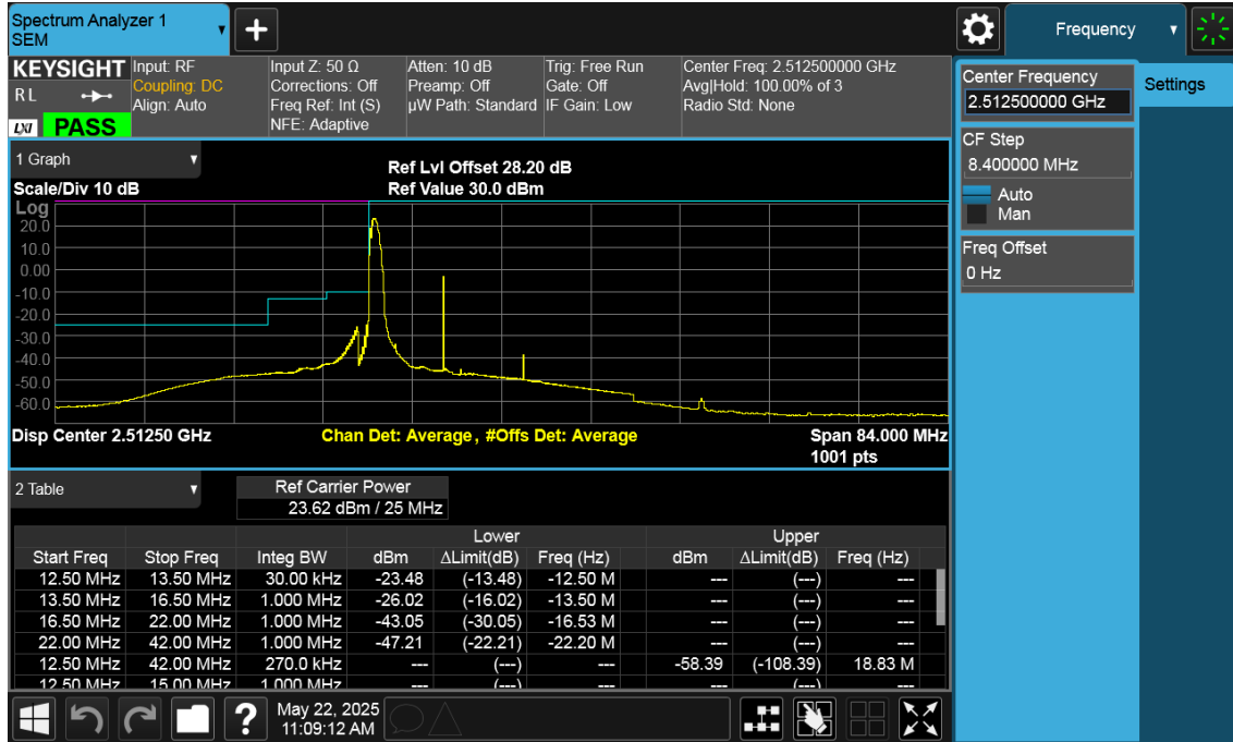
Low Channel Edge Plot (25 MHz BPSK RB 1)-1
