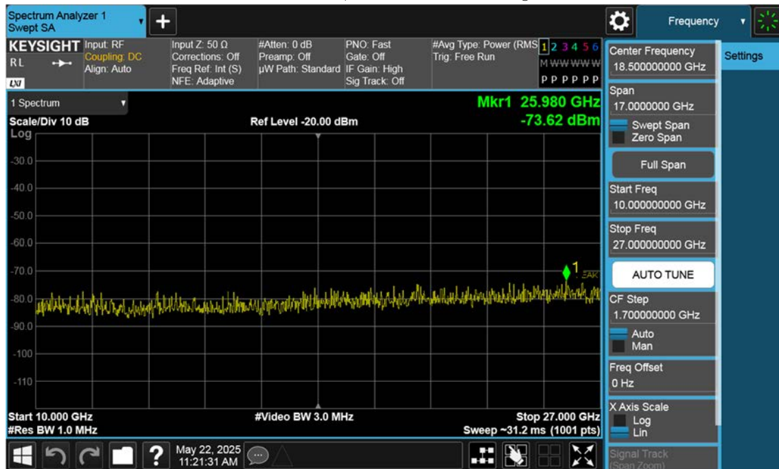
NR7_25 M_Conducted Spurious(Above10 G)_High_BPSK_1RB
