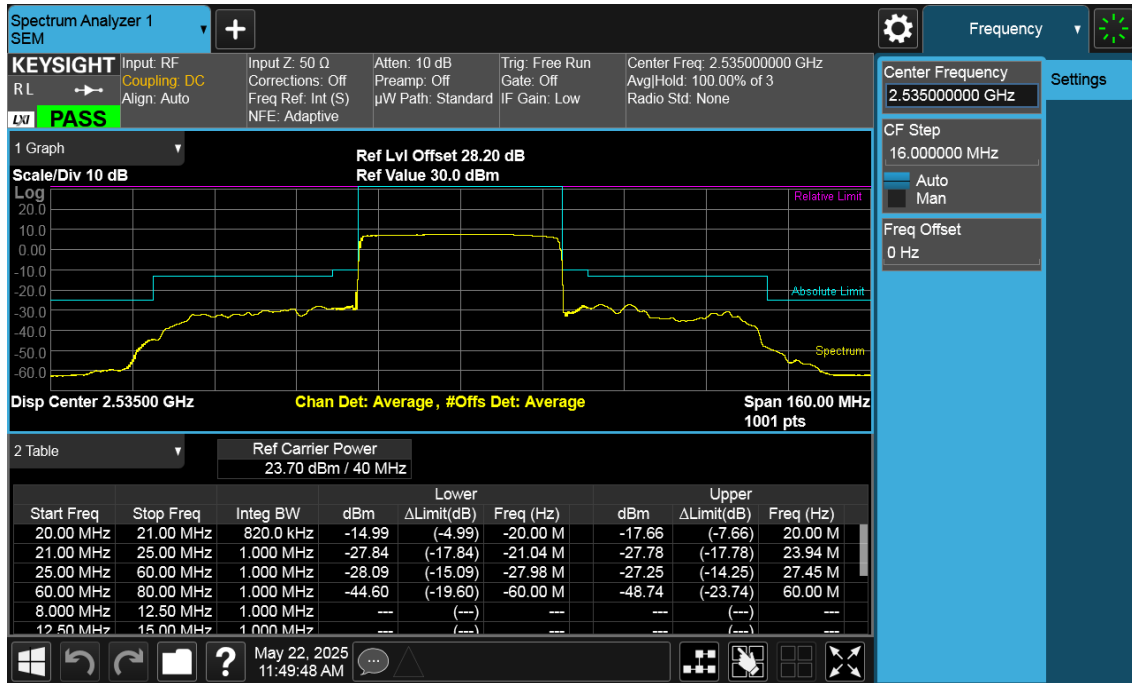
Mid Channel Edge Plot (40 MHz BPSK)
