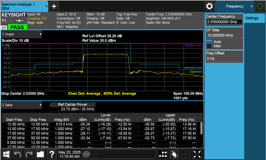
Mid Channel Edge Plot (25 MHz BPSK)
