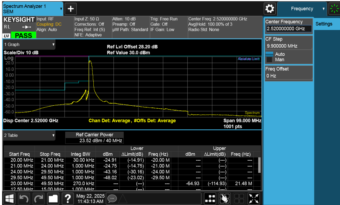
Low Channel Edge Plot (40 MHz BPSK RB 1)-1
