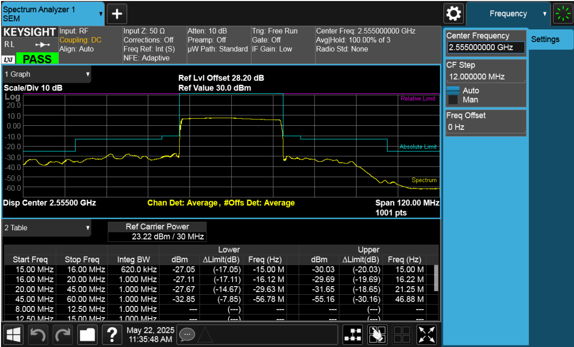
High Channel Edge Plot (30 MHz BPSK)
