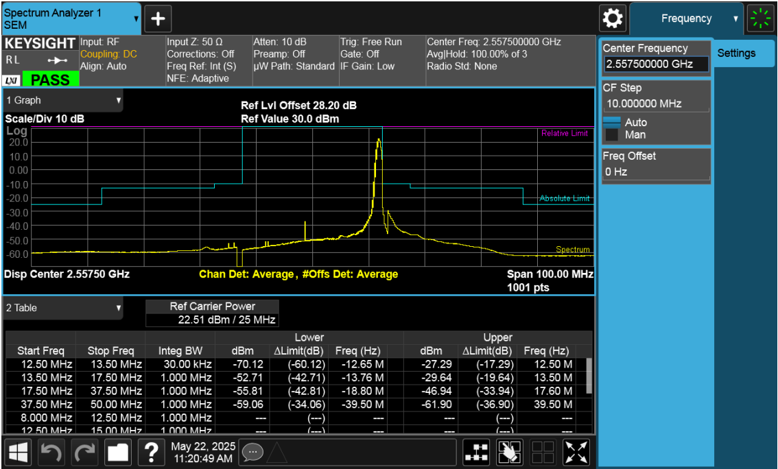
High Channel Edge Plot (25 MHz BPSK RB 1)
