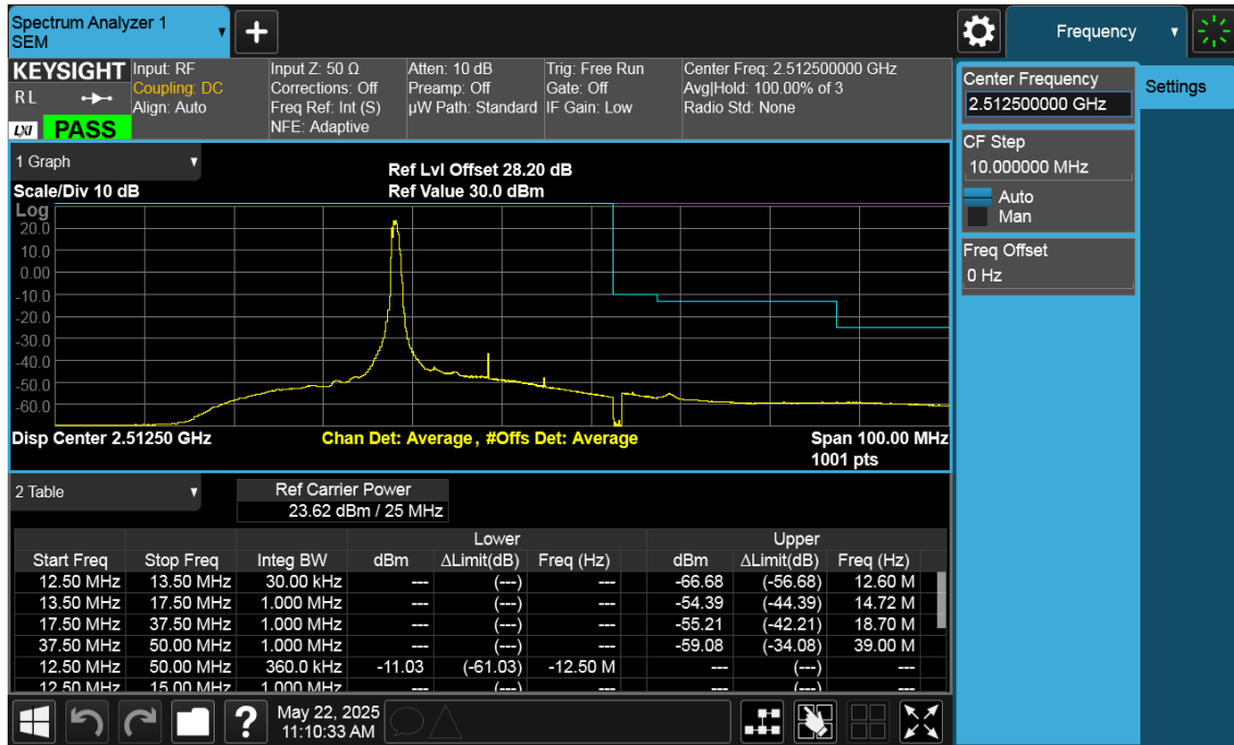
Low Channel Edge Plot (25 MHz BPSK_RB1)-2
