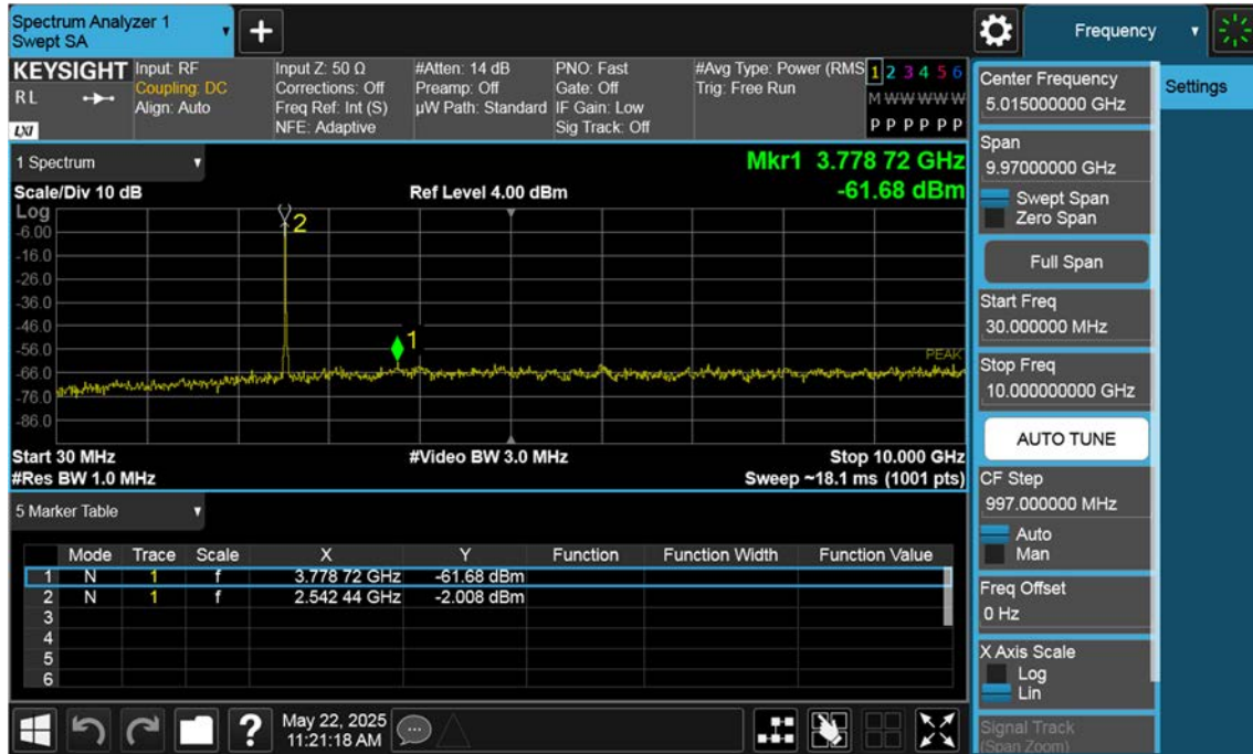
NR7_25 M_Conducted Spurious(30 M-10 G)_High_BPSK_1RB
