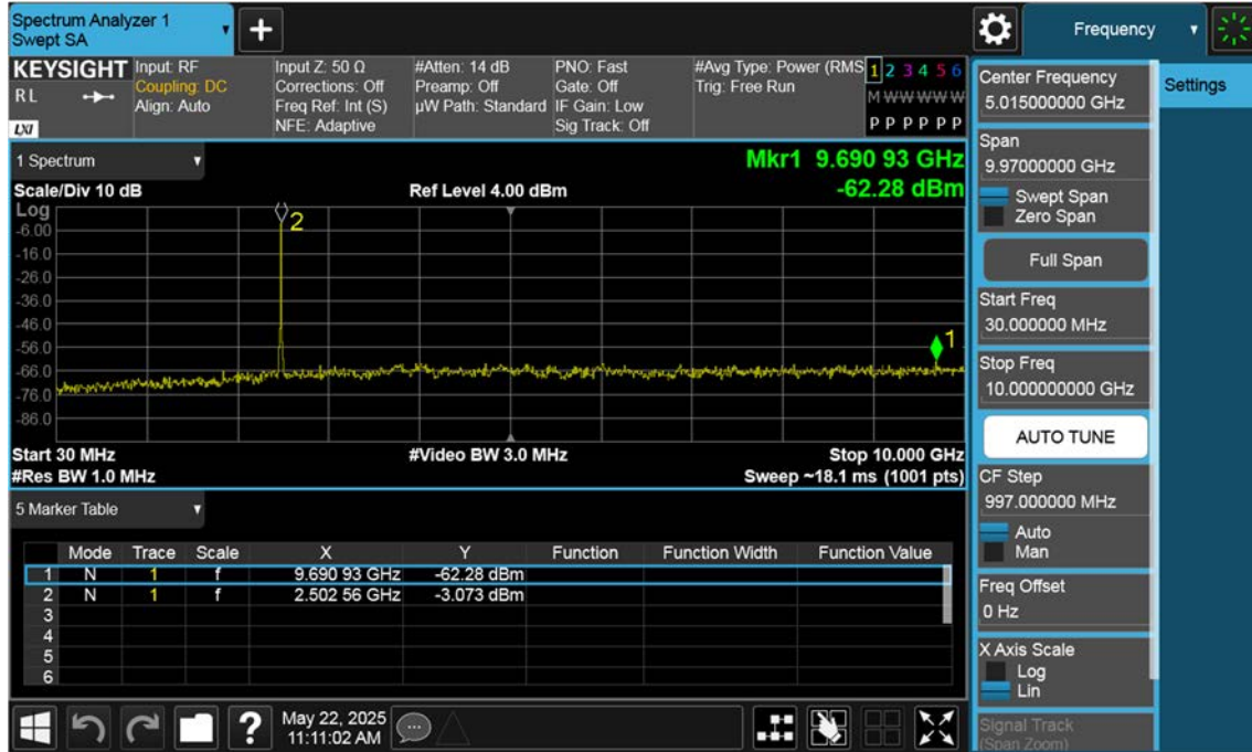
NR7_25 M_Conducted Spurious(30 M-10 G)_Low_BPSK_1RB
