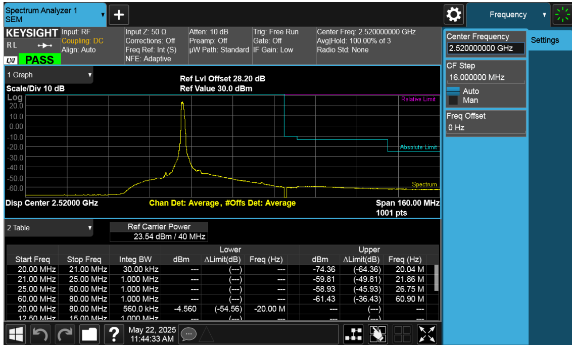
Low Channel Edge Plot (40 MHz BPSK_RB1)-2
