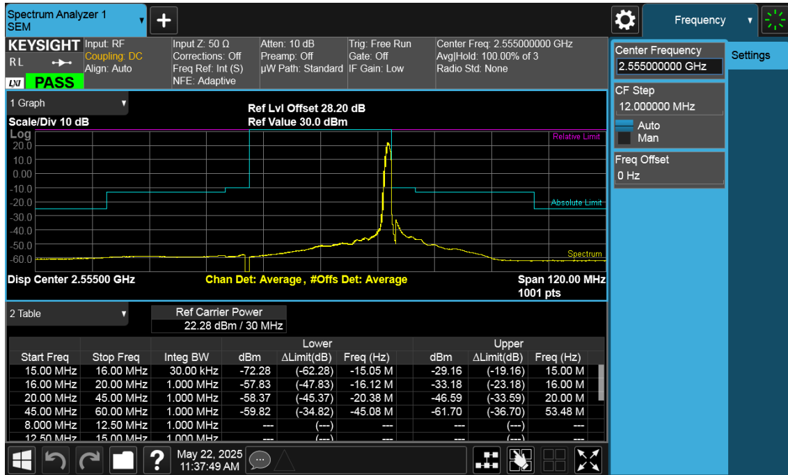
High Channel Edge Plot (30 MHz BPSK RB 1)
