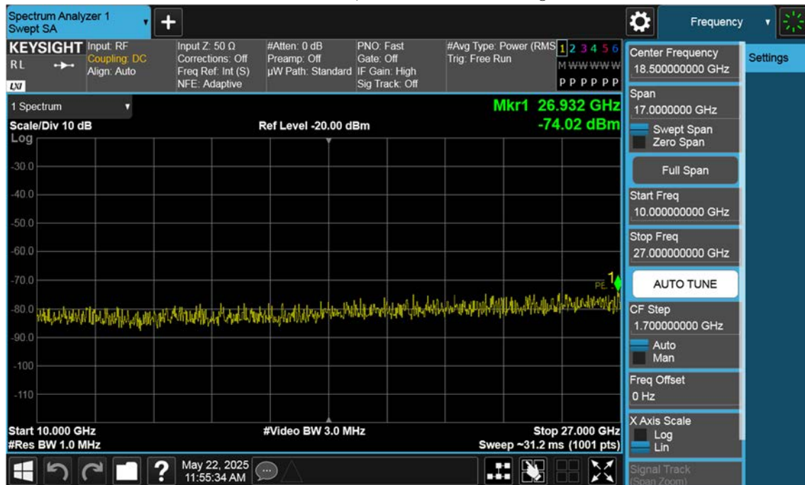
NR7_40 M_Conducted Spurious(Above10 G)_High_BPSK_1RB
