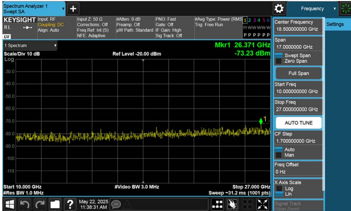
NR7_30 M_Conducted Spurious(Above10 G)_High_BPSK_1RB
