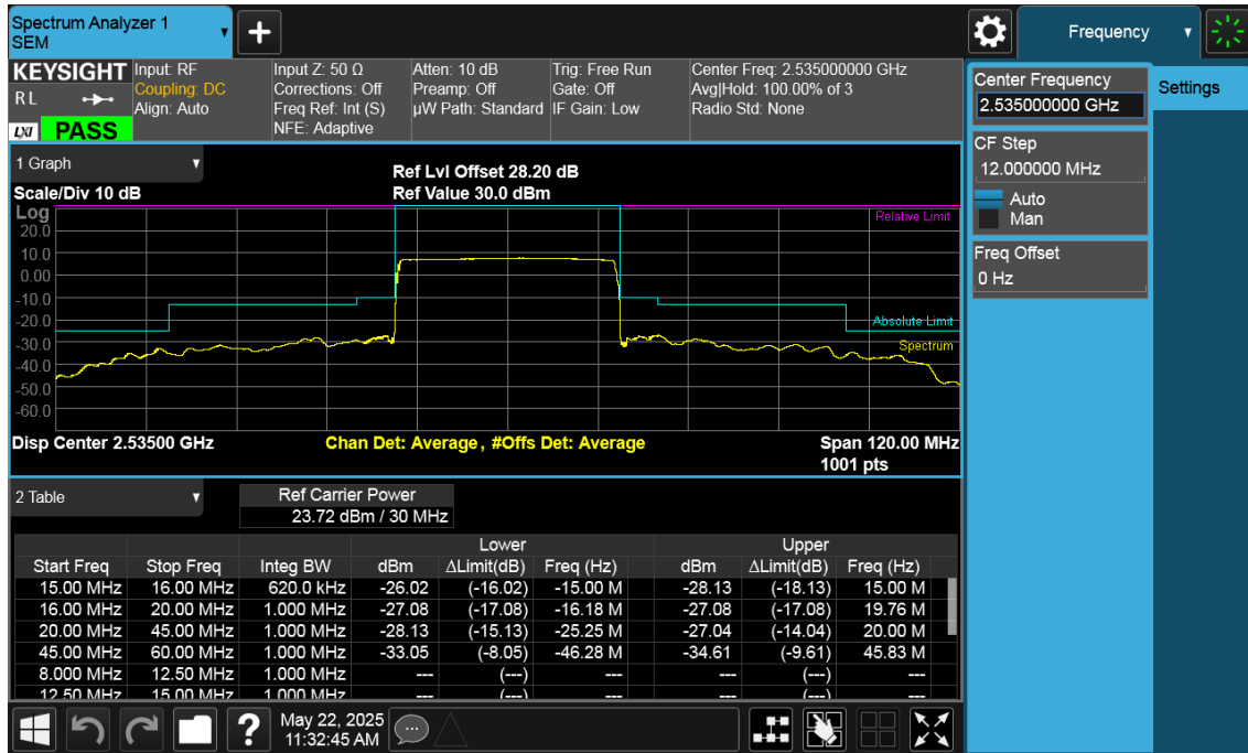
Mid Channel Edge Plot (30 MHz BPSK)
