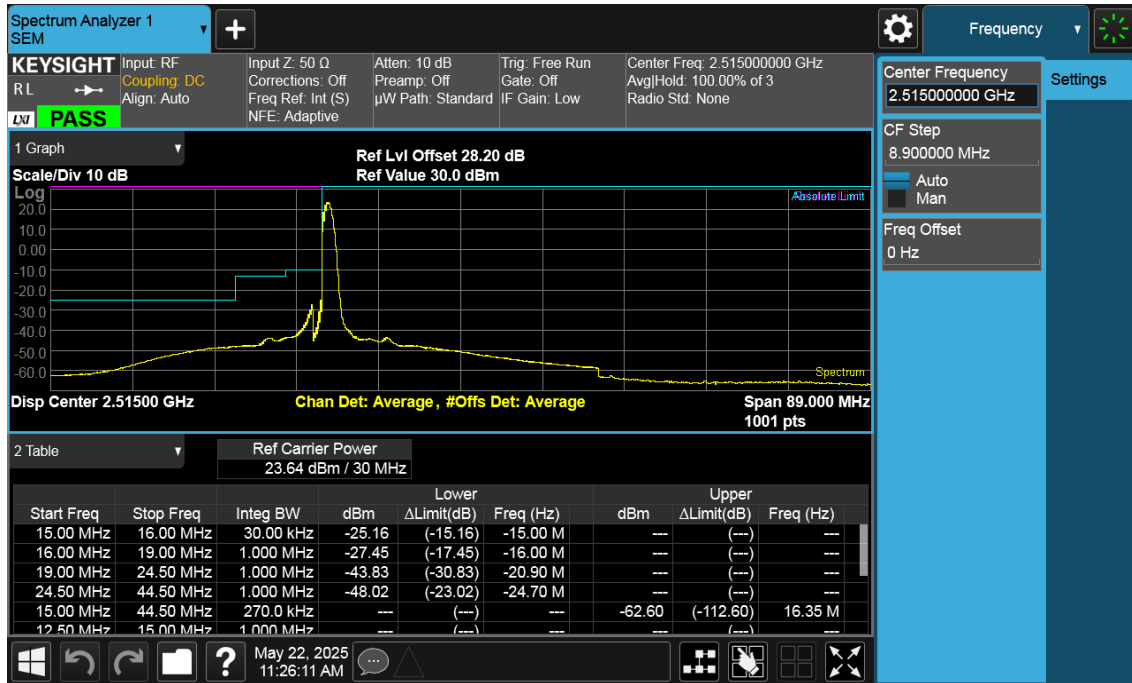
Low Channel Edge Plot (30 MHz BPSK RB 1)-1
