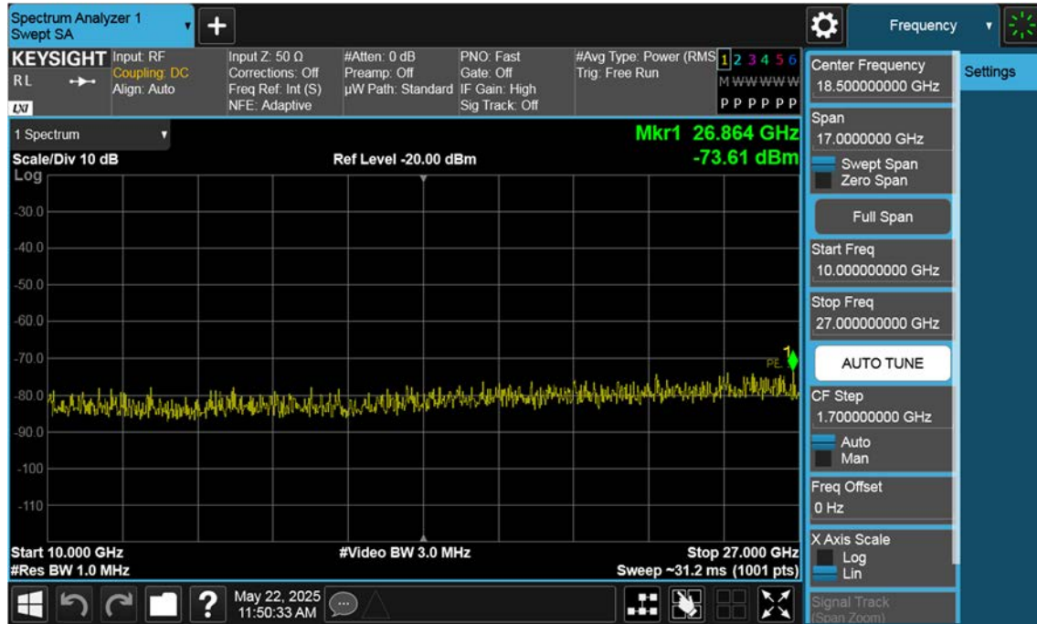
NR7_40 M_Conducted Spurious(Above10 G)_Mid_BPSK_1RB
