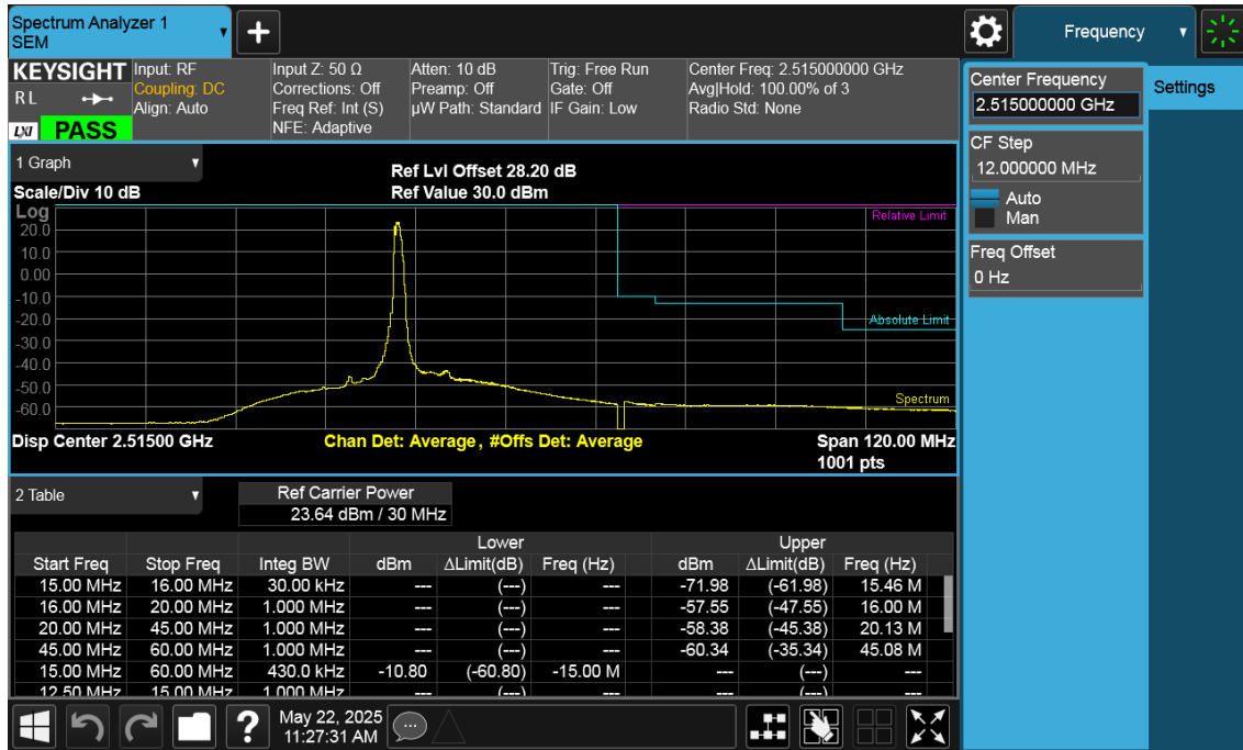
Low Channel Edge Plot (30 MHz BPSK_RB1)-2
