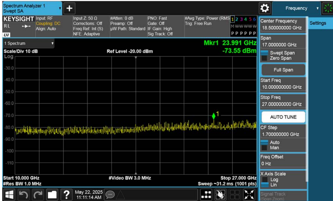
NR7_25 M_Conducted Spurious(Above10 G)_Low_BPSK_1RB
