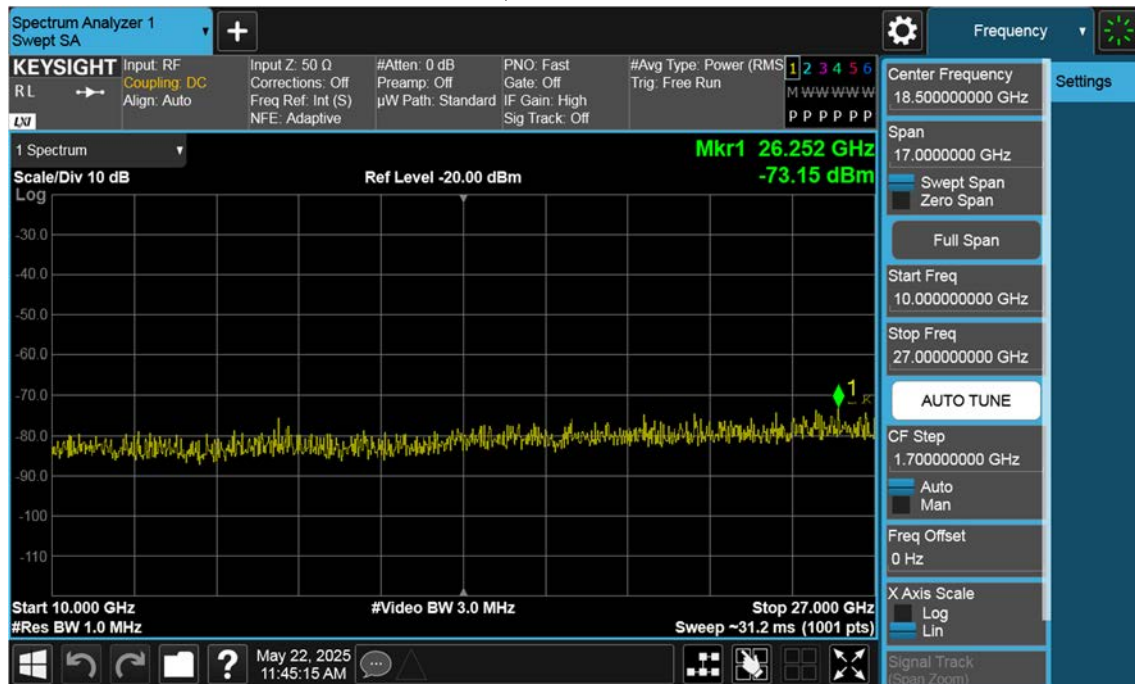
NR7_40 M_Conducted Spurious(Above10 G)_Low_BPSK_1RB
