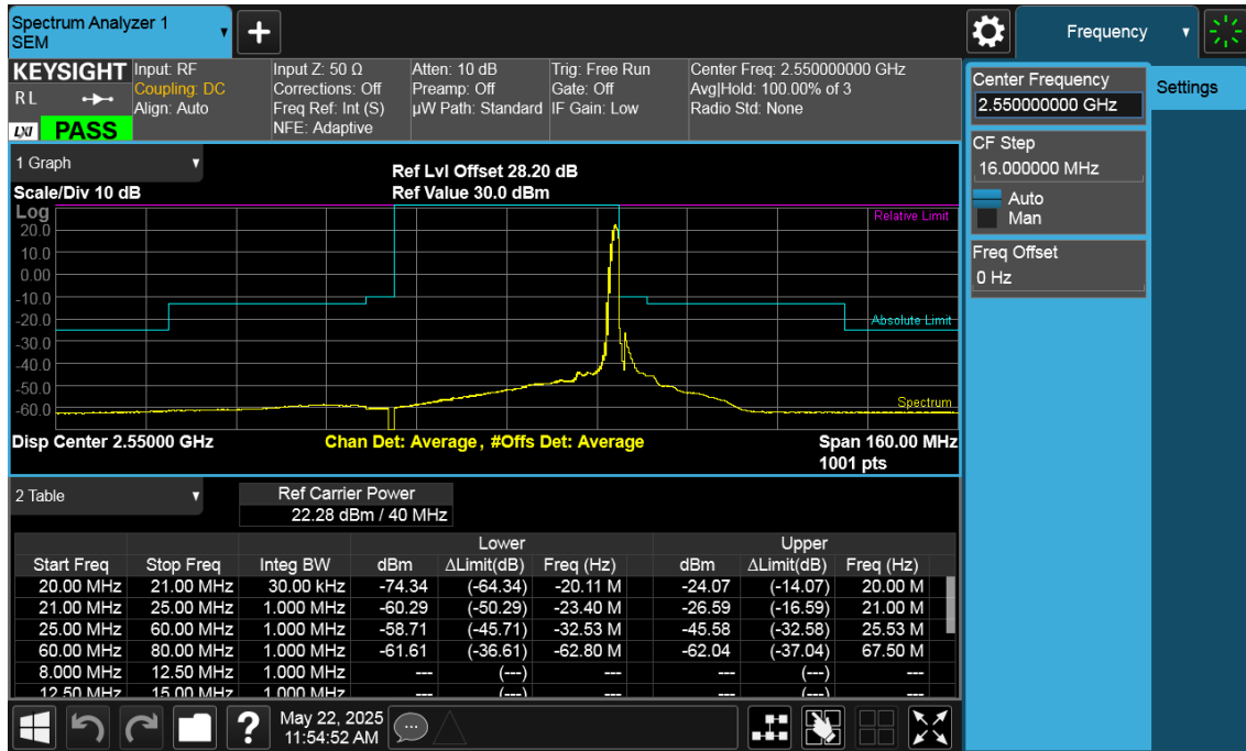
High Channel Edge Plot (40 MHz BPSK RB 1)
