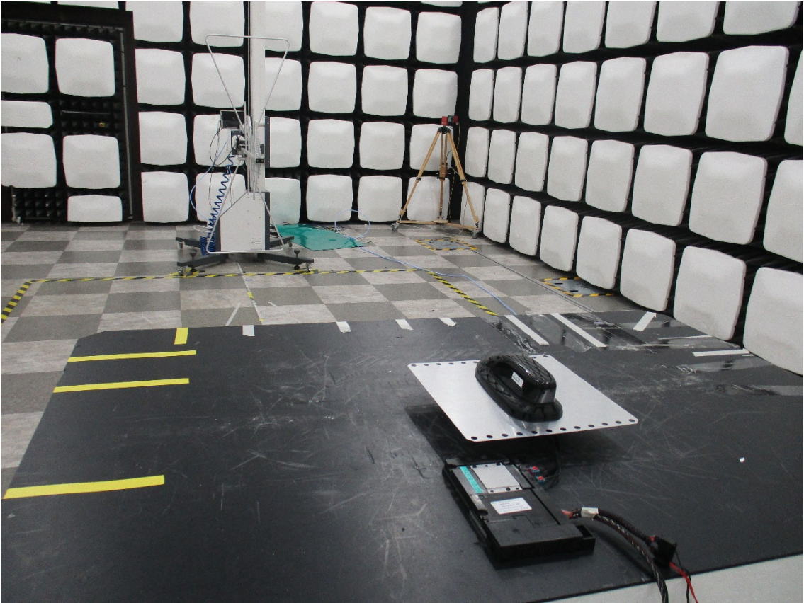
3-2. Radiated Test Setup Photo(BT1UG)-Bilog Antenna, Antenna Mast: Vertical
