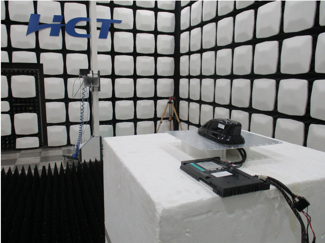
4-2. Radiated Test Setup Photo(BT1UG)-Horn Antenna, Antenna Mast: Vertical
