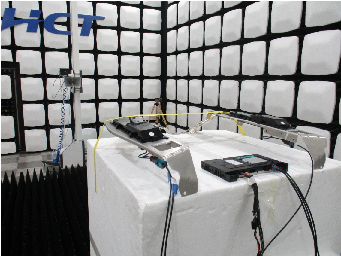
2-2. Radiated Test Setup Photo(Y2XX)-Horn Antenna, Antenna Mast: Vertical
