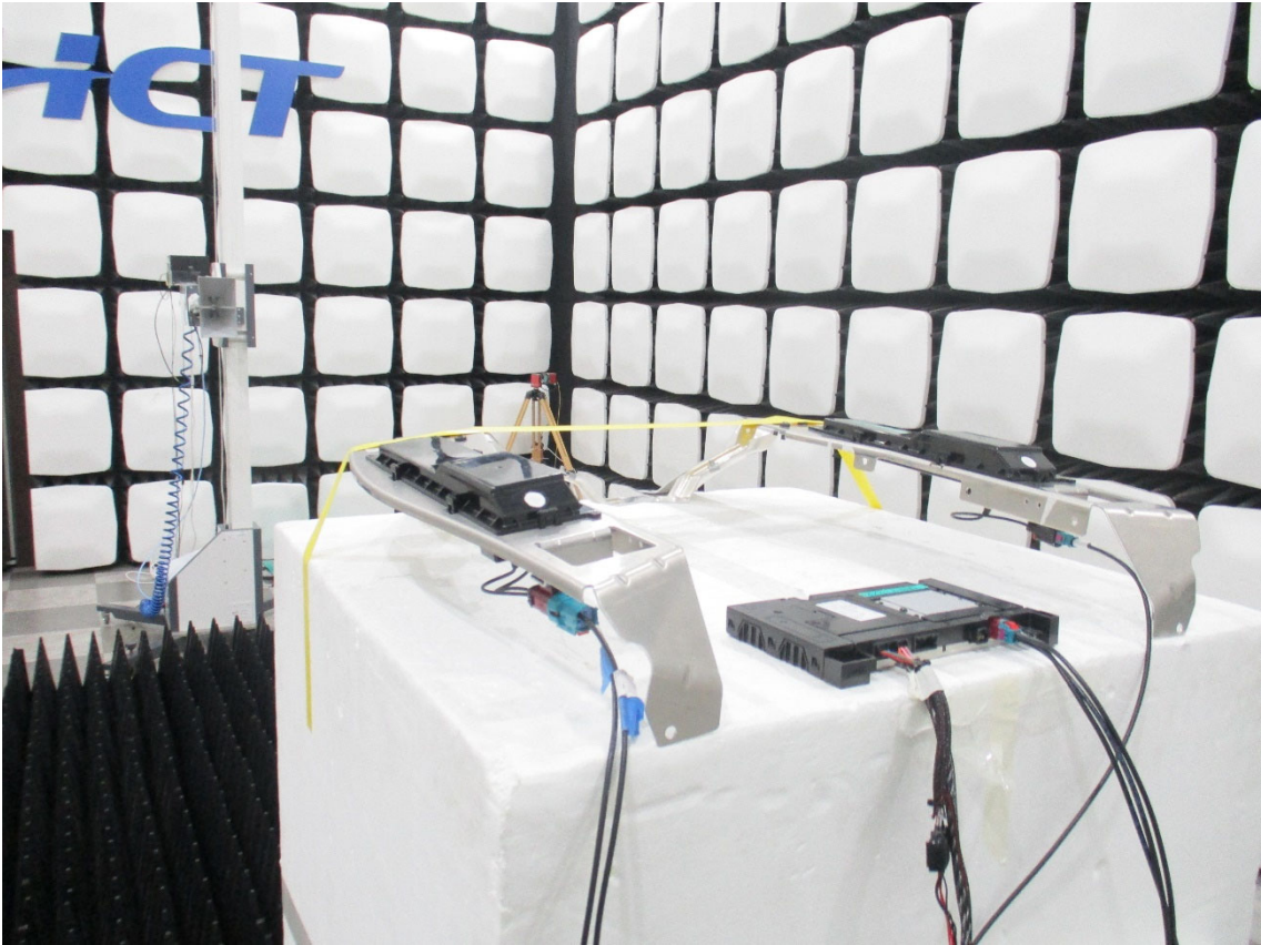
2-1. Radiated Test Setup Photo(Y2XX)-Horn Antenna, Antenna Mast: Horizontal
