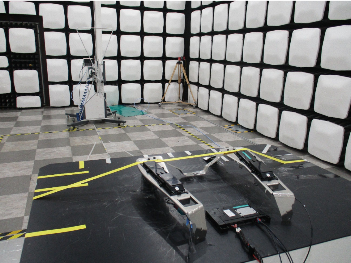
1-2. Radiated Test Setup Photo(Y2XX)-Bilog Antenna, Antenna Mast: Vertical
