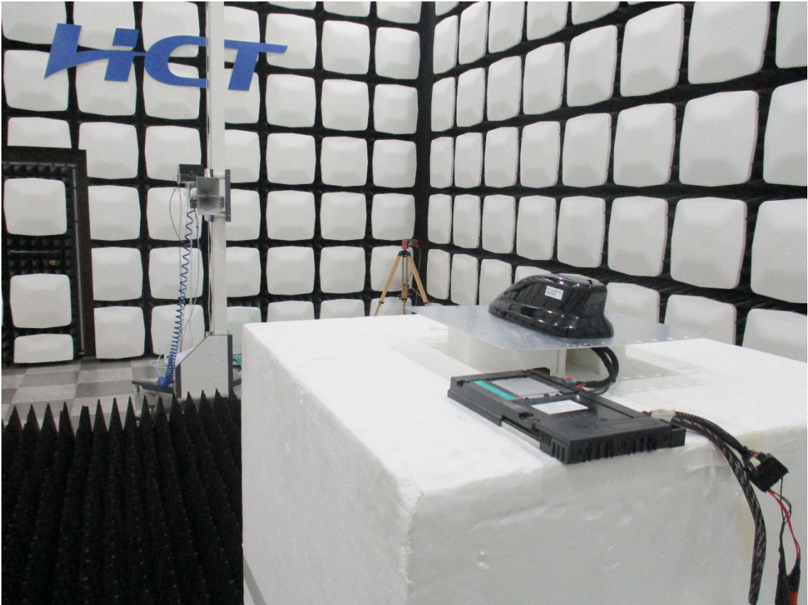
4-1. Radiated Test Setup Photo(BT1UG)-Horn Antenna, Antenna Mast: Horizontal
