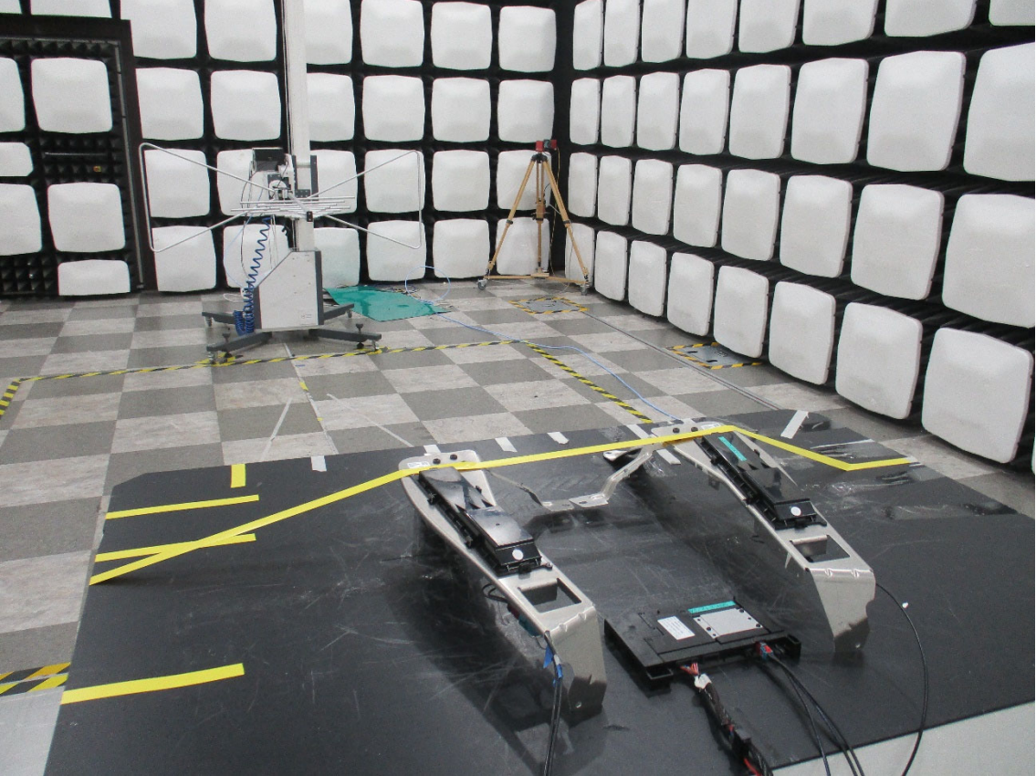
1-1. Radiated Test Setup Photo(Y2XX)-Bilog Antenna, Antenna Mast: Horizontal
