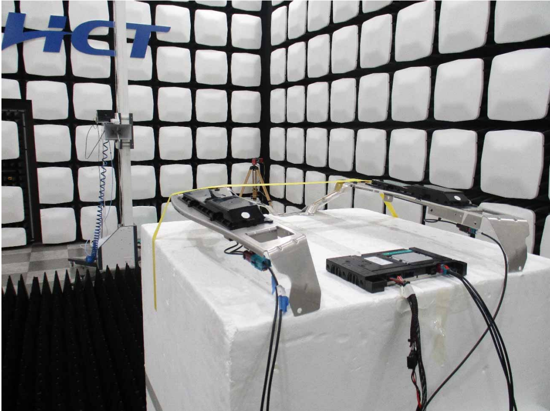
1-2. (Y2XX)-Horn Antenna, Antenna Mast: Vertical
