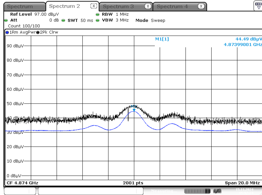
Radiated Spurious Emissions plot – Average Result (802.11b_1 Mbps, Ch.6 2nd Harmonic)
