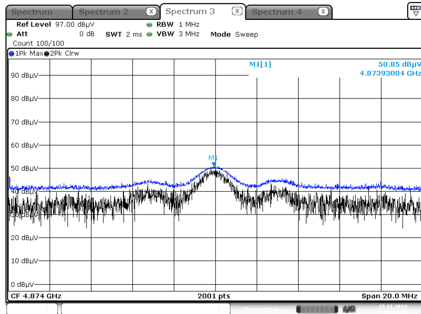
Radiated Spurious Emissions plot – Peak Result (802.11b_1 Mbps, Ch.6 2nd Harmonic)
