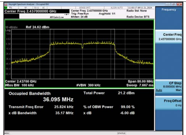
6 dB Bandwidth plot (802.11n_HT40-CH 6)
