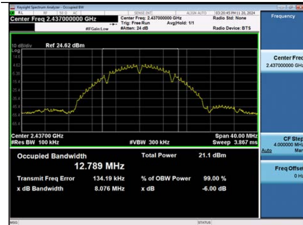
6 dB Bandwidth plot (802.11n_HT20-CH 6)
