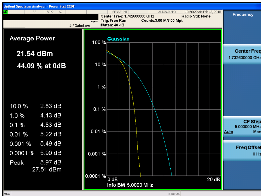
HSUPA1700 & Channel: 1413
