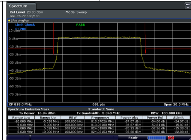
QPSK - Full RB
