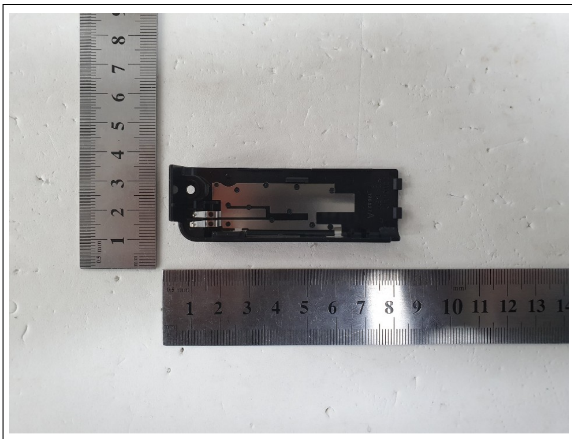
< Internal Antenna >
