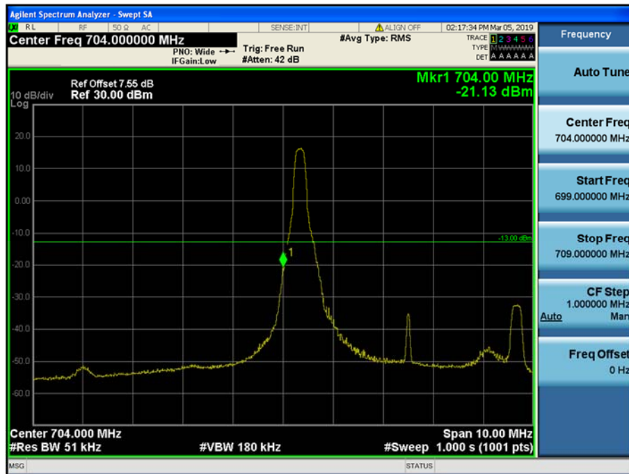
LTE Band 17 / 5MHz / 16QAM Offset/Size (1/0)
