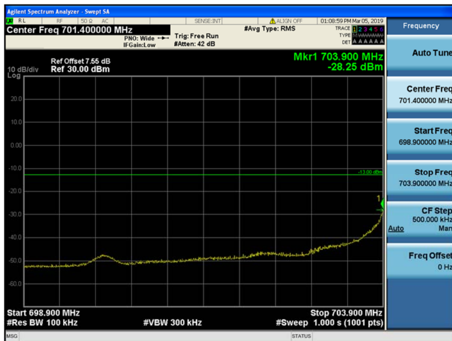
LTE Band 17 / 5MHz / QPSK Offset/Size (1/0)
