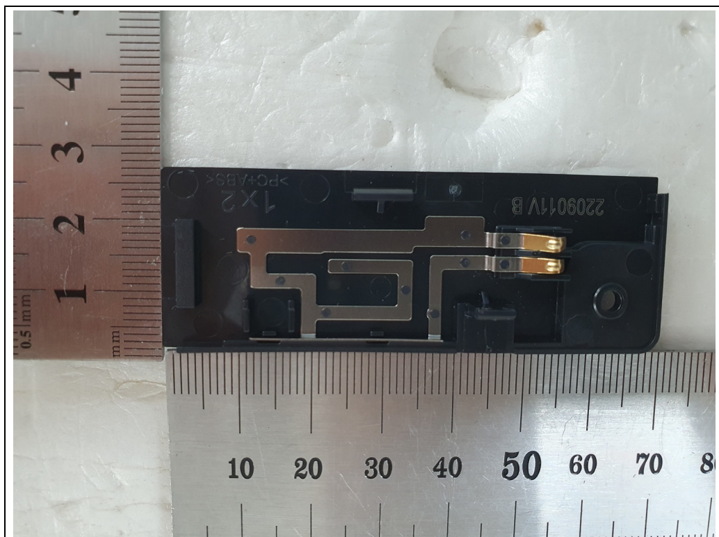
<Internal Antenna 2>
