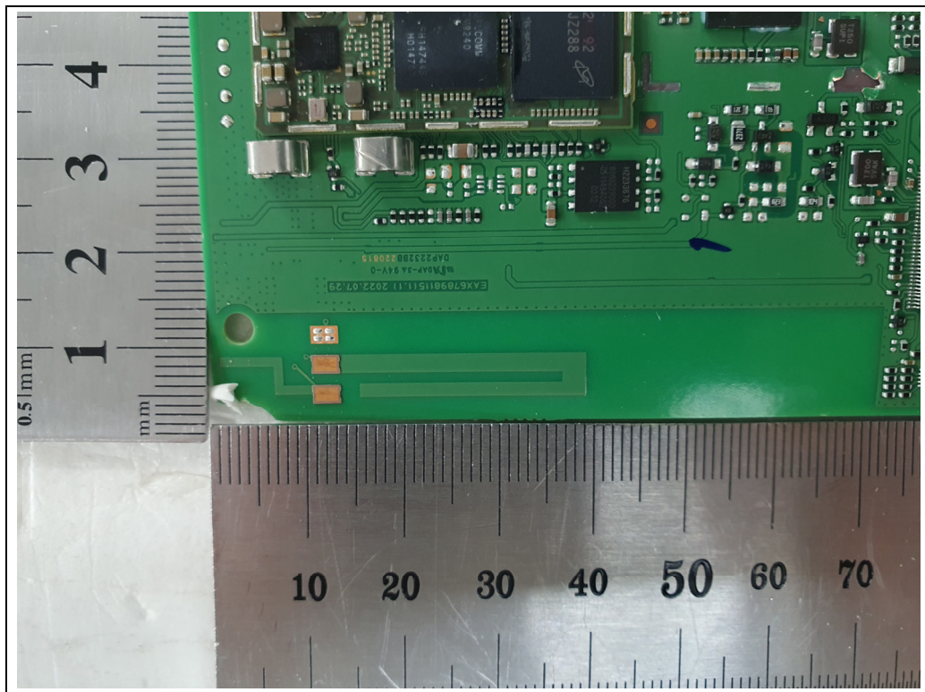
<Internal Antenna 1>
