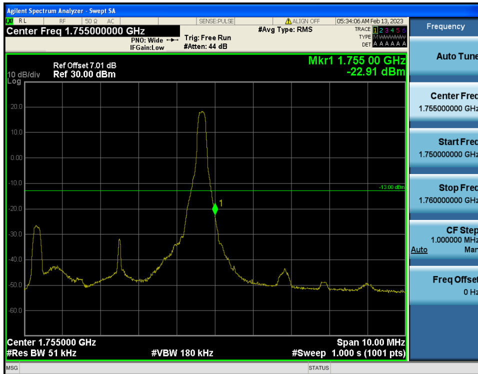
LTE Band 4 / 5MHz / QPSK - RB Size/Offset (1/24)
