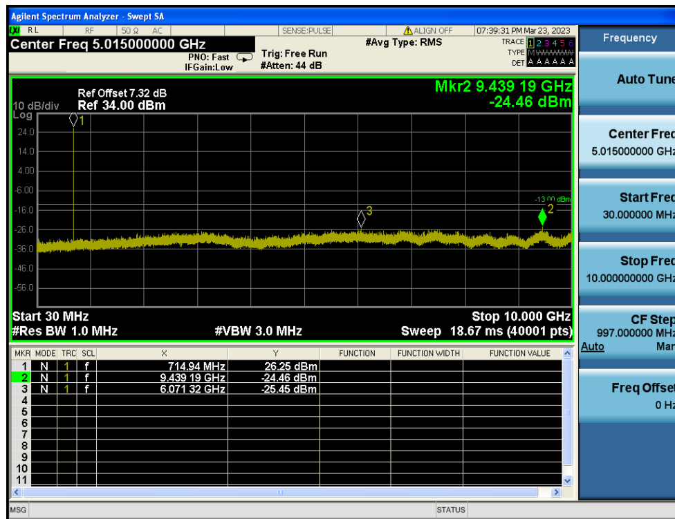
LTE Band 12 / 1.4MHz / QPSK - RB Size/Offset (1/0) - High Channel
