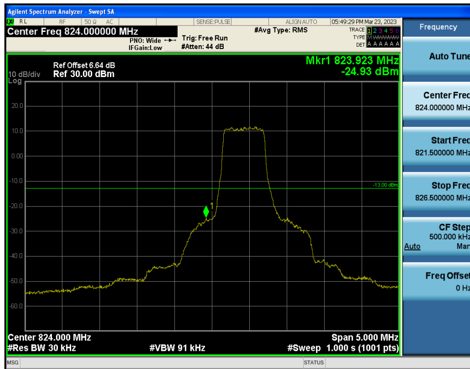
LTE Band 5 / 1.4MHz / QPSK - RB Size/Offset (3/0)
