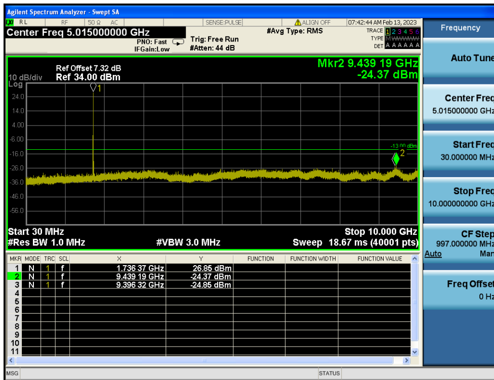
LTE Band 4 / 20MHz / QPSK - RB Size/Offset (1/0) - High Channel
