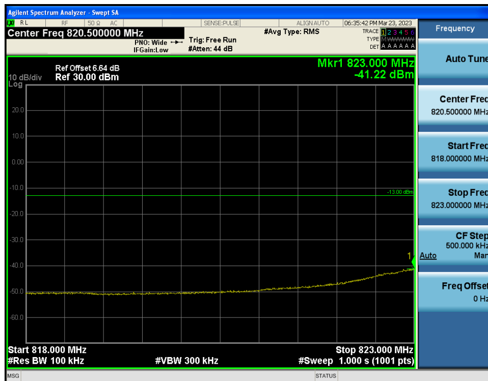
LTE Band 5 / 1.4MHz / 16QAM - RB Size/Offset (6/0)
