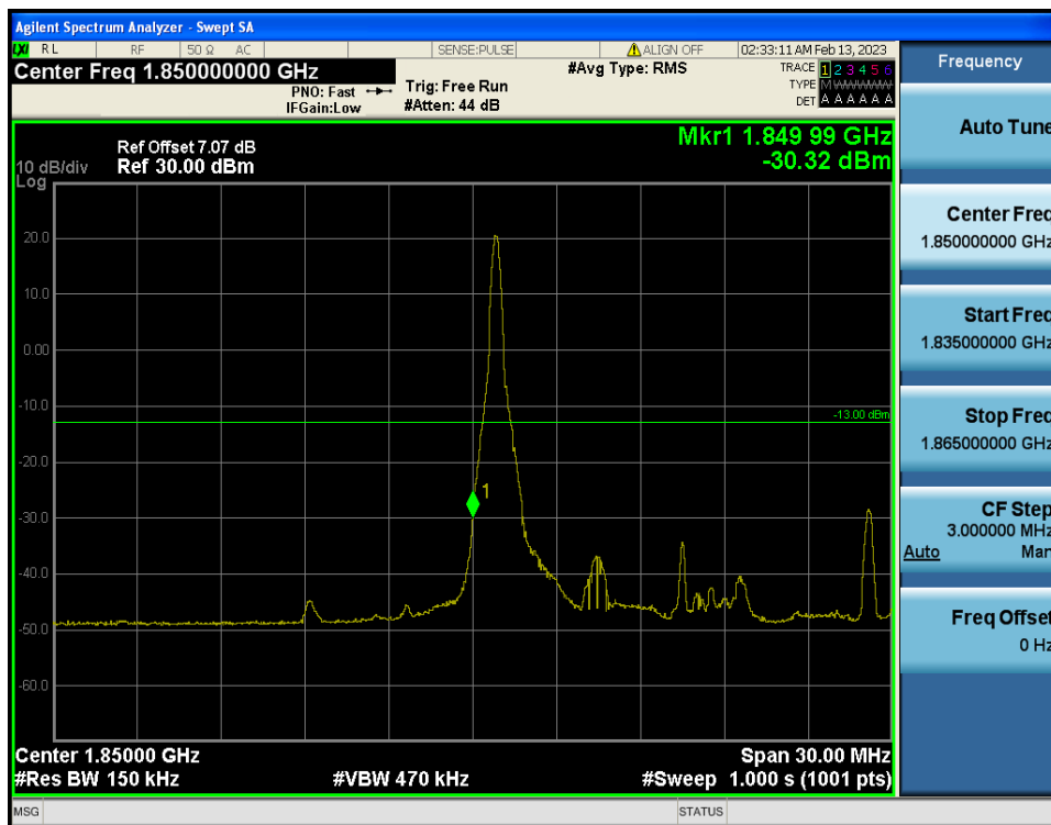
LTE Band 2 / 15MHz / 16QAM - RB Size/Offset (1/0)
