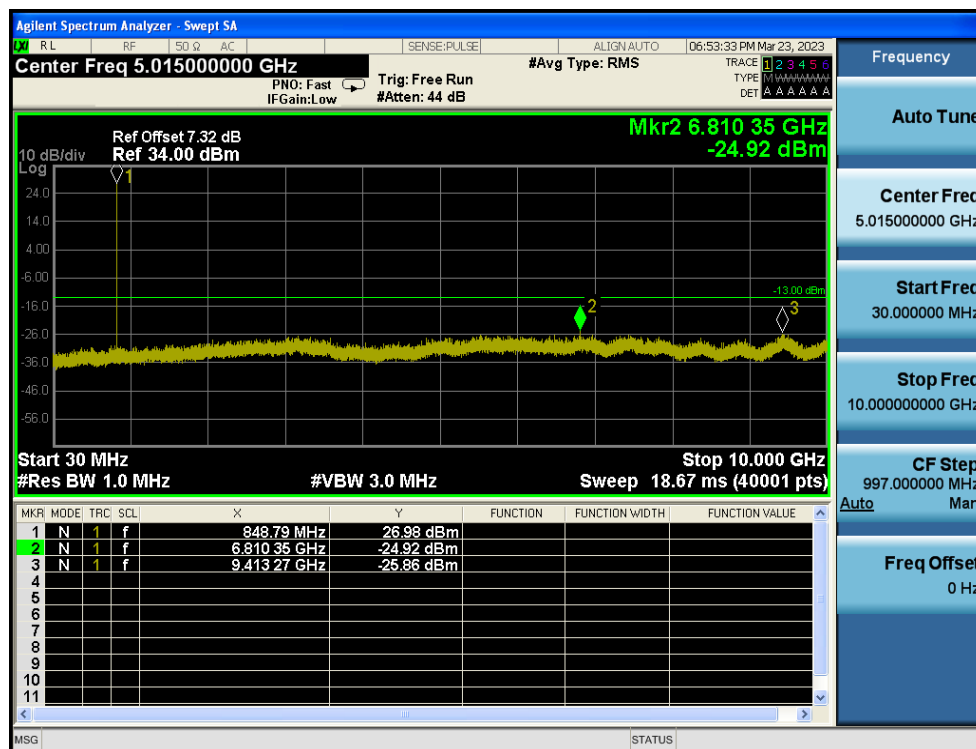
LTE Band 5 / 1.4MHz / 16QAM - RB Size/Offset (3/3) - High Channel
