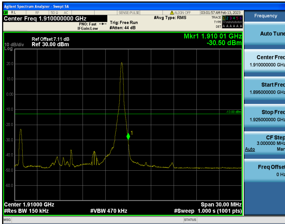
LTE Band 2 / 15MHz / 16QAM - RB Size/Offset (1/74)
