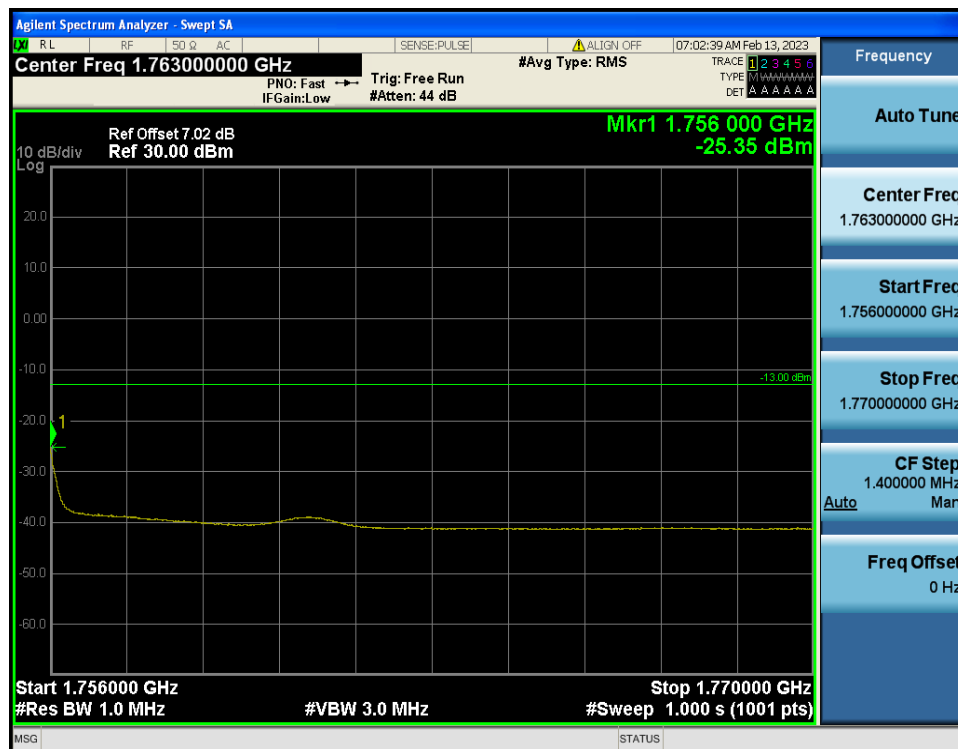
LTE Band 4 / 15MHz / QPSK - RB Size/Offset (1/74)
