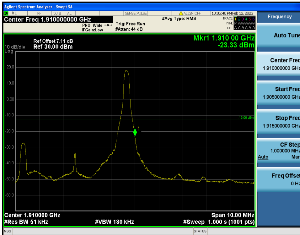
LTE Band 2 / 5MHz / QPSK - RB Size/Offset (1/24)
