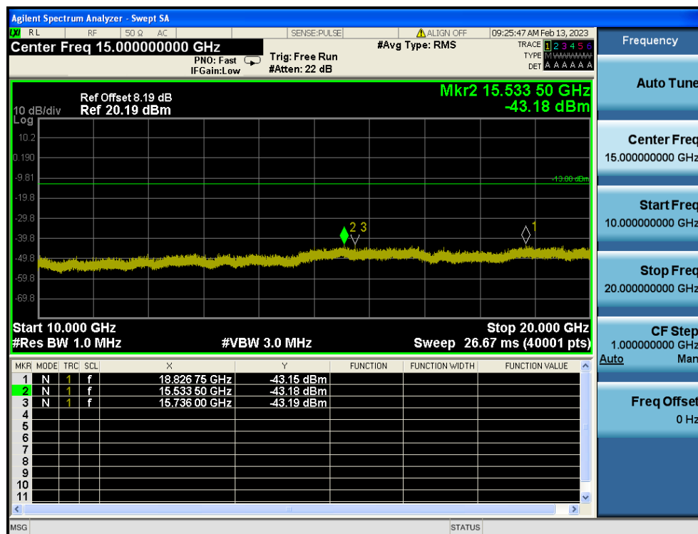
LTE Band 4 / 5MHz / 16QAM - RB Size/Offset (12/13) - High Channel
