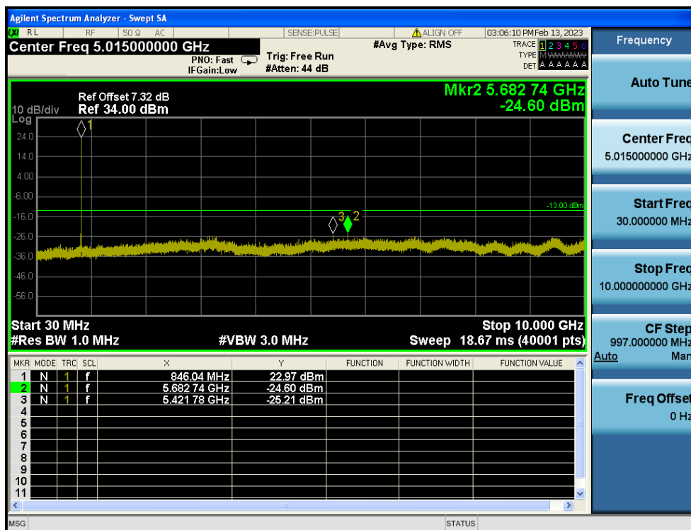
LTE Band 5 / 5MHz / 16QAM - RB Size/Offset (12/6) - High Channel
