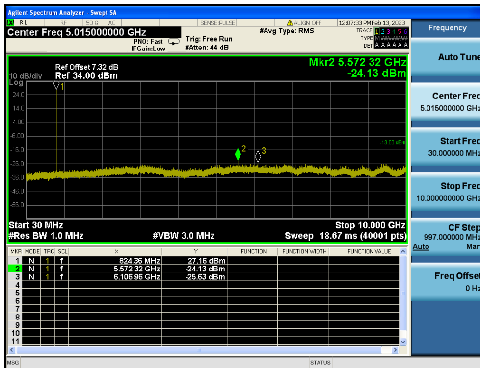
LTE Band 5 / 3MHz / QPSK - RB Size/Offset (1/0) - Low Channel
