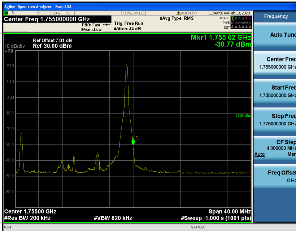
LTE Band 4 / 20MHz / 16QAM - RB Size/Offset (1/99)
