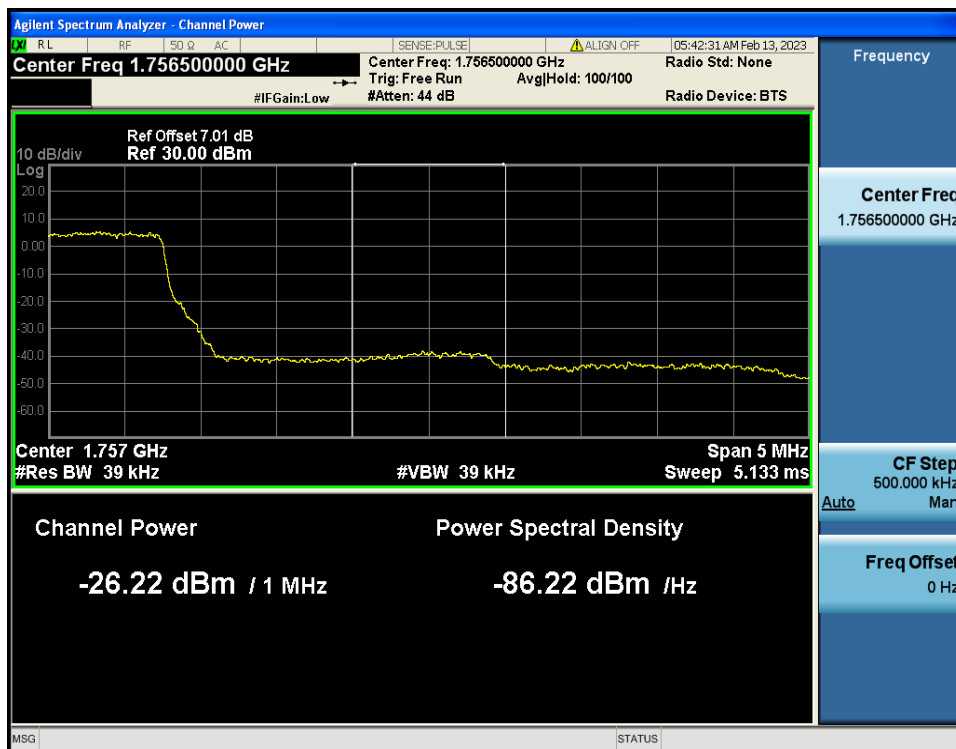
LTE Band 4 / 5MHz / QPSK - RB Size/Offset (12/13)
