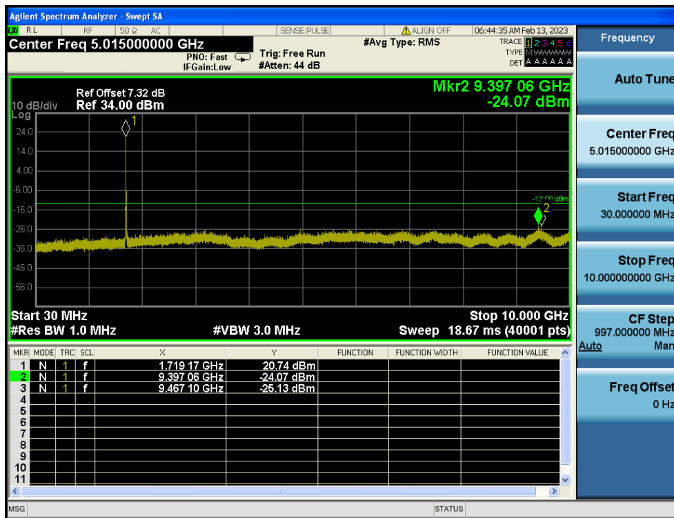
LTE Band 4 / 15MHz / QPSK - RB Size/Offset (36/18) - Low Channel
