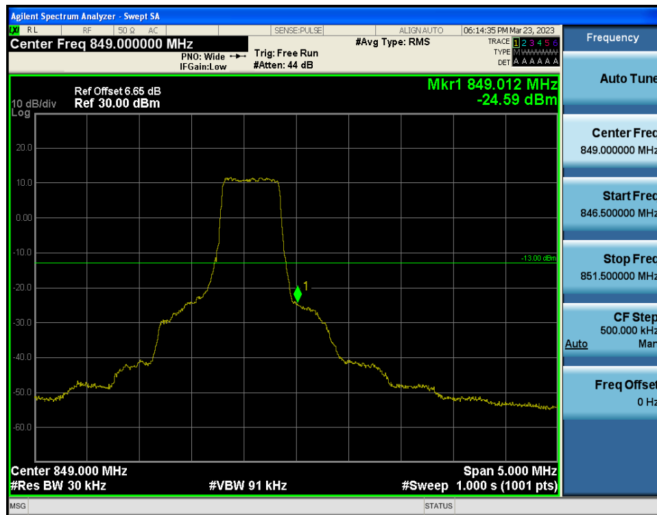
LTE Band 5 / 1.4MHz / QPSK - RB Size/Offset (3/3)
