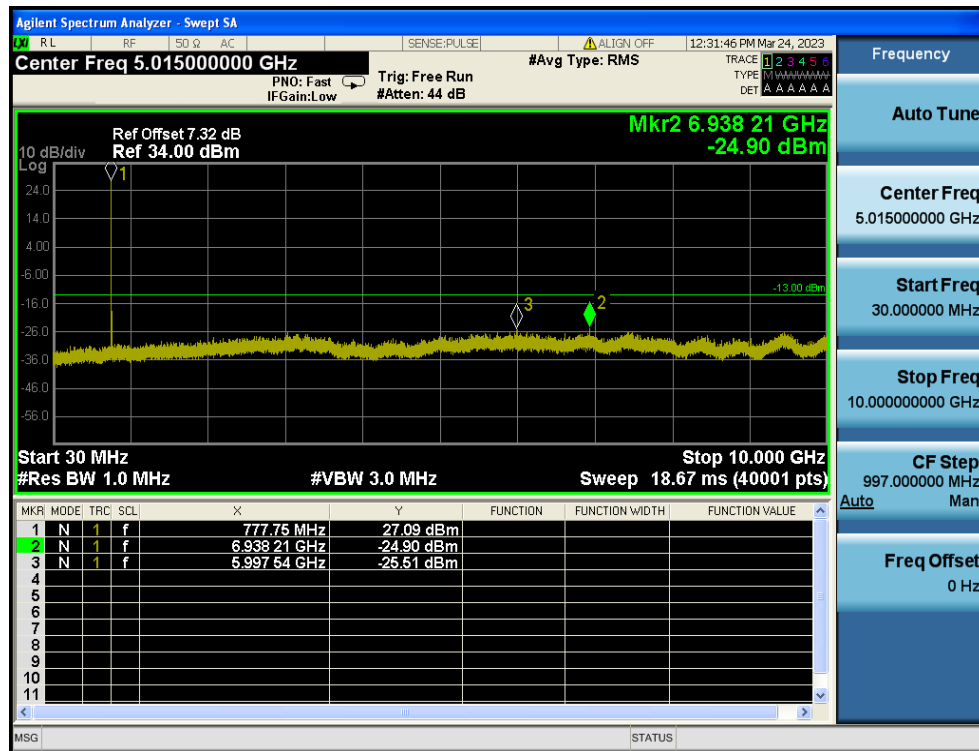
LTE Band 13 / 10MHz / 16QAM - RB Size/Offset (1/0) - Low Channel
