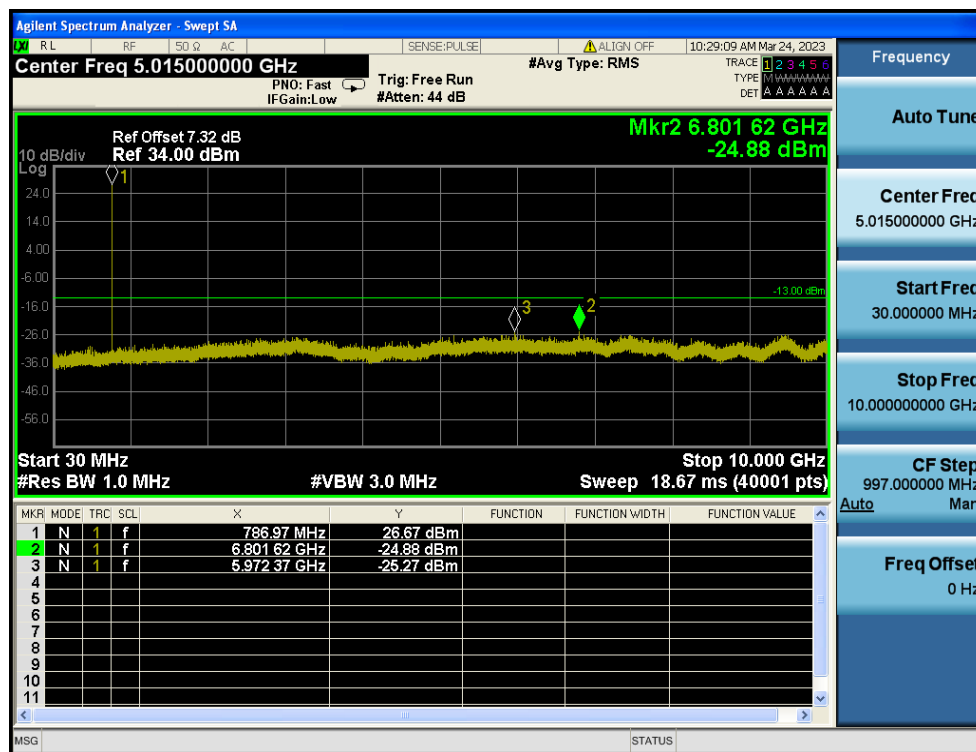
LTE Band 13 / 5MHz / QPSK - RB Size/Offset (1/24) - High Channel
