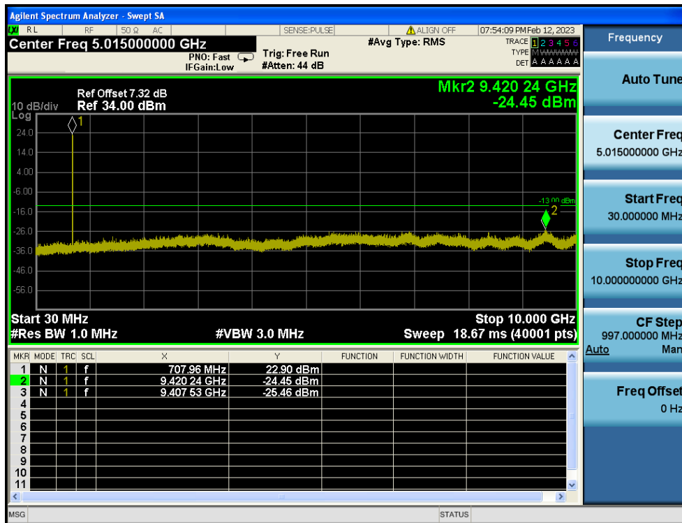
LTE Band 12 / 5MHz / 16QAM - RB Size/Offset (12/6) - Mid Channel
