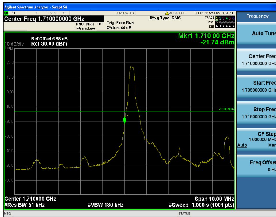
LTE Band 4 / 5MHz / 16QAM - RB Size/Offset (1/0)
