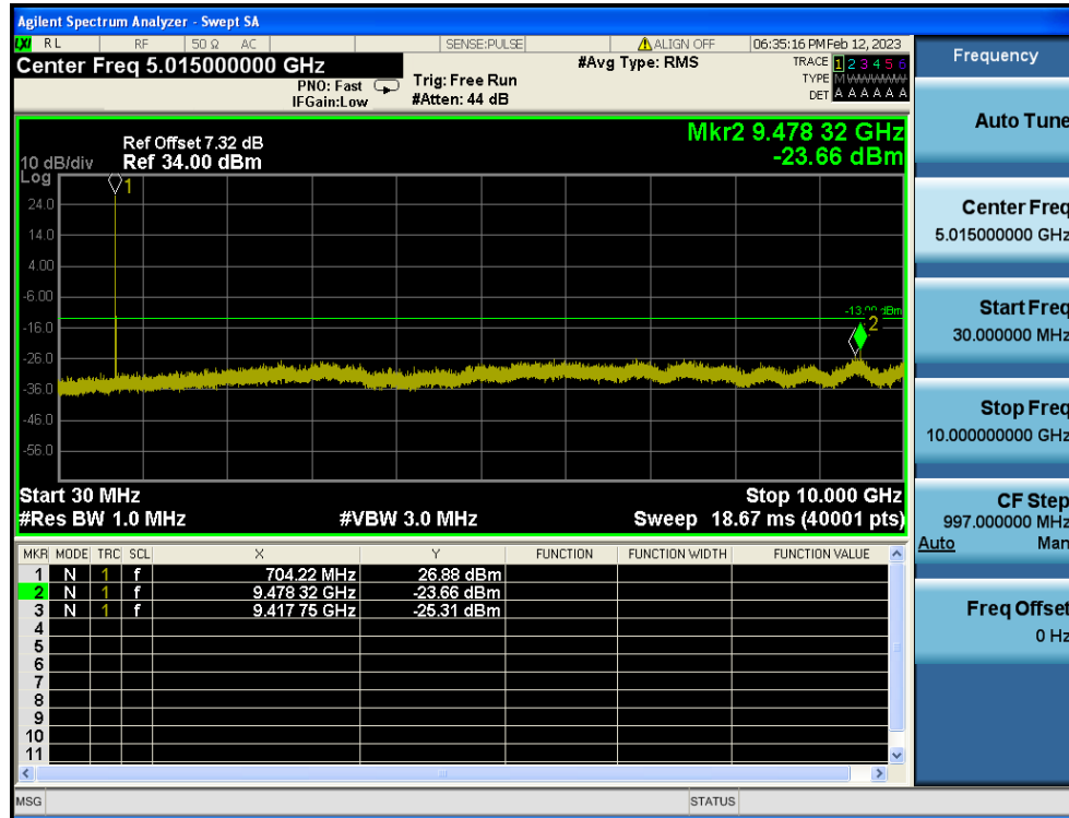
LTE Band 12 / 10MHz / QPSK - RB Size/Offset (1/25) - Low Channel
