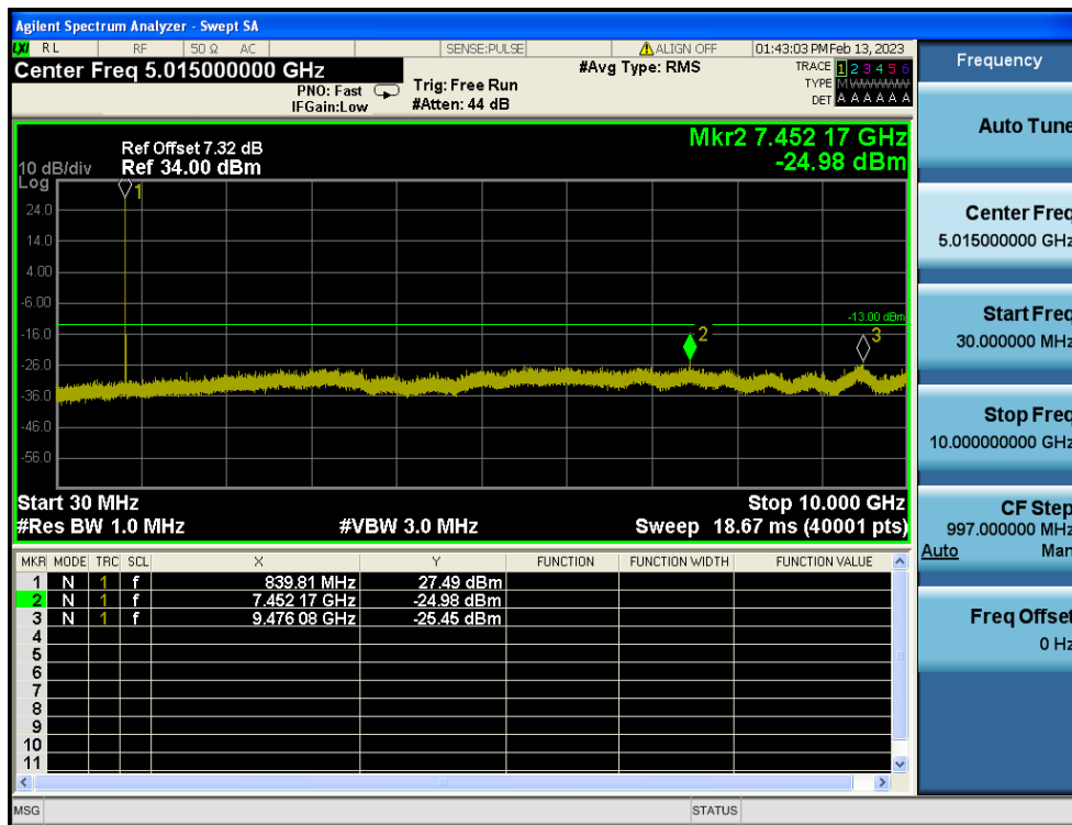
LTE Band 5 / 10MHz / QPSK - RB Size/Offset (1/0) - High Channel
