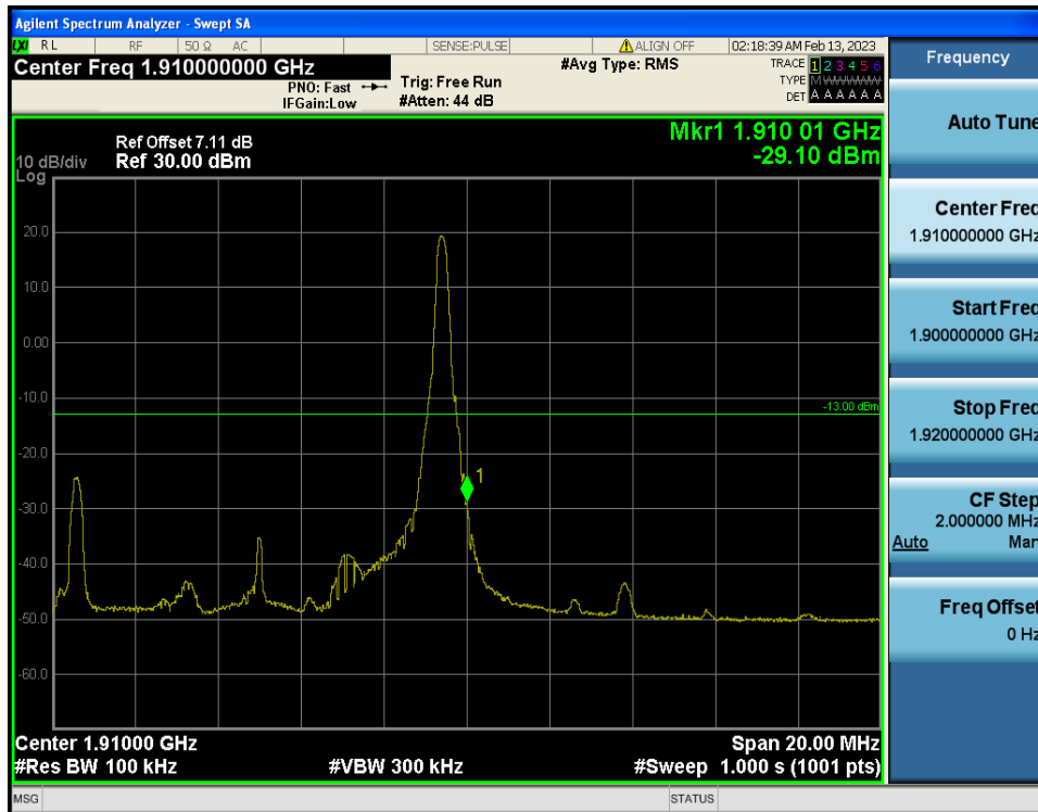
LTE Band 2 / 10MHz / 16QAM - RB Size/Offset (1/49)
