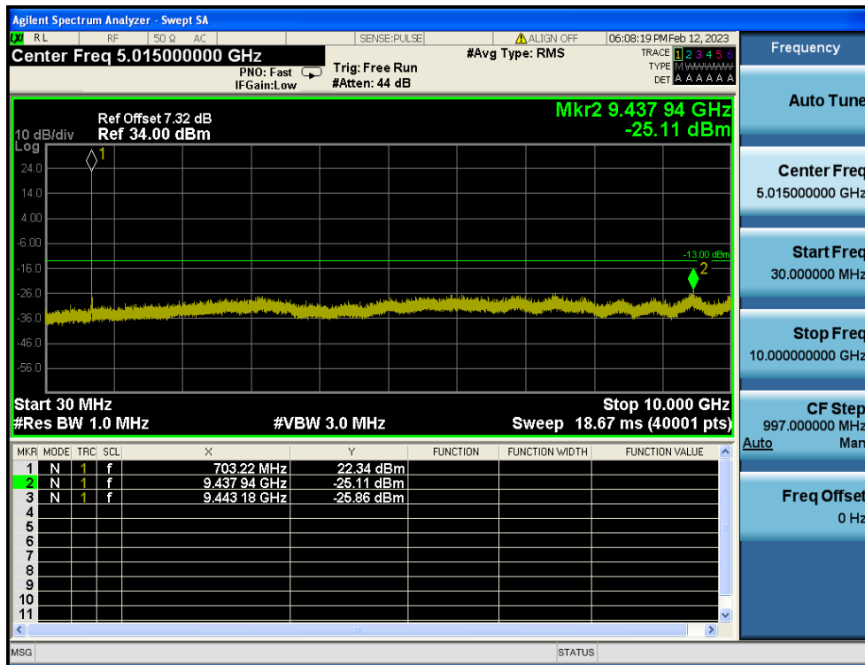
LTE Band 12 / 5MHz / QPSK - RB Size/Offset (12/13) - Low Channel
