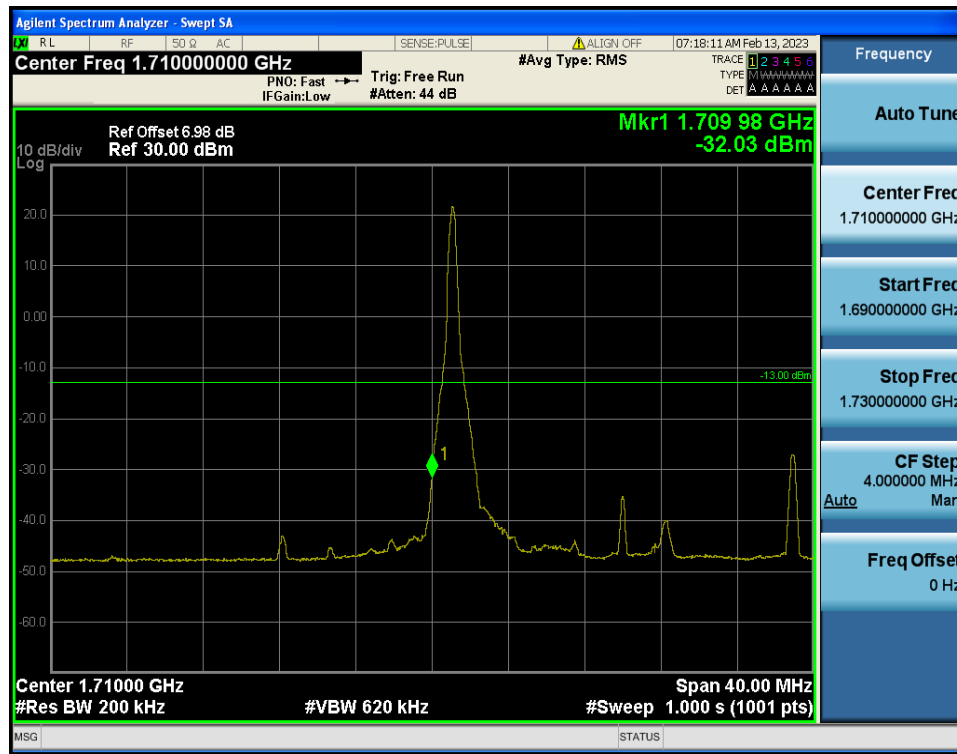
LTE Band 4 / 20MHz / QPSK - RB Size/Offset (1/0)
