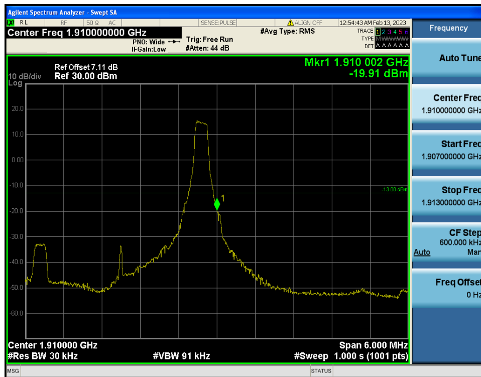
LTE Band 2 / 3MHz / 16QAM - RB Size/Offset (1/14)
