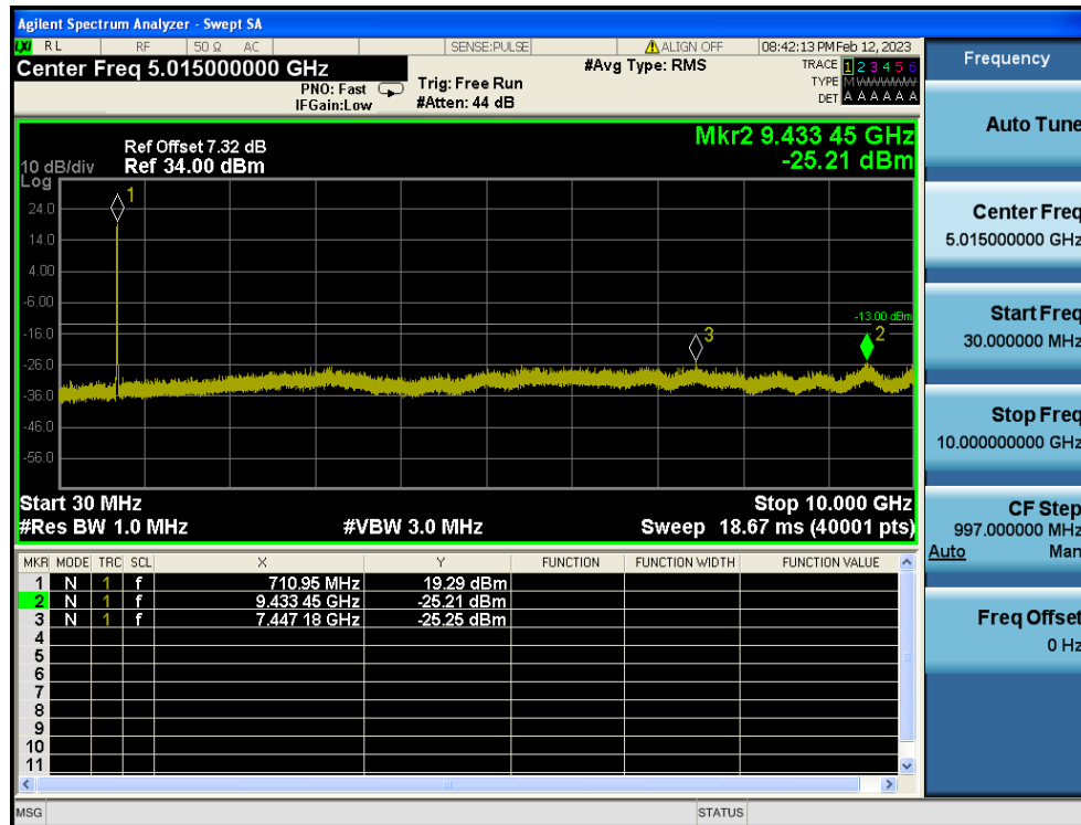
LTE Band 12 / 10MHz / 16QAM - RB Size/Offset (50/0) - High Channel
