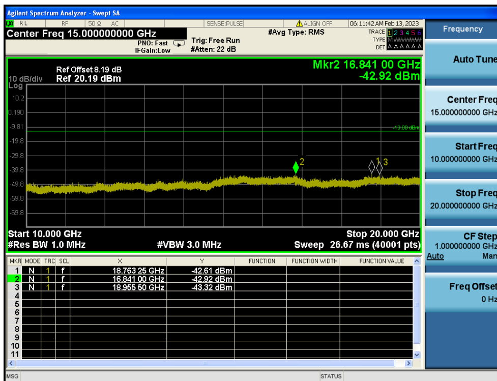
LTE Band 4 / 10MHz / QPSK - RB Size/Offset (25/25) - Mid Channel
