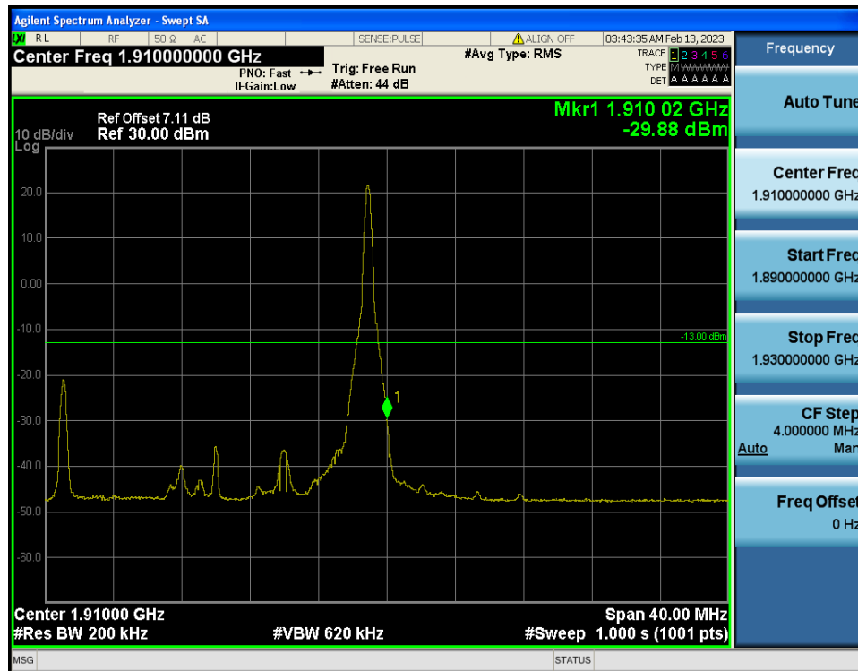
LTE Band 2 / 20MHz / 16QAM - RB Size/Offset (1/99)
