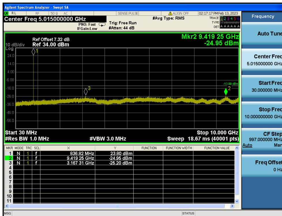
LTE Band 5 / 3MHz / 16QAM - RB Size/Offset (8/4) - Mid Channel
