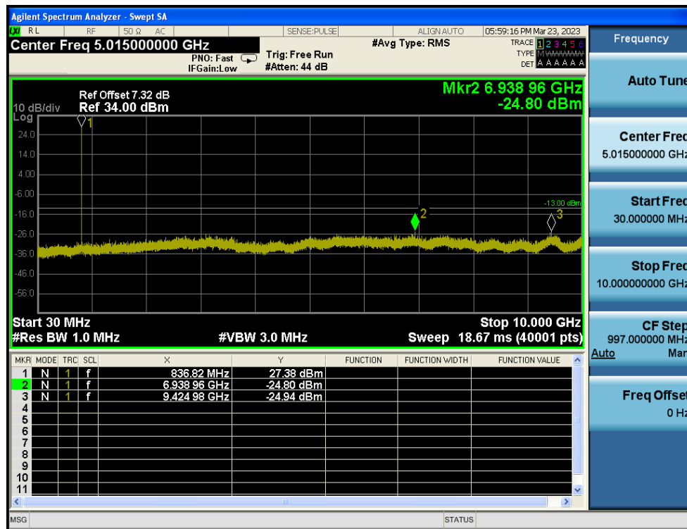
LTE Band 5 / 1.4MHz / QPSK - RB Size/Offset (1/2) - Mid Channel
