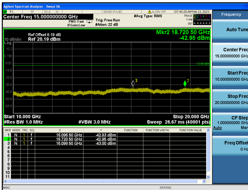
LTE Band 4 / 20MHz / QPSK - RB Size/Offset (100/0) - Mid Channel
