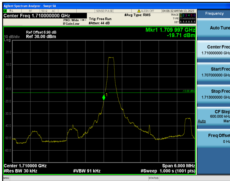
LTE Band 4 / 3MHz / QPSK - RB Size/Offset (1/0)
