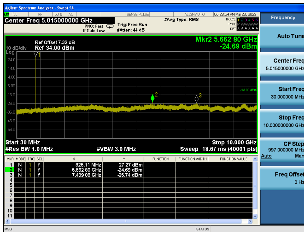
LTE Band 5 / 1.4MHz / 16QAM - RB Size/Offset (1/2) - Low Channel
