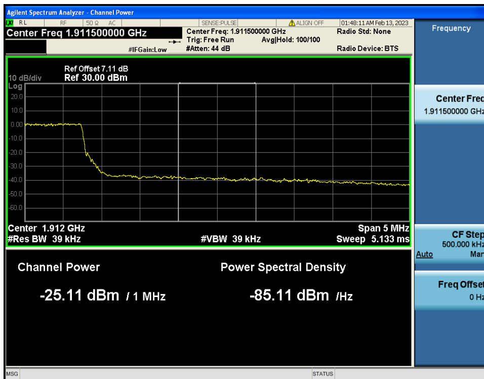
LTE Band 2 / 5MHz / 16QAM - RB Size/Offset (25/0)
