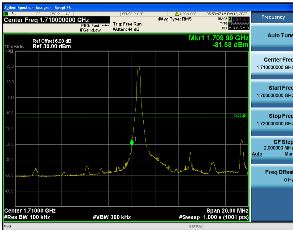
LTE Band 4 / 10MHz / QPSK - RB Size/Offset (1/0)
