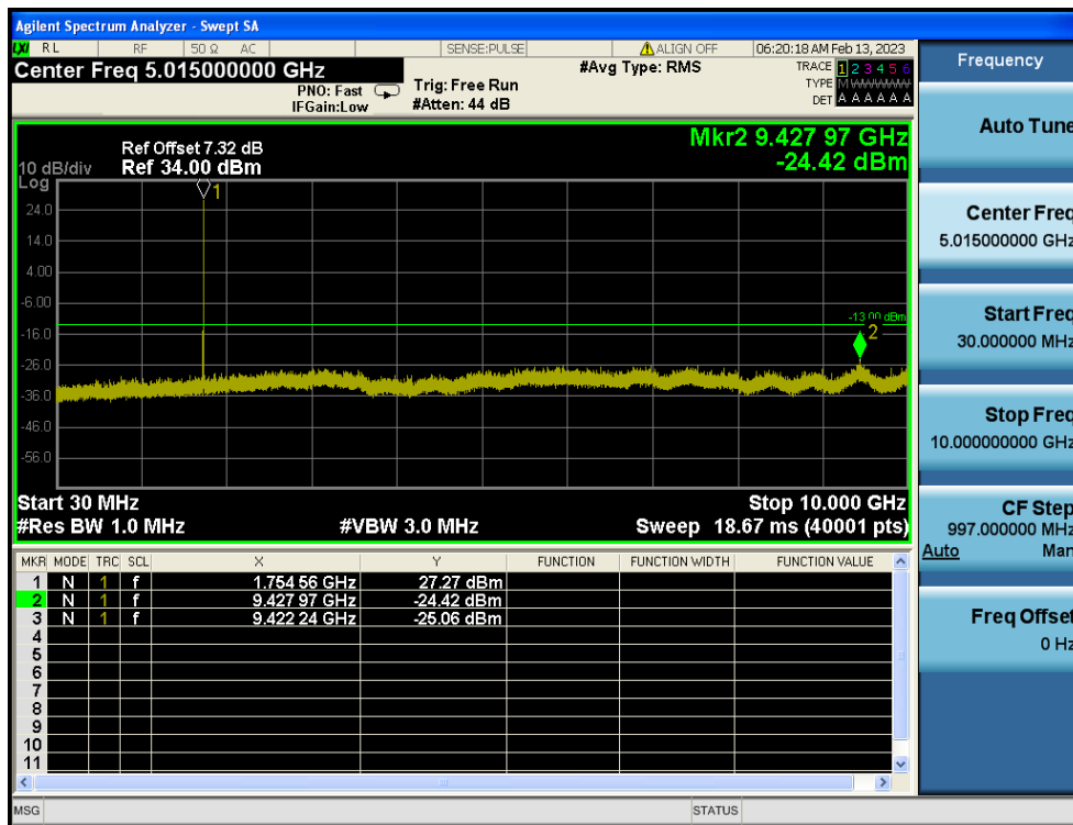
LTE Band 4 / 10MHz / QPSK - RB Size/Offset (1/49) - High Channel
