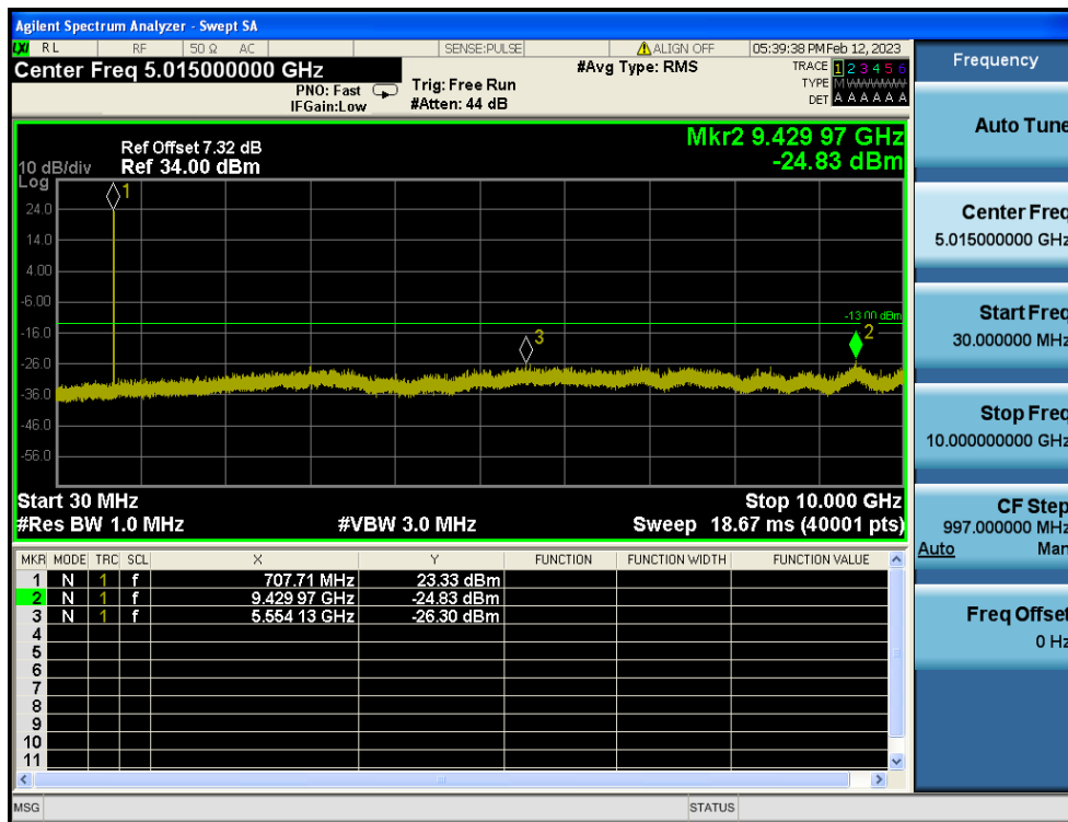
LTE Band 12 / 3MHz / QPSK - RB Size/Offset (8/7) - Mid Channel
