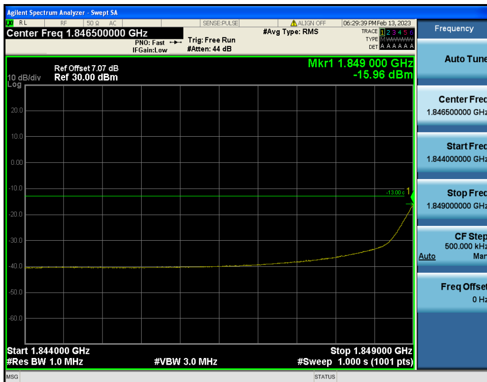
LTE Band 2 / 1.4MHz / QPSK - RB Size/Offset (3/2)
