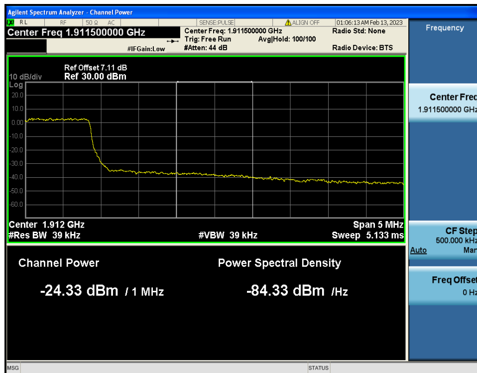
LTE Band 2 / 3MHz / 16QAM - RB Size/Offset (15/0)
