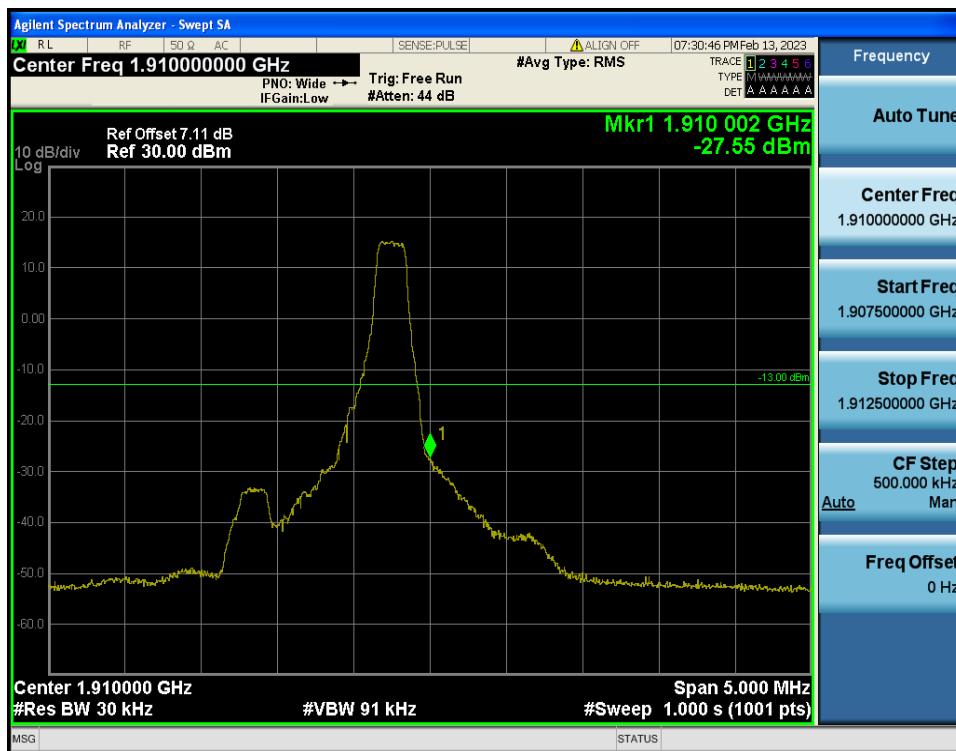
LTE Band 2 / 1.4MHz / 16QAM - RB Size/Offset (1/5)
