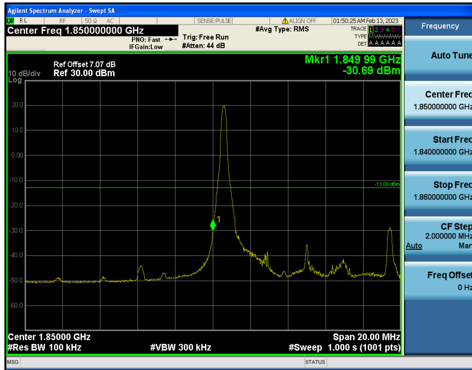
LTE Band 2 / 10MHz / 16QAM - RB Size/Offset (1/0)
