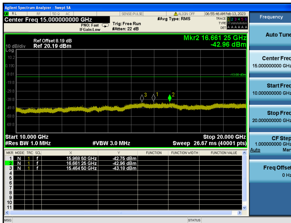
LTE Band 4 / 15MHz / QPSK - RB Size/Offset (75/0) - Mid Channel
