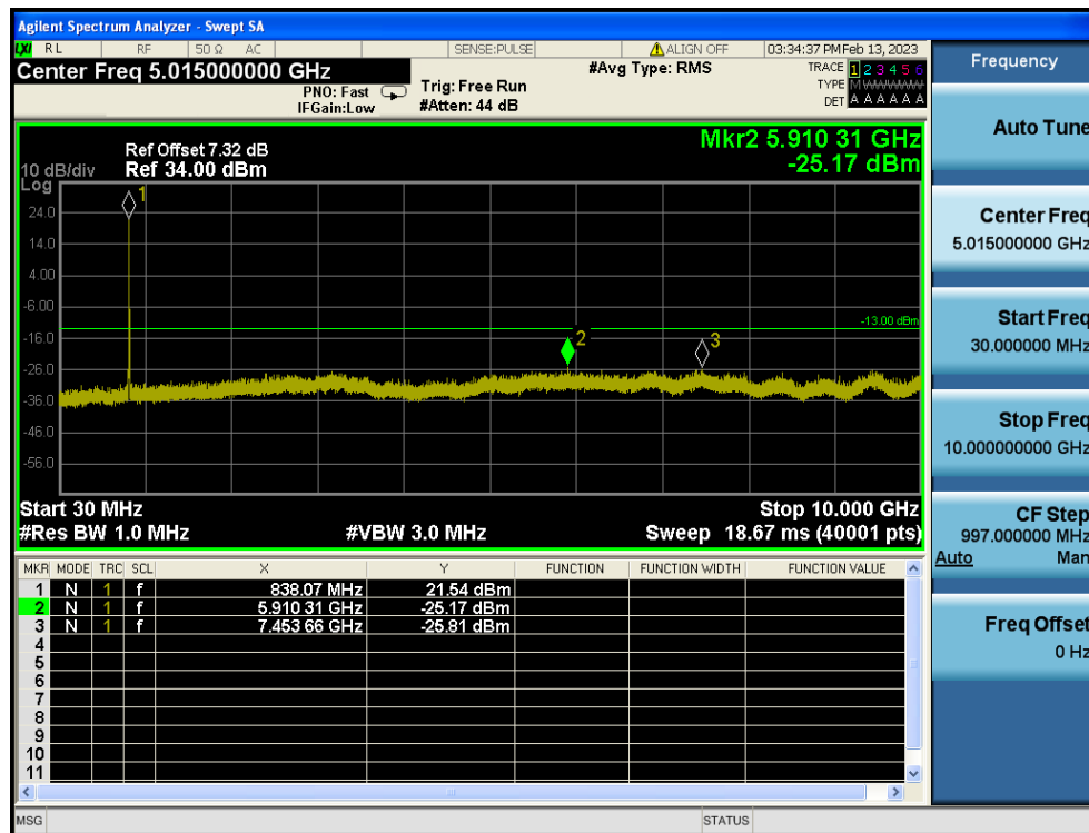
LTE Band 5 / 10MHz / 16QAM - RB Size/Offset (25/25) - Mid Channel
