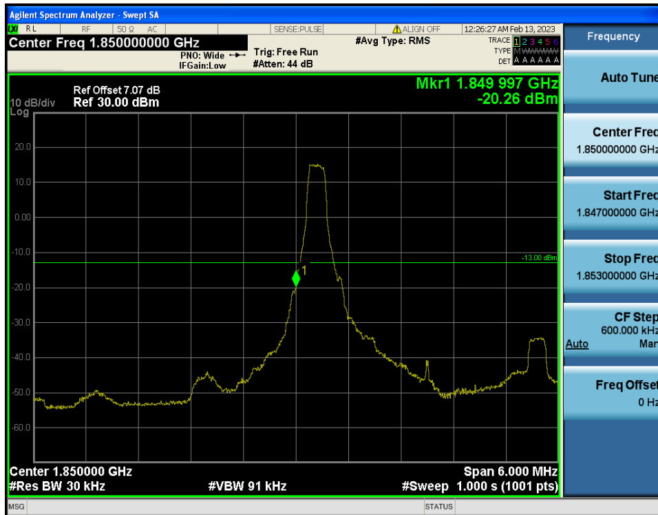
LTE Band 2 / 3MHz / 16QAM - RB Size/Offset (1/0)
