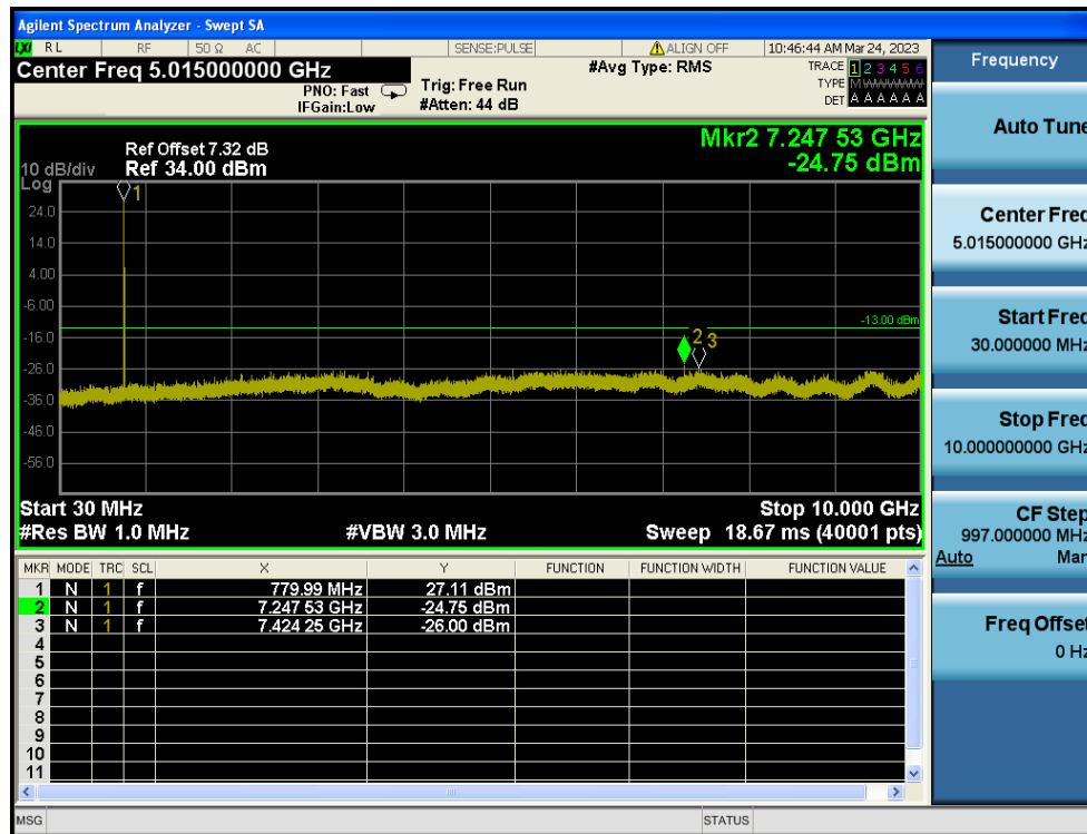
LTE Band 13 / 5MHz / 16QAM - RB Size/Offset (1/12) - Low Channel
