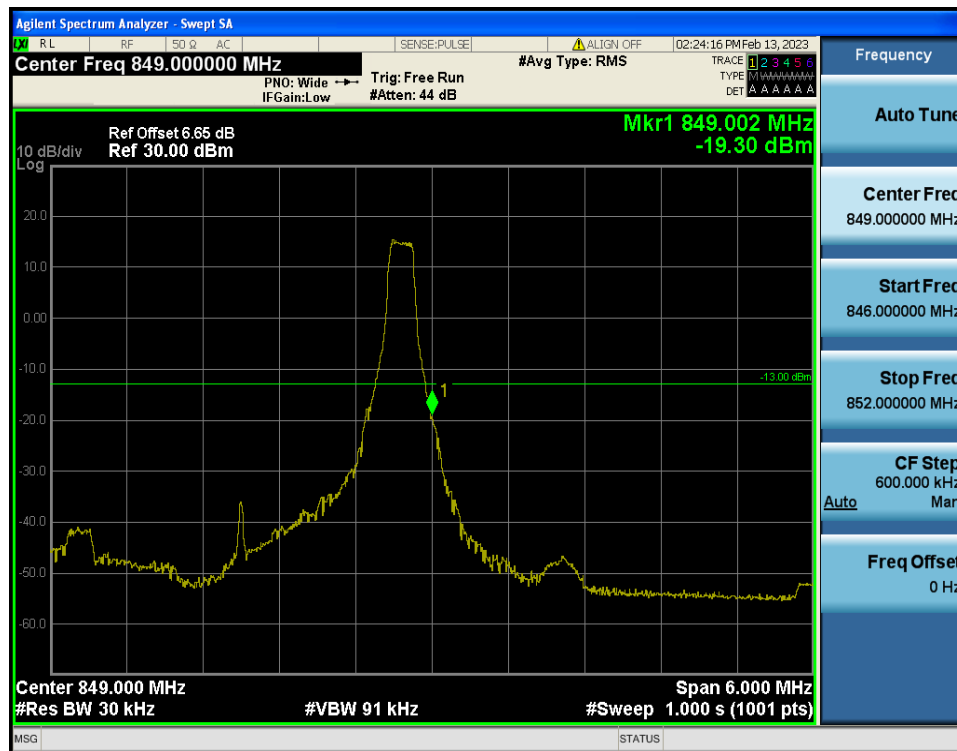
LTE Band 5 / 3MHz / 16QAM - RB Size/Offset (1/14)
