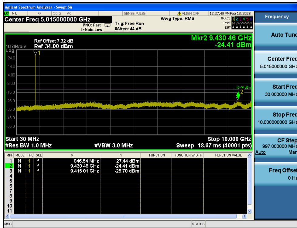
LTE Band 5 / 3MHz / QPSK - RB Size/Offset (1/0) - High Channel
