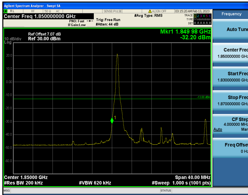
LTE Band 2 / 20MHz / 16QAM - RB Size/Offset (1/0)
