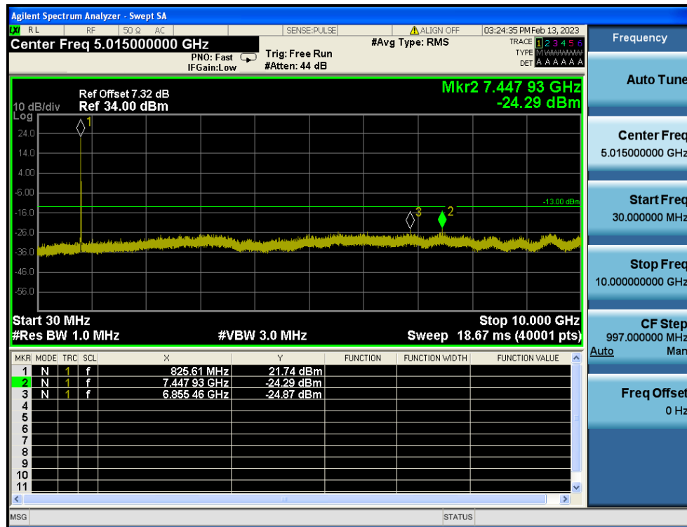
LTE Band 5 / 10MHz / 16QAM - RB Size/Offset (25/0) - Low Channel
