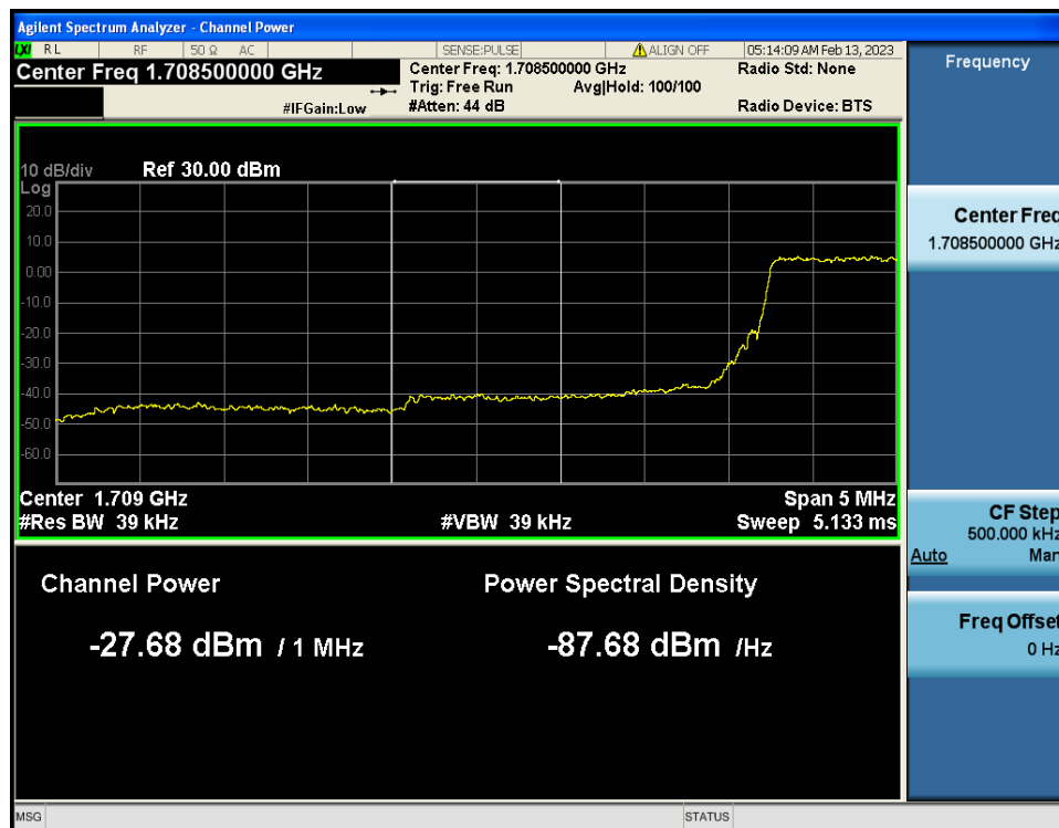
LTE Band 4 / 5MHz / QPSK - RB Size/Offset (12/0)
