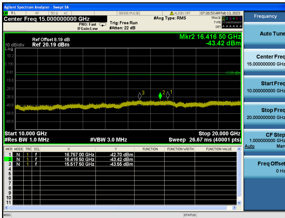
LTE Band 4 / 20MHz / QPSK - RB Size/Offset (50/0) - Low Channel
