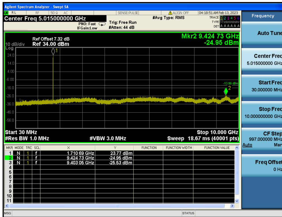
LTE Band 4 / 3MHz / QPSK - RB Size/Offset (8/0) - Low Channel
