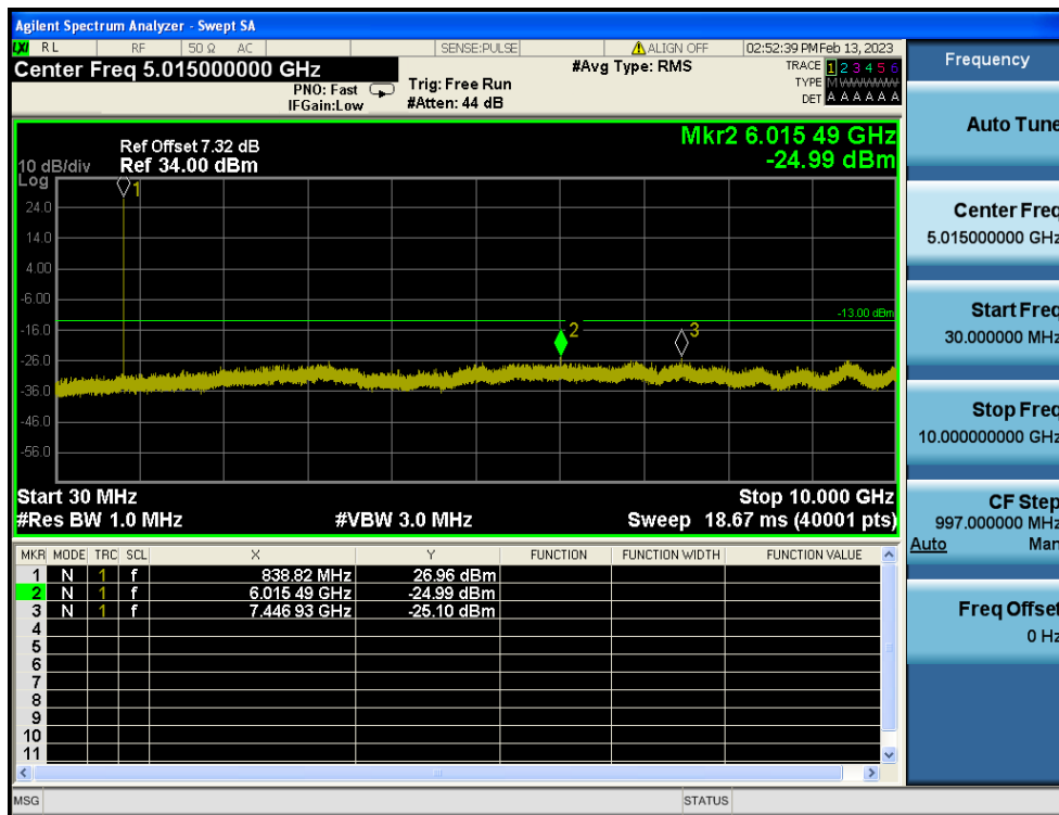
LTE Band 5 / 5MHz / 16QAM - RB Size/Offset (1/24) - Mid Channel
