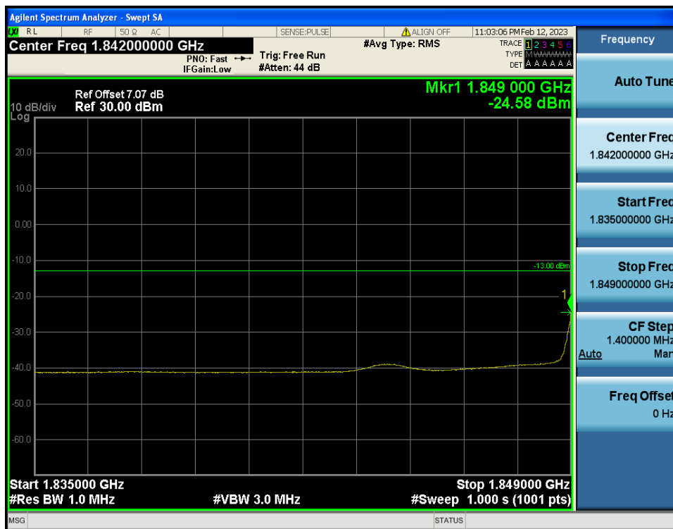
LTE Band 2 / 15MHz / QPSK - RB Size/Offset (1/0)
