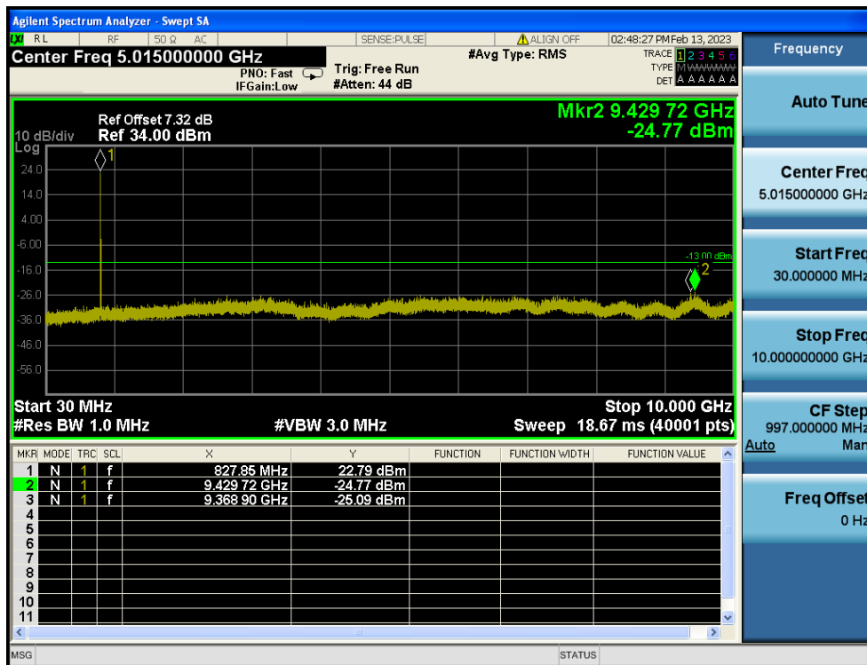
LTE Band 5 / 5MHz / 16QAM - RB Size/Offset (12/13) - Low Channel
