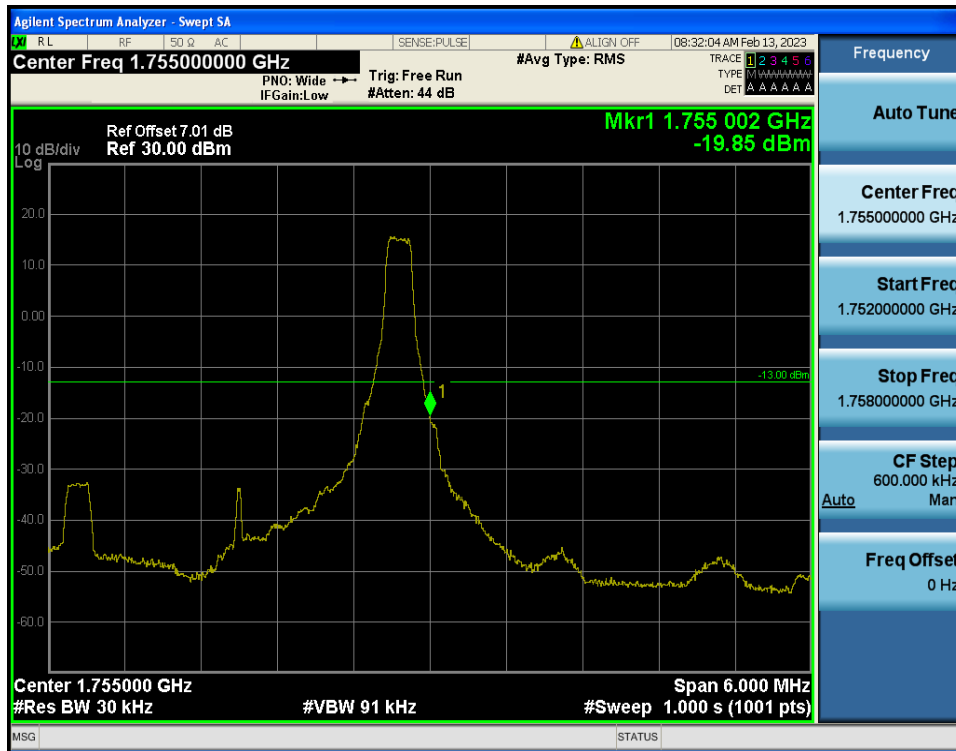
LTE Band 4 / 3MHz / 16QAM - RB Size/Offset (1/14)
