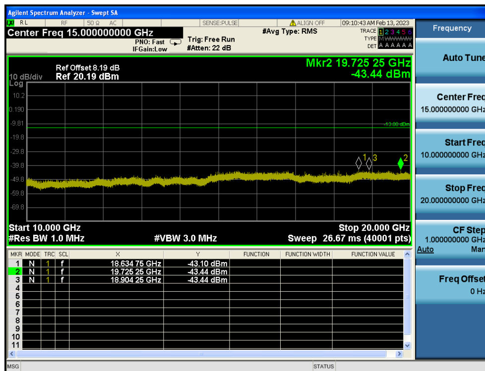
LTE Band 4 / 5MHz / 16QAM - RB Size/Offset (25/0) - Mid Channel
