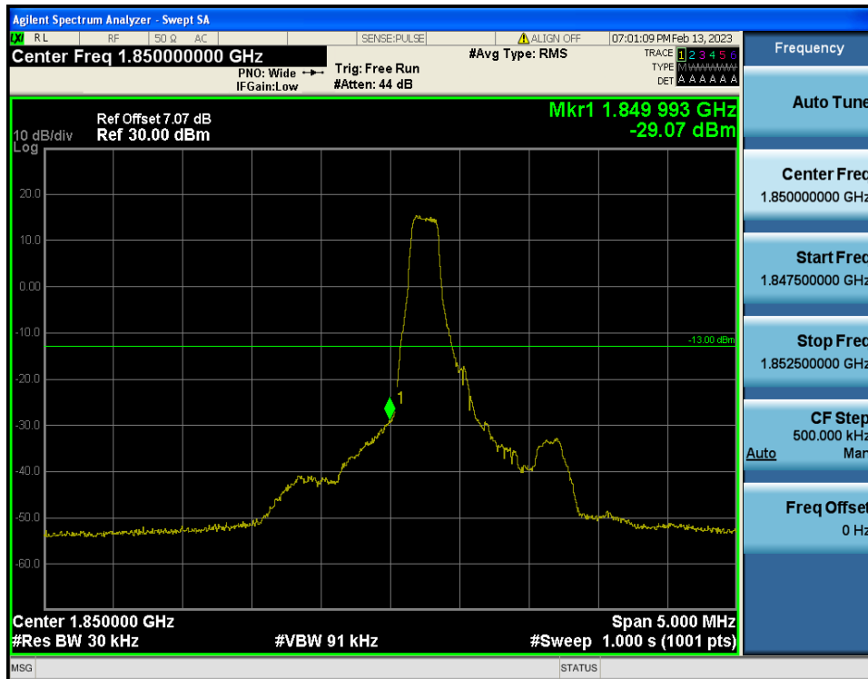
LTE Band 2 / 1.4MHz / 16QAM - RB Size/Offset (1/0)
