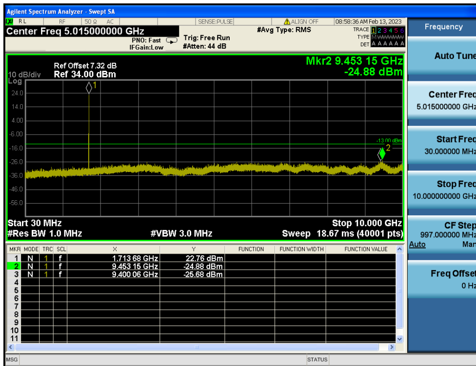
LTE Band 4 / 5MHz / 16QAM - RB Size/Offset (12/6) - Low Channel
