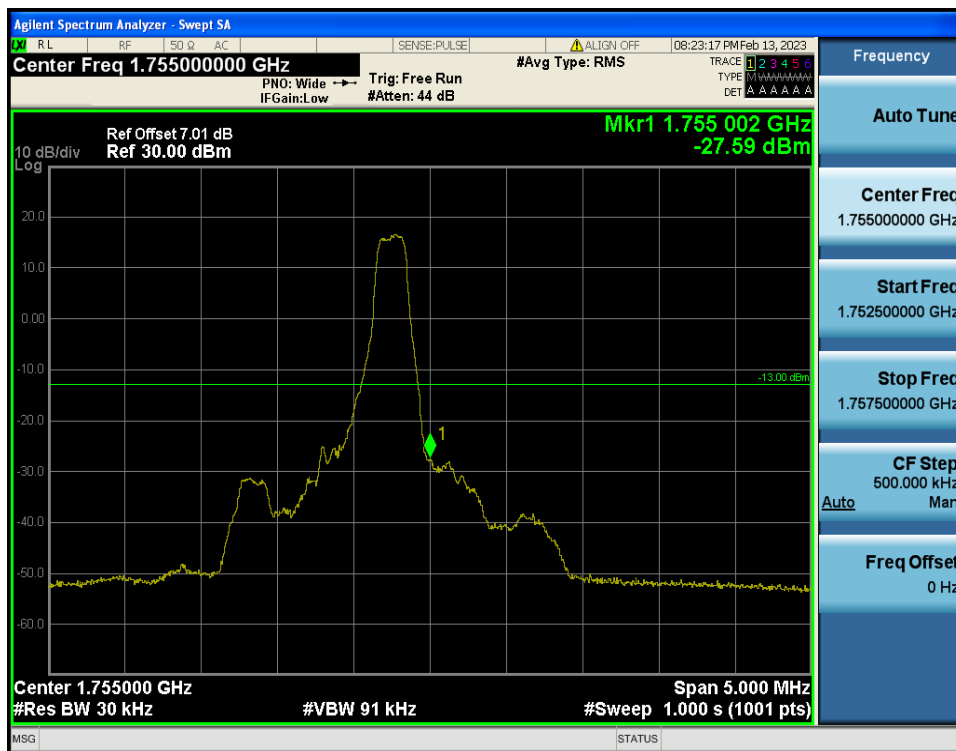
LTE Band 4 / 1.4MHz / QPSK - RB Size/Offset (1/5)
