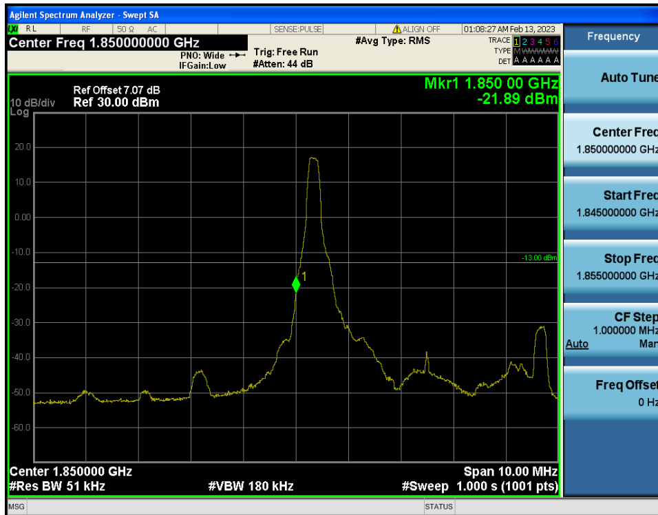
LTE Band 2 / 5MHz / 16QAM - RB Size/Offset (1/0)
