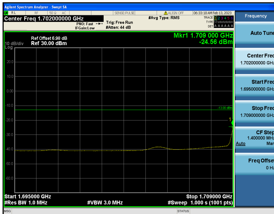
LTE Band 4 / 15MHz / QPSK - RB Size/Offset (1/0)
