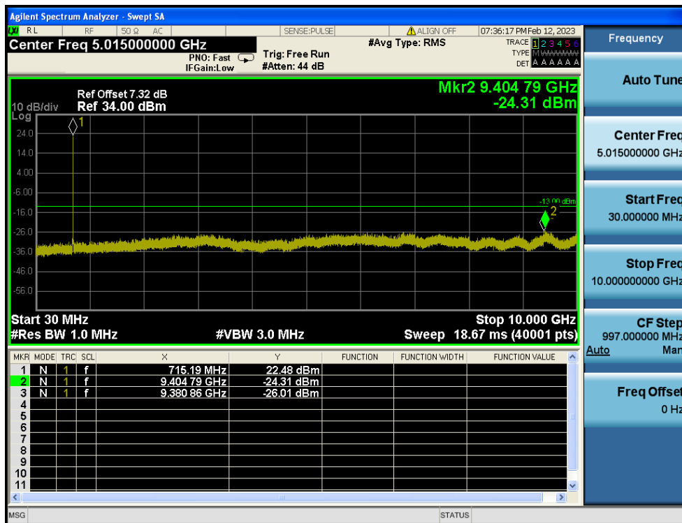
LTE Band 12 / 3MHz / 16QAM - RB Size/Offset (15/0) - High Channel
