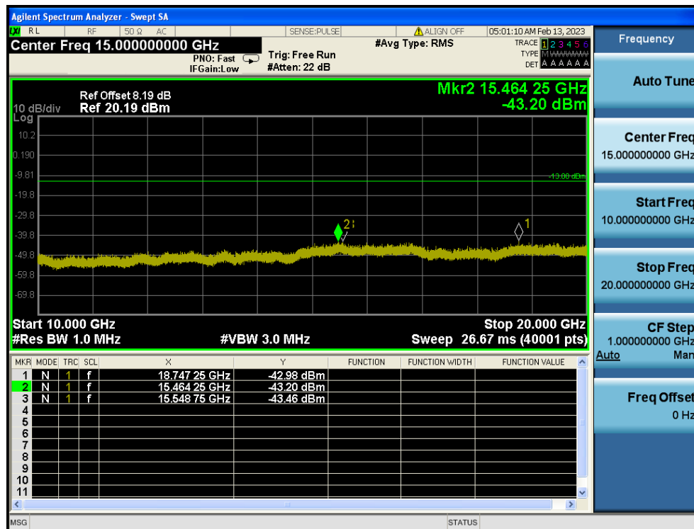
LTE Band 4 / 3MHz / QPSK - RB Size/Offset (15/0) - High Channel
