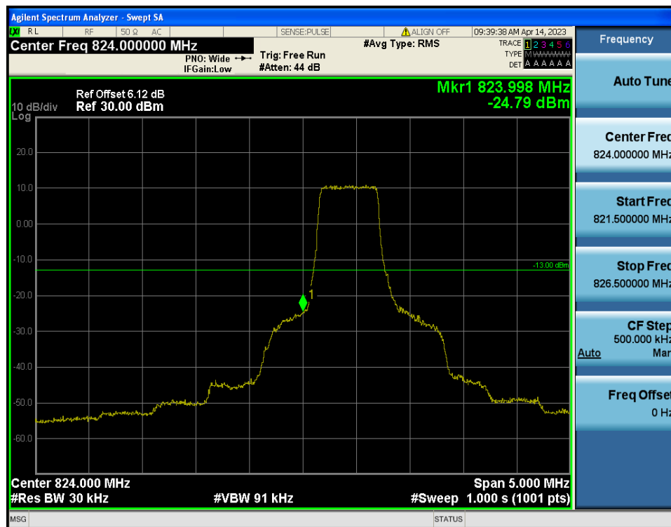
LTE Band 5 / 1.4MHz / 16QAM - RB Size/Offset (3/0)
