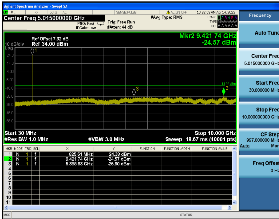
LTE Band 5 / 3MHz / 16QAM - RB Size/Offset (8/4) - Low Channel
