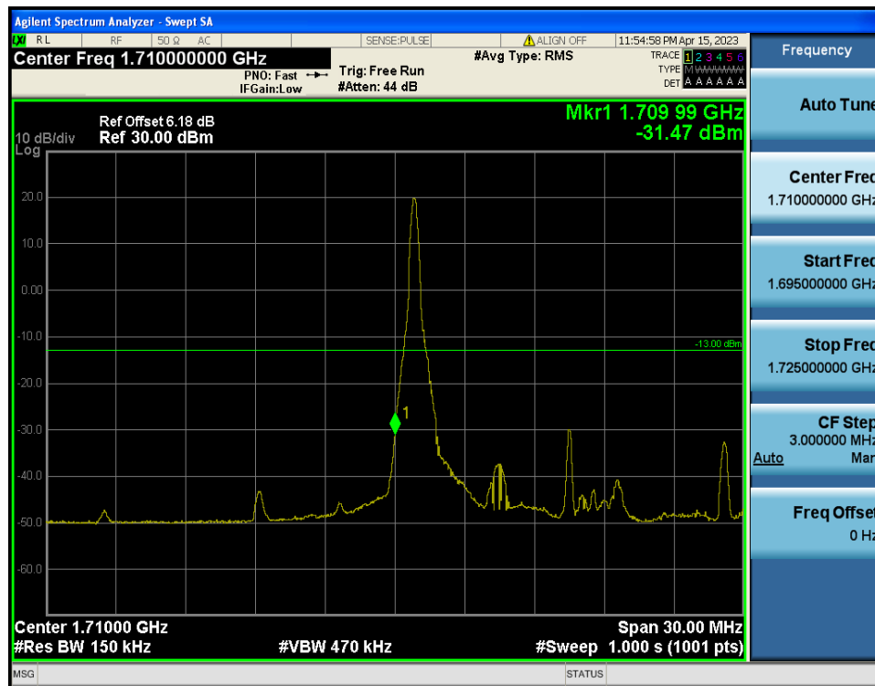
LTE Band 4 / 15MHz / 16QAM - RB Size/Offset (1/0)
