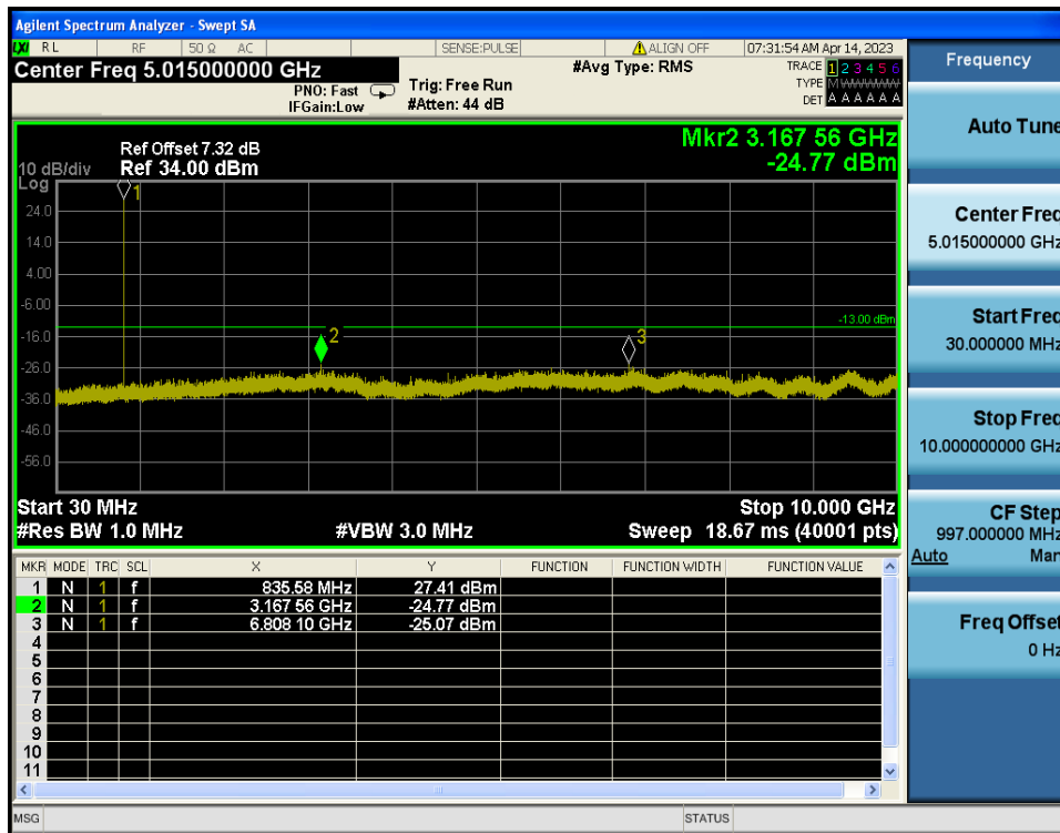
LTE Band 5 / 3MHz / QPSK - RB Size/Offset (1/0) - Mid Channel
