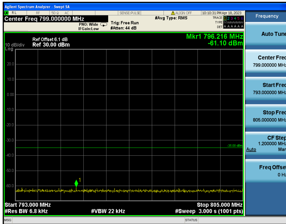
LTE Band 13 / 5MHz / QPSK - RB Size/Offset (1/24)
