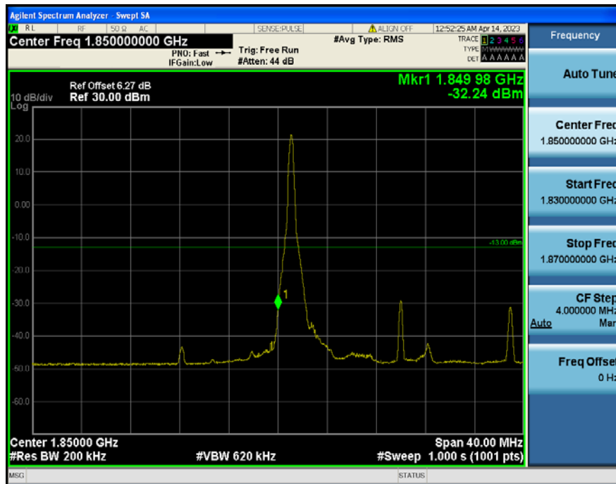
LTE Band 2 / 20MHz / QPSK - RB Size/Offset (1/0)
