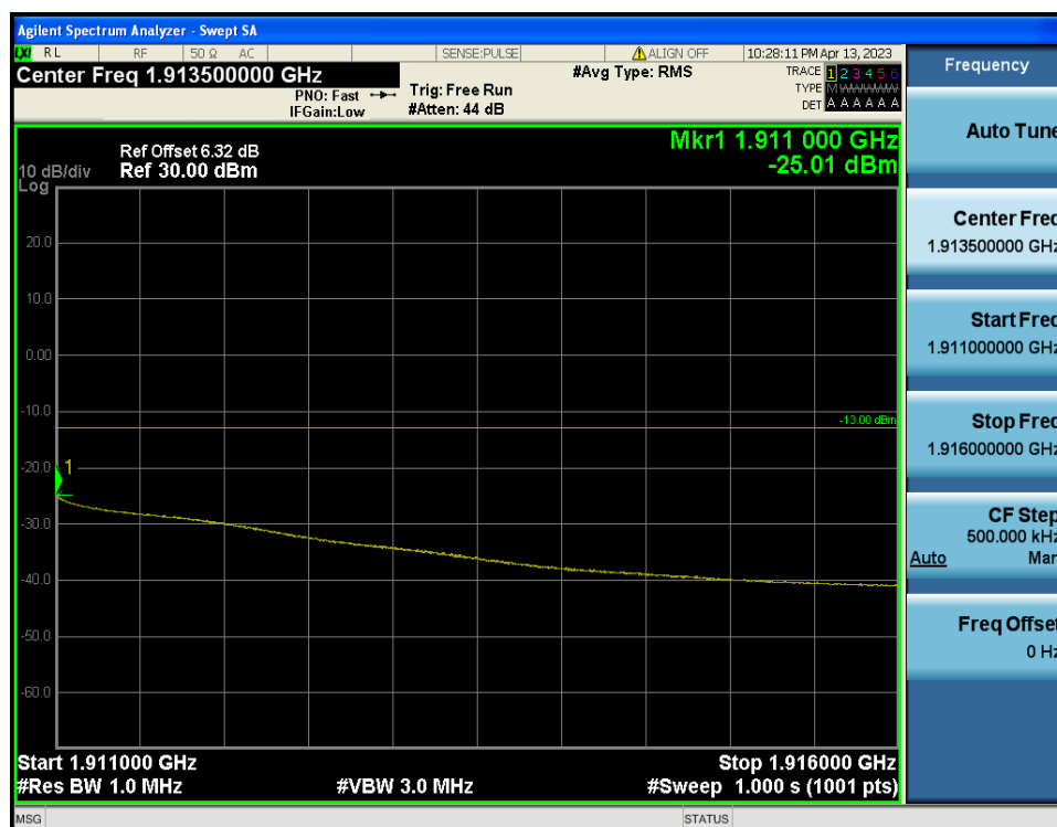
LTE Band 2 / 3MHz / QPSK - RB Size/Offset (8/4)
