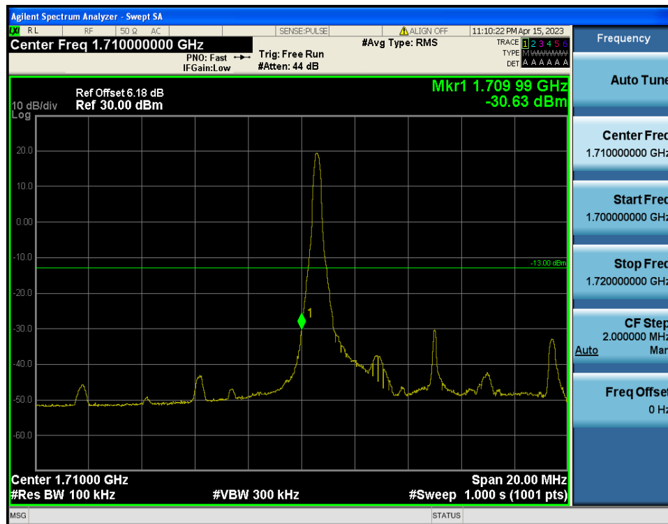
LTE Band 4 / 10MHz / 16QAM - RB Size/Offset (1/0)
