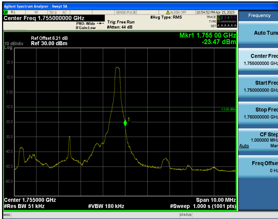
LTE Band 4 / 5MHz / 16QAM - RB Size/Offset (1/24)
