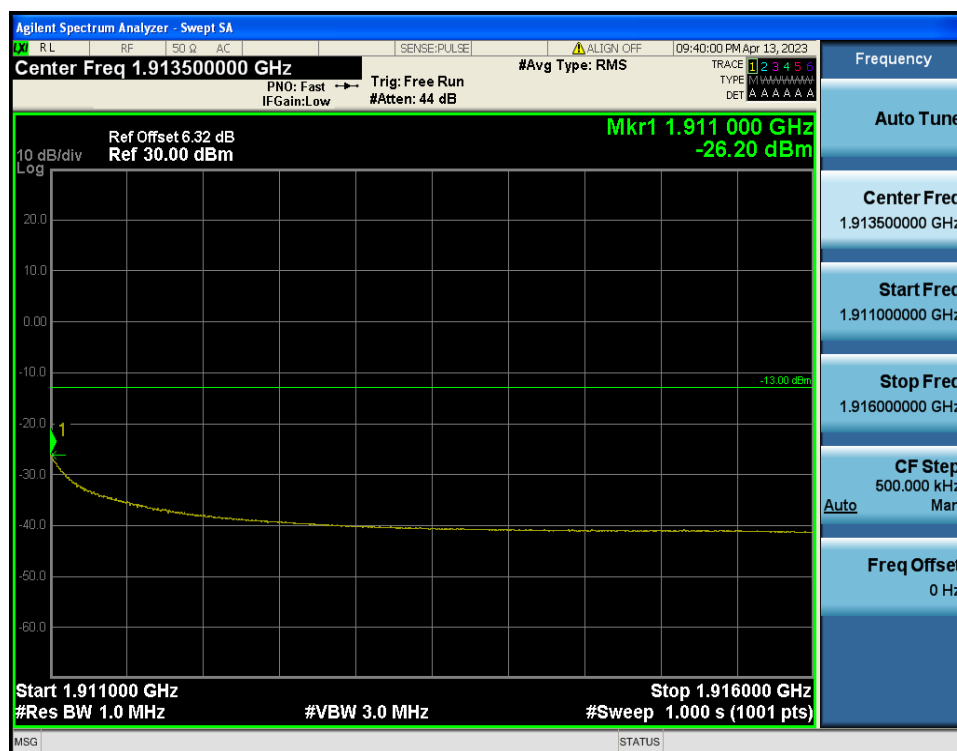
LTE Band 2 / 1.4MHz / QPSK - RB Size/Offset (3/0)
