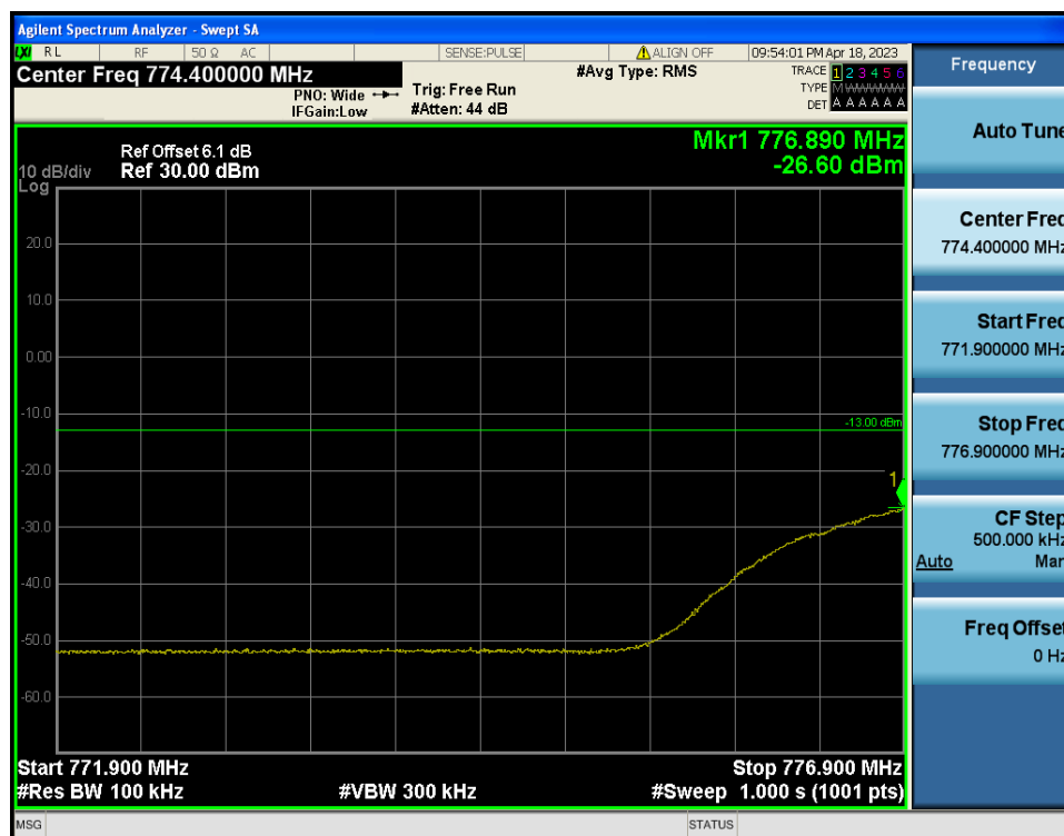
LTE Band 13 / 5MHz / QPSK - RB Size/Offset (12/0)
