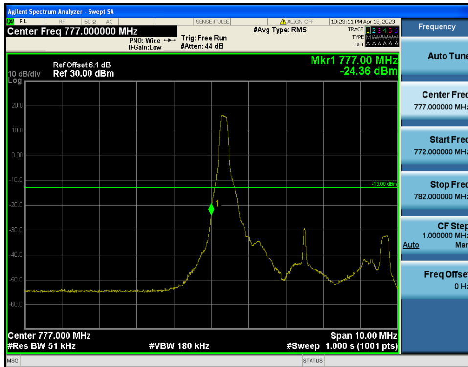
LTE Band 13 / 5MHz / 16QAM - RB Size/Offset (1/0)
