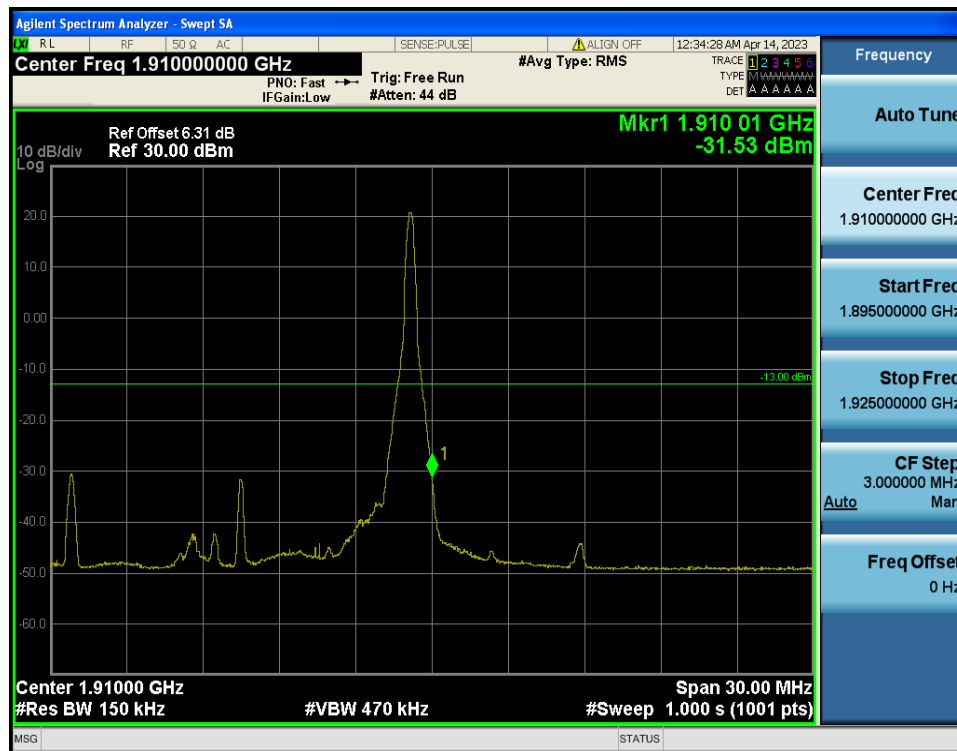
LTE Band 2 / 15MHz / QPSK - RB Size/Offset (1/74)
