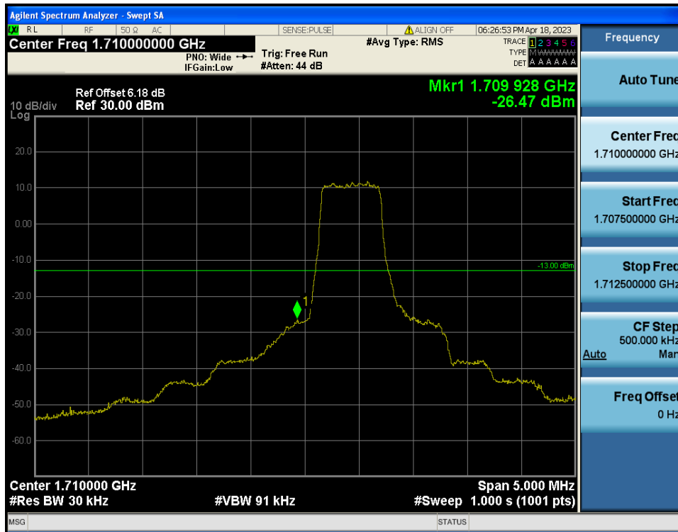
LTE Band 4 / 1.4MHz / QPSK - RB Size/Offset (3/0)
