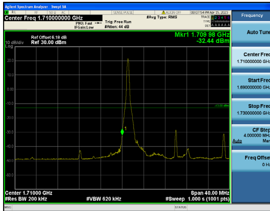
LTE Band 4 / 20MHz / QPSK - RB Size/Offset (1/0)
