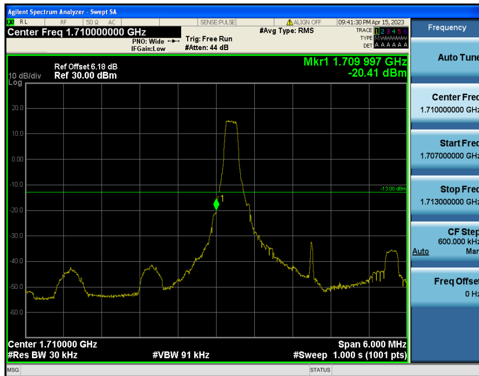
LTE Band 4 / 3MHz / 16QAM - RB Size/Offset (1/0)
