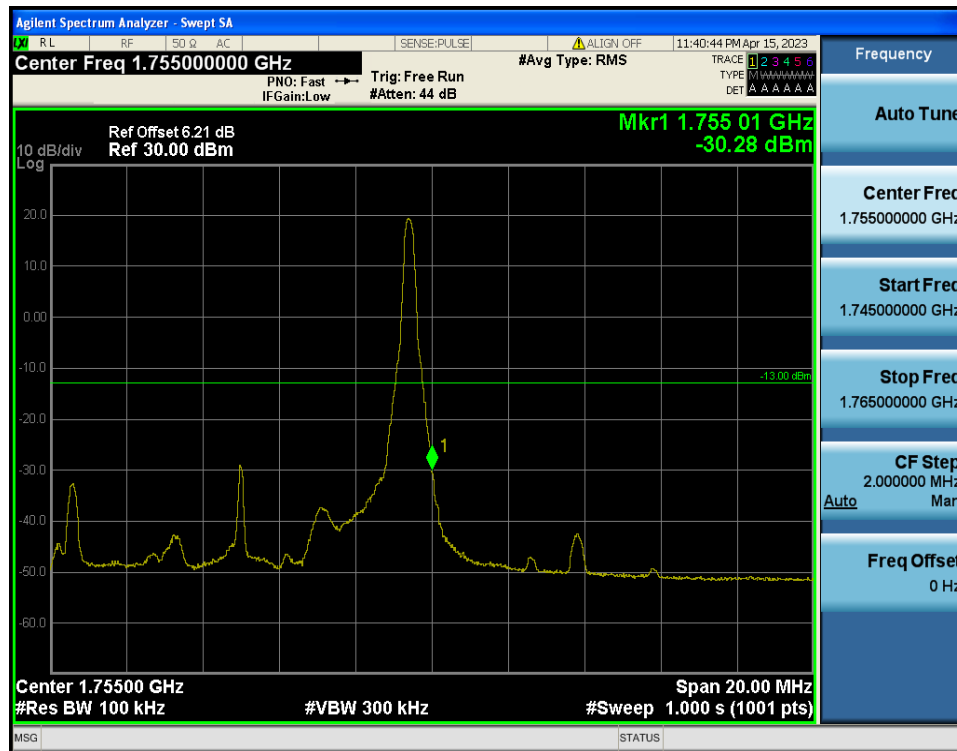
LTE Band 4 / 10MHz / 16QAM - RB Size/Offset (1/49)
