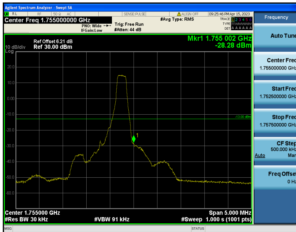
LTE Band 4 / 1.4MHz / 16QAM - RB Size/Offset (1/5)
