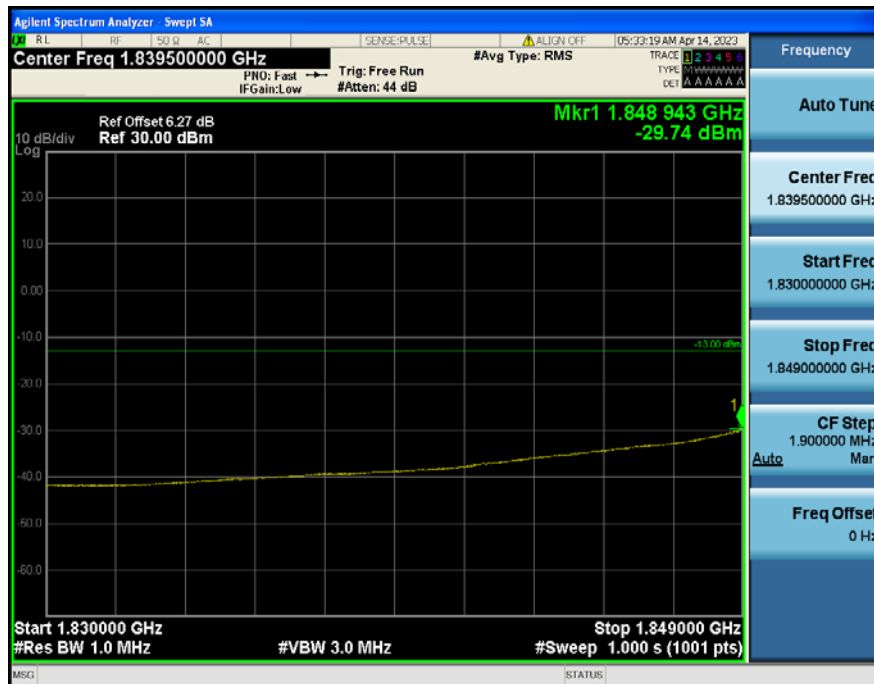
LTE Band 2 / 20MHz / 16QAM - RB Size/Offset (50/0)
