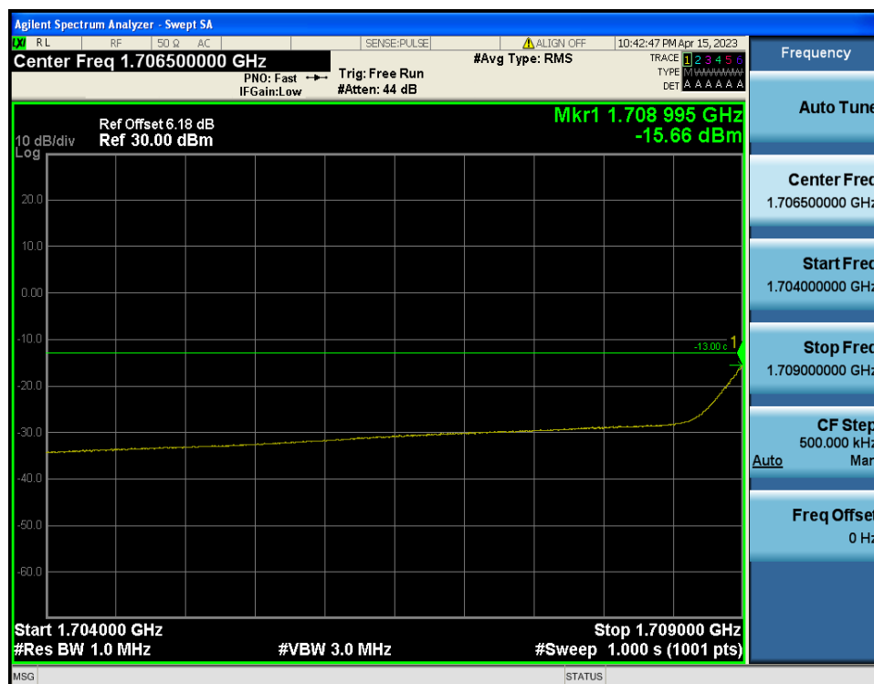
LTE Band 4 / 5MHz / 16QAM - RB Size/Offset (25/0)
