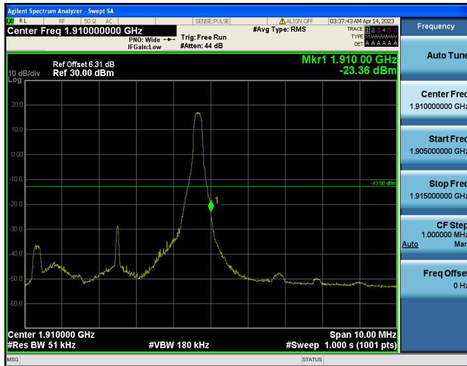
LTE Band 2 / 5MHz / 16QAM - RB Size/Offset (1/24)
