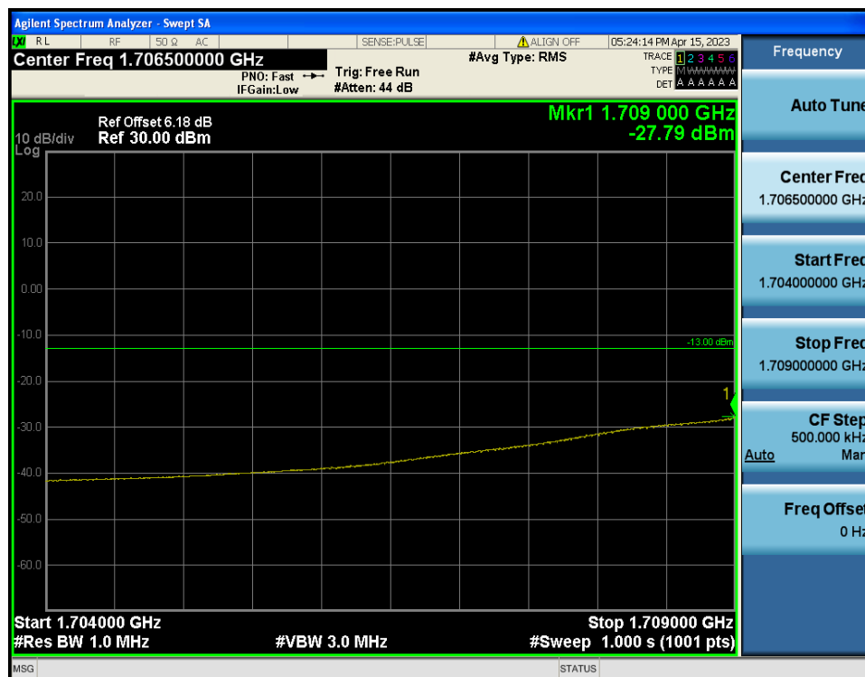
LTE Band 4 / 3MHz / QPSK - RB Size/Offset (8/4)
