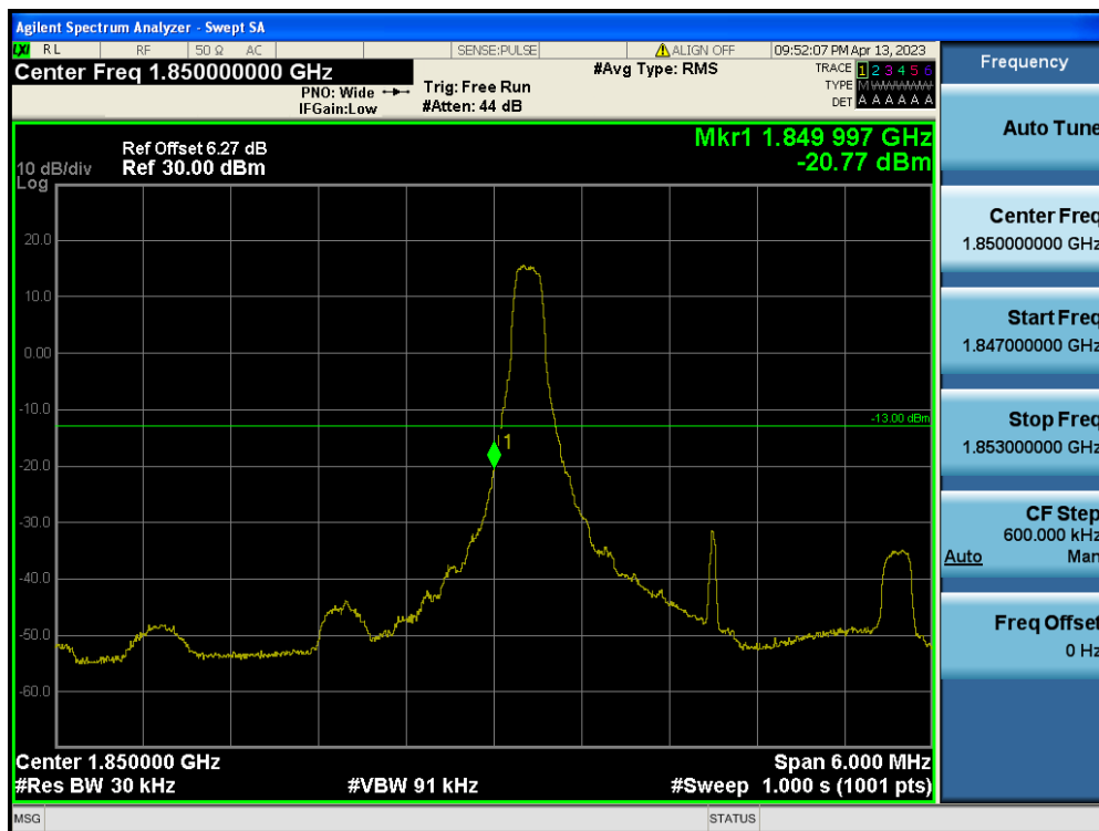
LTE Band 2 / 3MHz / QPSK - RB Size/Offset (1/0)
