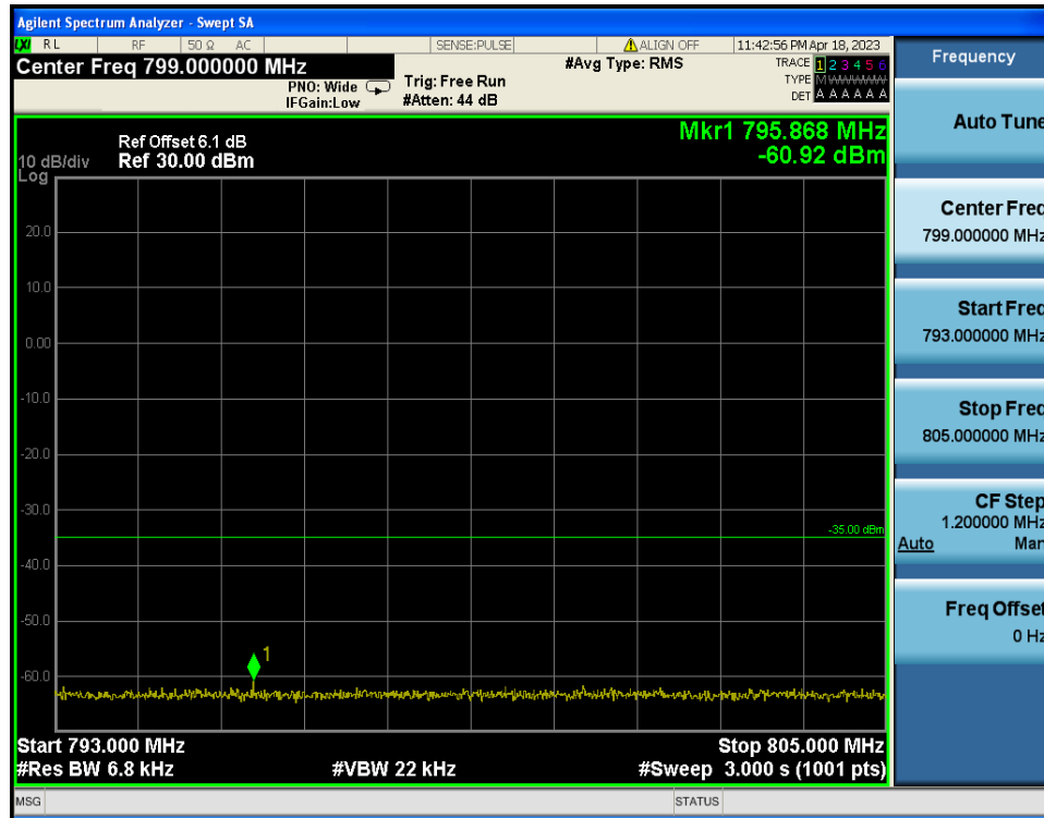
LTE Band 13 / 10MHz / 16QAM - RB Size/Offset (1/25)
