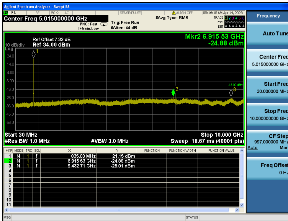
LTE Band 5 / 5MHz / QPSK - RB Size/Offset (25/0) - Mid Channel
