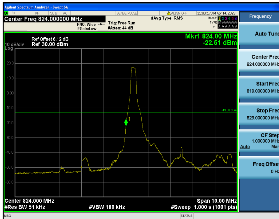
LTE Band 5 / 5MHz / 16QAM - RB Size/Offset (1/0)
