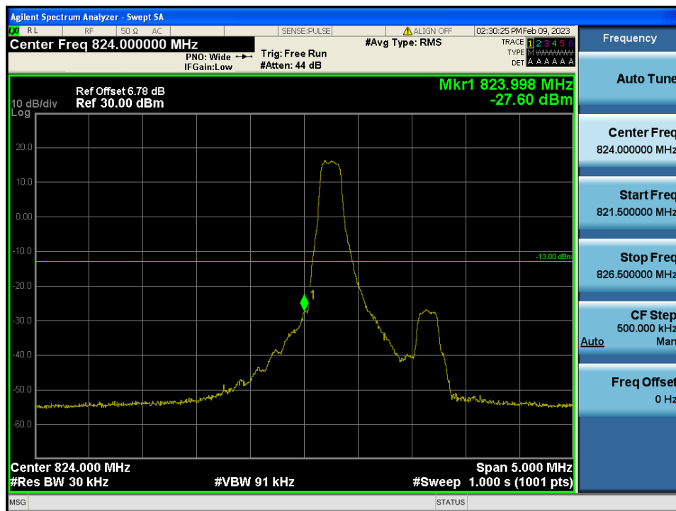
LTE Band 5 / 1.4 MHz / QPSK - RB Size/Offset (1/0)
