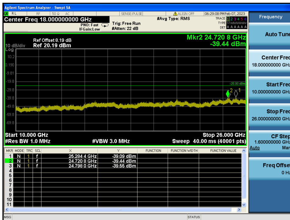
LTE Band 7 / 10 MHz / 16QAM - RB Size/Offset (25/25) – Low Channel
