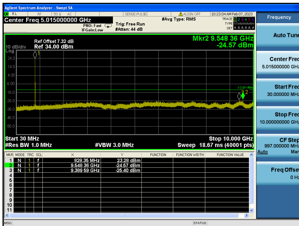
LTE Band 5 / 5 MHz / 16QAM - RB Size/Offset (12/13) – Low Channel
