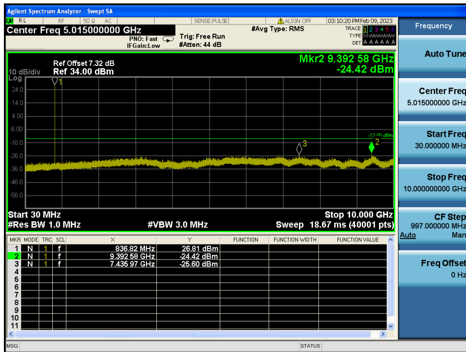
LTE Band 5 / 1.4 MHz / QPSK - RB Size/Offset (3/2) – Mid Channel
