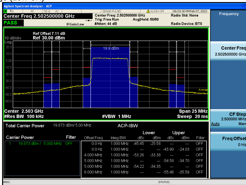
LTE Band 7 / 5 MHz / 16QAM - RB Size/Offset (25/0)
