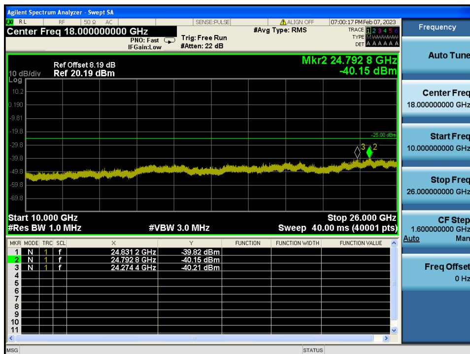
LTE Band 7 / 15 MHz / 16QAM - RB Size/Offset (75/0) – Low Channel
