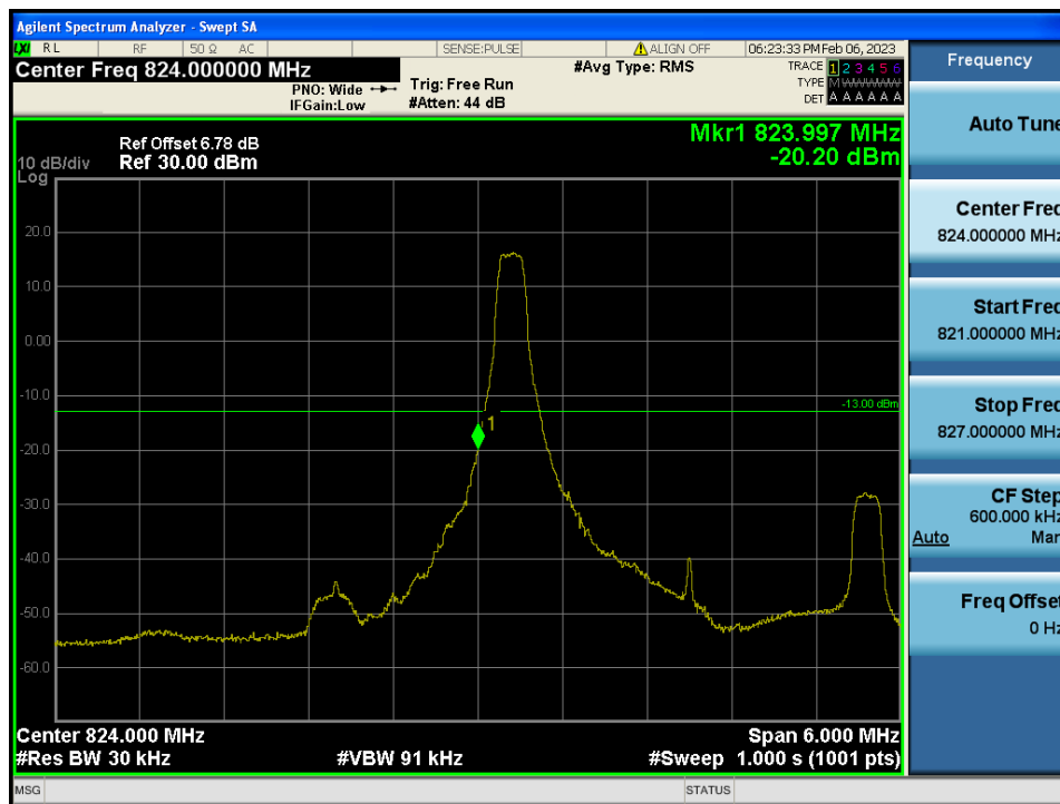
LTE Band 5 / 3 MHz / QPSK- RB Size/Offset (1/0)
