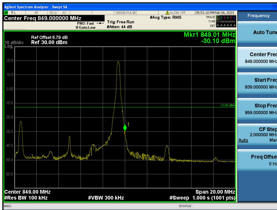
LTE Band 5 / 10 MHz / 16QAM - RB Size/Offset (1/49)
