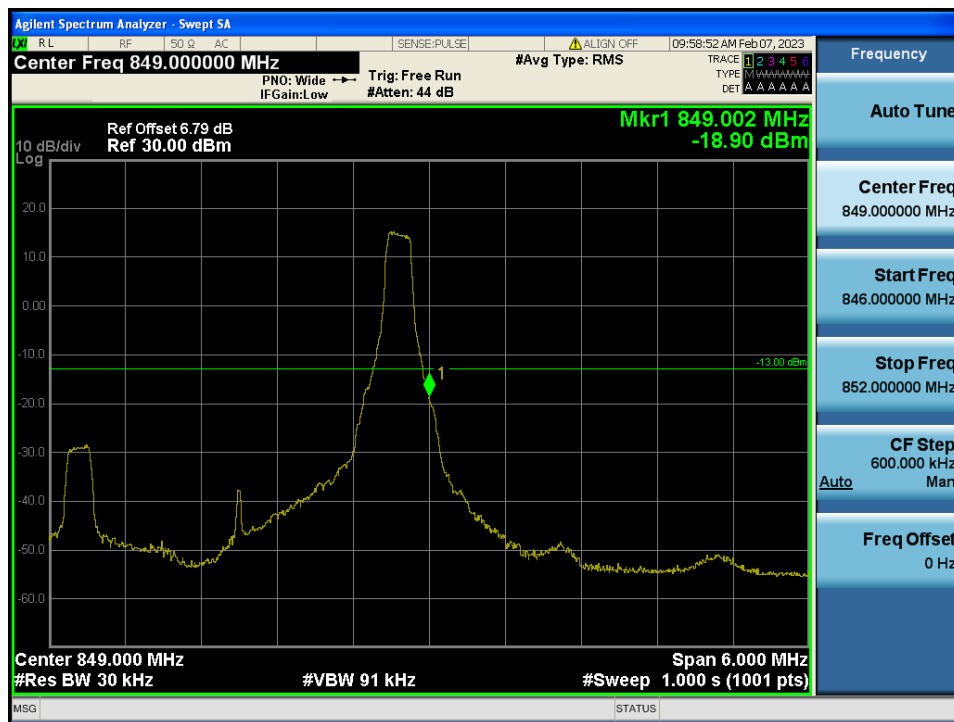
LTE Band 5 / 3 MHz / 16QAM - RB Size/Offset (1/14)
