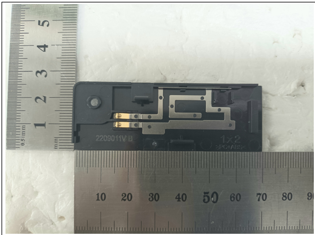
<Internal Antenna 2>
