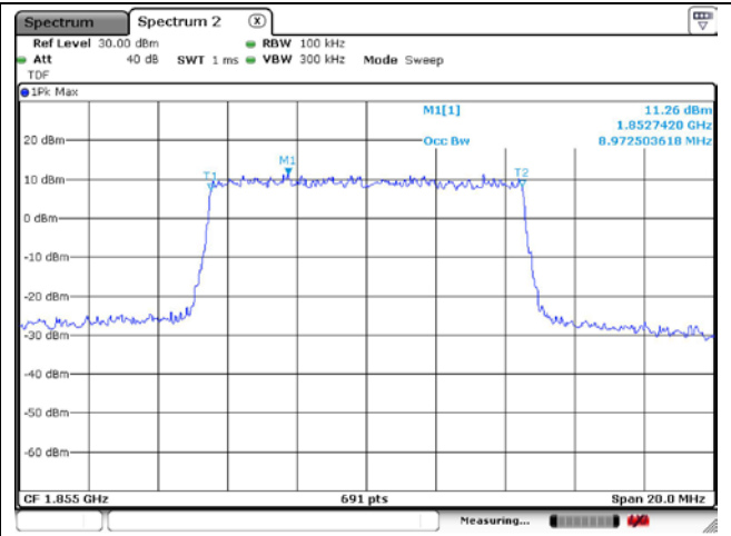
10 MHz 16QAM Low Channel - Full RB
