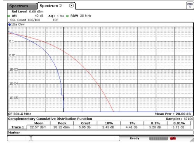
15 MHz Low Channel - Full RB_QPSK
