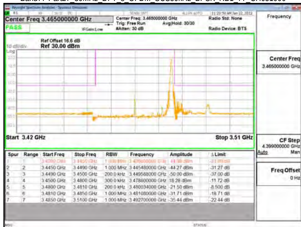
Band77-Part27 30MHz DFT s OFDM SCS30kHz BPSK RB1 77 CH633334
