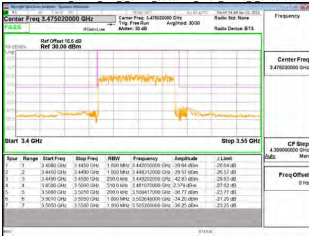
Band77-Part27 50MHz DFT s OFDM SCS30kHz BPSK RB128 0 CH633334
