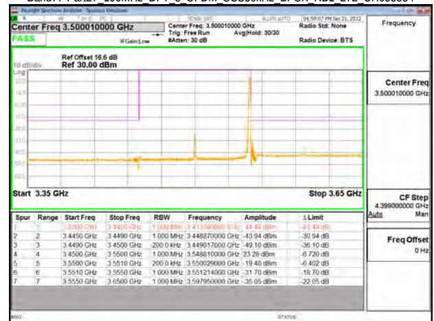
Band77-Part27 100MHz DFT s OFDM SCS30kHz BPSK RB1 272 CH633334
