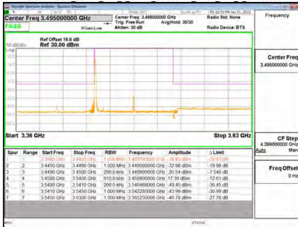
Band77-Part27 90MHz DFT s OFDM SCS30kHz BPSK RB1 0 CH633334
