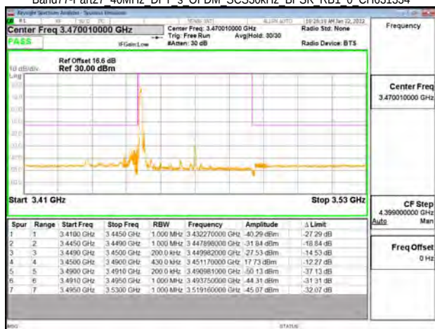
Band77-Part27 40MHz DFT s OFDM SCS30kHz BPSK RB1 0 CH633334
