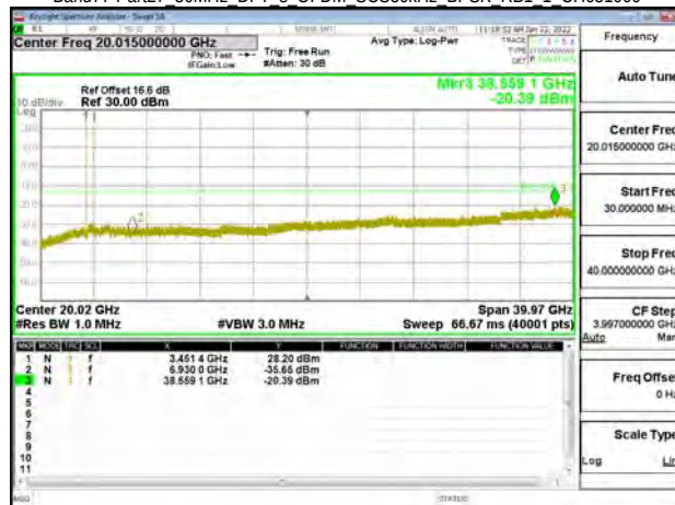
Band77-Part27 30MHz DFT s OFDM SCS30kHz BPSK RB1 1 CH633334
