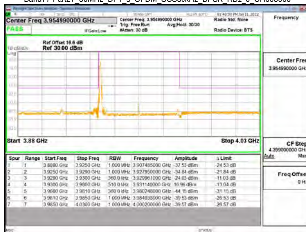
Band77-Part27 50MHz DFT s OFDM SCS30kHz BPSK RB1 0 CH663666
