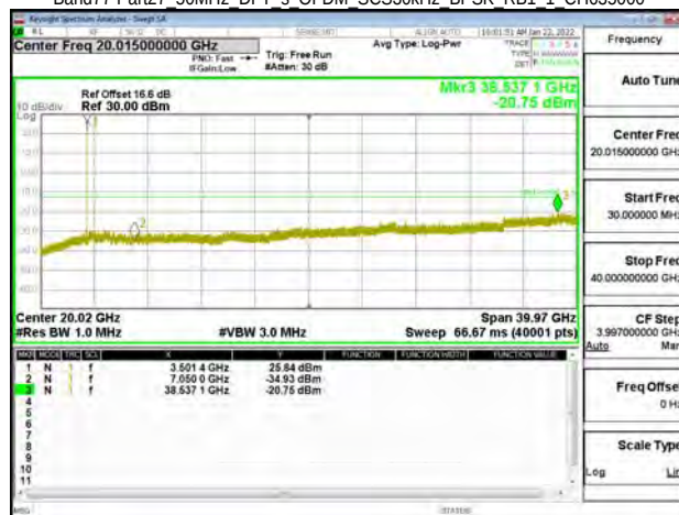
Band77-Part27 50MHz DFT s OFDM SCS30kHz BPSK RB1 1 CH635000
