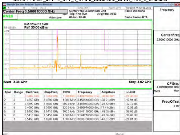
Band77-Part27 80MHz DFT s OFDM SCS30kHz BPSK RB1 0 CH634000
