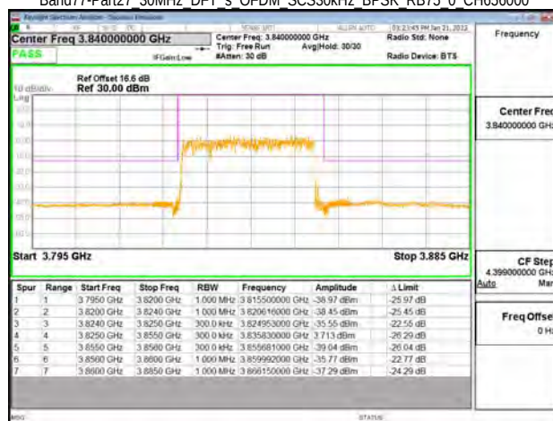
Band77-Part27 30MHz DFT s OFDM SCS30kHz BPSK RB75 0 CH656000
