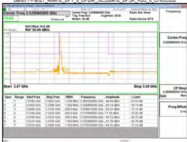
Band77-Part27 40MHz DFT s OFDM SCS30kHz BPSK RB1 0 CH635332
