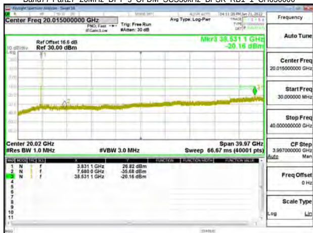
Band77-Part27 20MHz DFT s OFDM SCS30kHz BPSK RB1 1 CH664666
