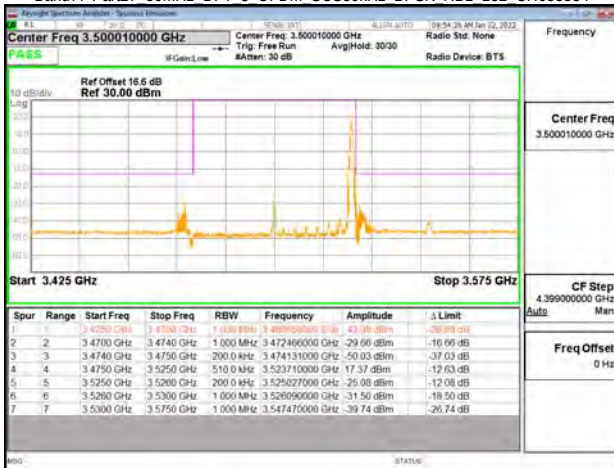
Band77-Part27 50MHz DFT s OFDM SCS30kHz BPSK RB1 132 CH635000
