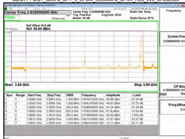
Band77-Part27 80MHz DFT s OFDM SCS30kHz BPSK RB1 216 CH626666
