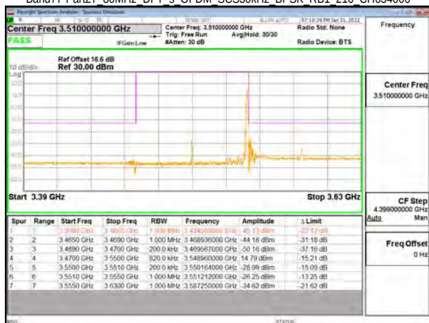
Band77-Part27 80MHz DFT s OFDM SCS30kHz BPSK RB1 216 CH634000
