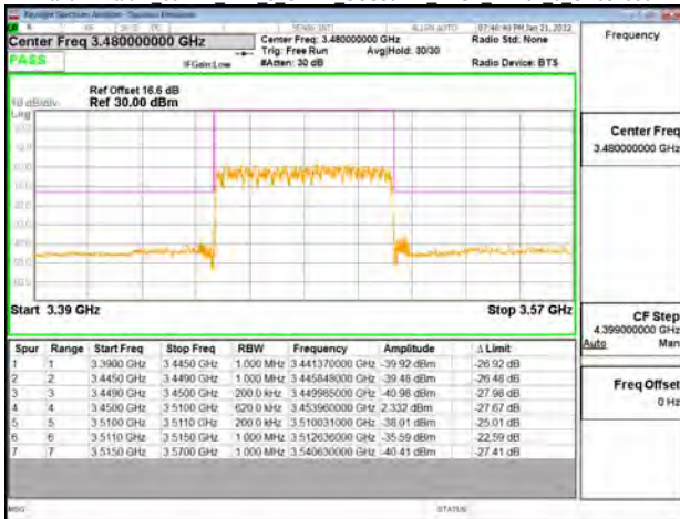
Band77-Part27 60MHz DFT s OFDM SCS30kHz BPSK RB162 0 CH633334
