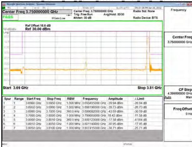
Band77-Part27 100MHz DFT s OFDM SCS30kHz BPSK RB1 272 CH656000
