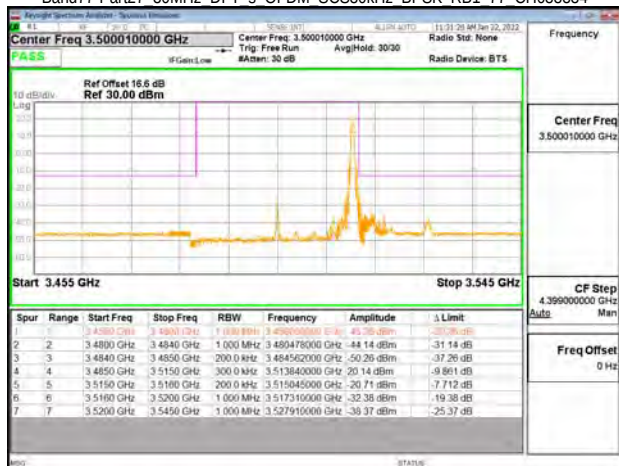
Band77-Part27 30MHz DFT s OFDM SCS30kHz BPSK RB1 77 CH635666
