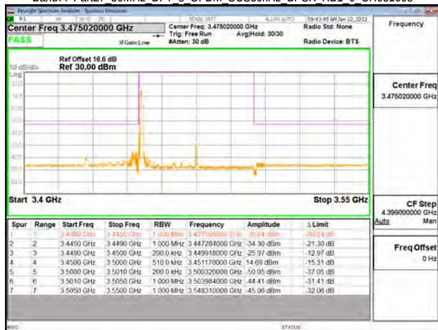
Band77-Part27 50MHz DFT s OFDM SCS30kHz BPSK RB1 0 CH633334
