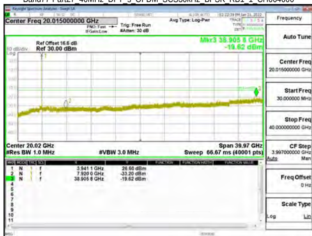
Band77-Part27 40MHz DFT s OFDM SCS30kHz BPSK RB1 1 CH664000
