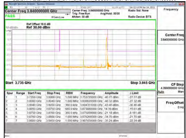
Band77-Part27 70MHz DFT s OFDM SCS30kHz BPSK RB1 188 CH636000
