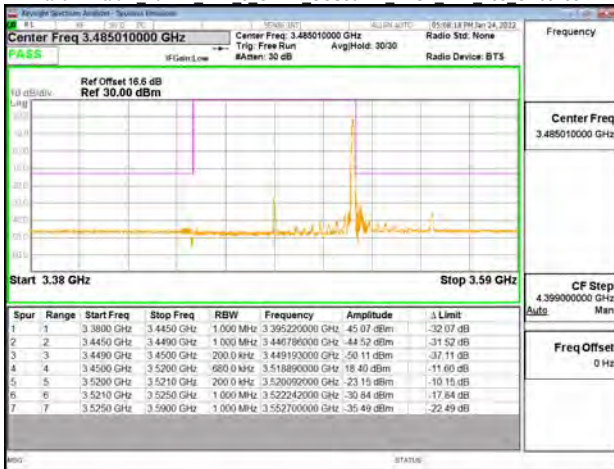
Band77-Part27 70MHz DFT s OFDM SCS30kHz BPSK RB1 188 CH633334
