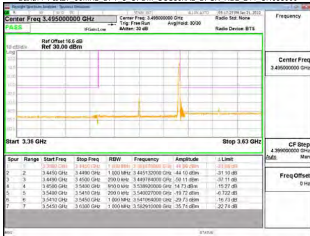
Band77-Part27 90MHz DFT s OFDM SCS30kHz BPSK RB1 244 CH633334
