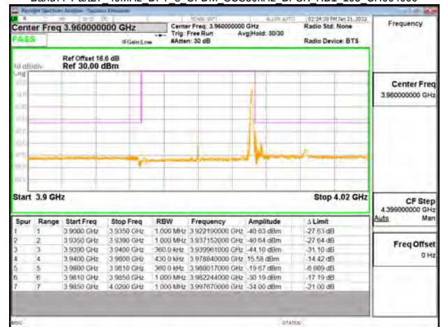
Band77-Part27 40MHz DFT s OFDM SCS30kHz BPSK RB1_105 CH664000
