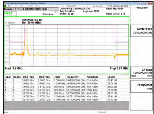
Band77-Part27 60MHz DFT s OFDM SCS30kHz BPSK RB1 0 CH663332
