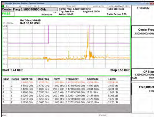
Band77-Part27 40MHz DFT s OFDM SCS30kHz BPSK RB1_105 CH635332
