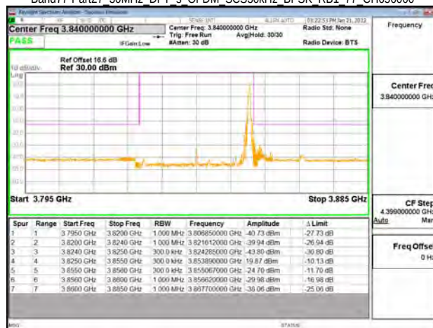
Band77-Part27 30MHz DFT s OFDM SCS30kHz BPSK RB1 77 CH656000
