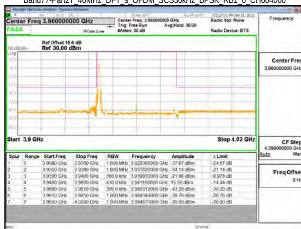
Band77-Part27 40MHz DFT s OFDM SCS30kHz BPSK RB1 0 CH664000
