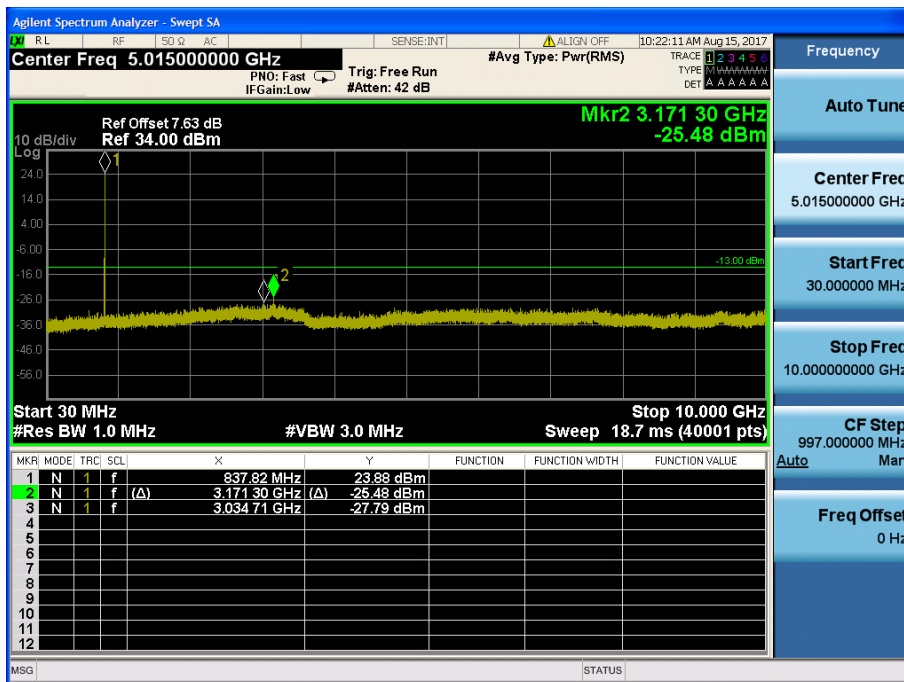
LTE Band 5 / 5MHz / 16QAM - RB Size/Offset (12/13) – Mid Channel
