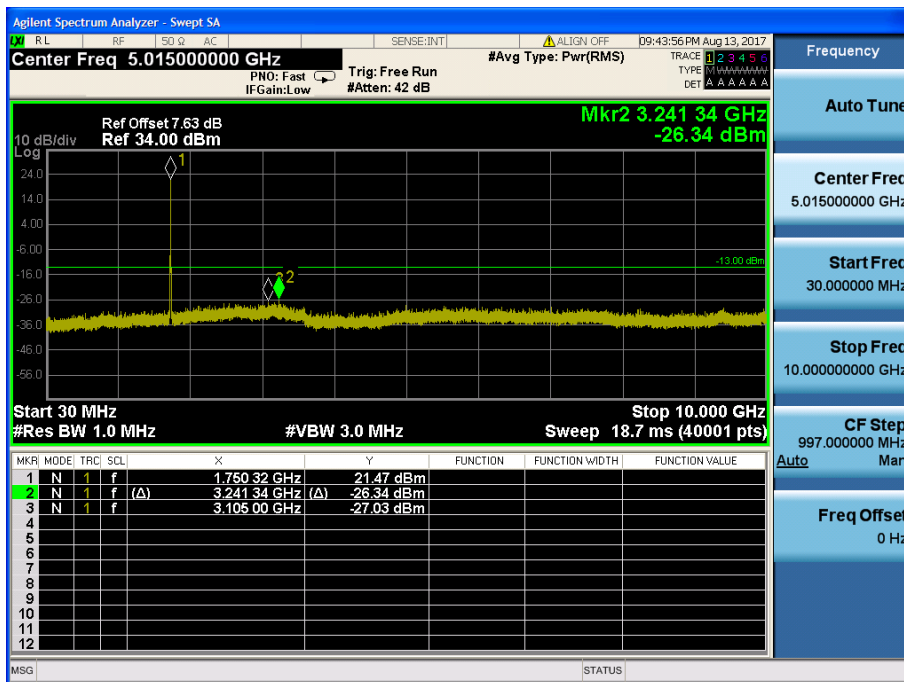
LTE Band 4 / 15MHz / QPSK - RB Size/Offset (36/19) – High Channel
