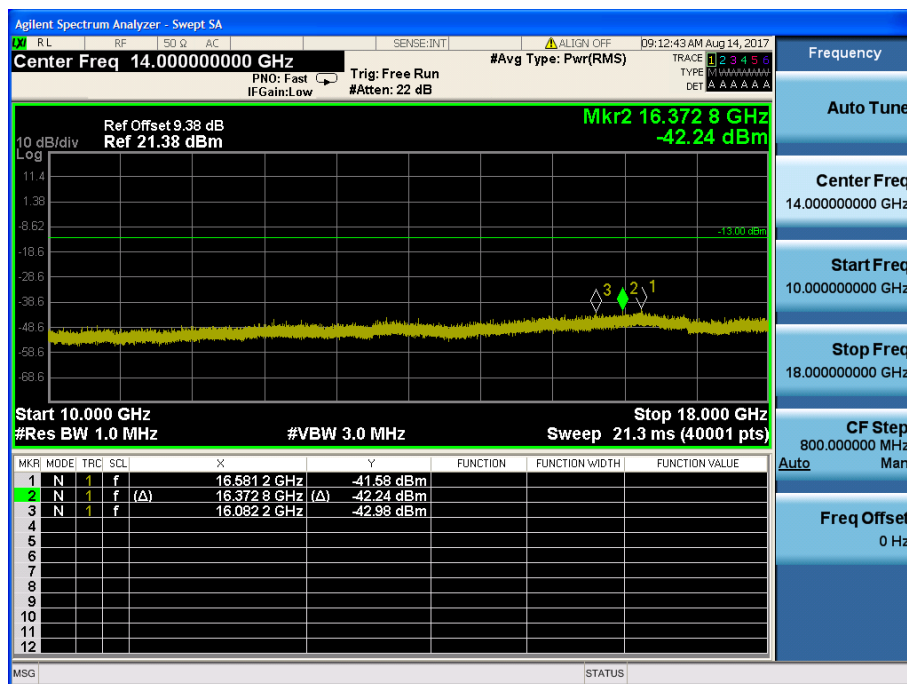
LTE Band 4 / 20MHz / QPSK - RB Size/Offset (50/50) –Low Channel
