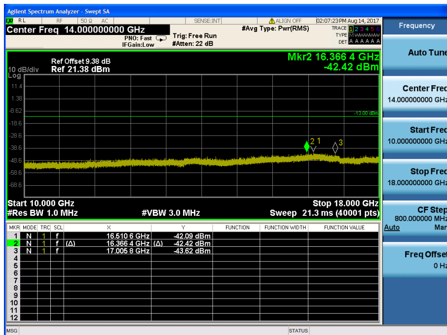
LTE Band 4 / 10MHz / 16QAM - RB Size/Offset (25/0) – High Channel
