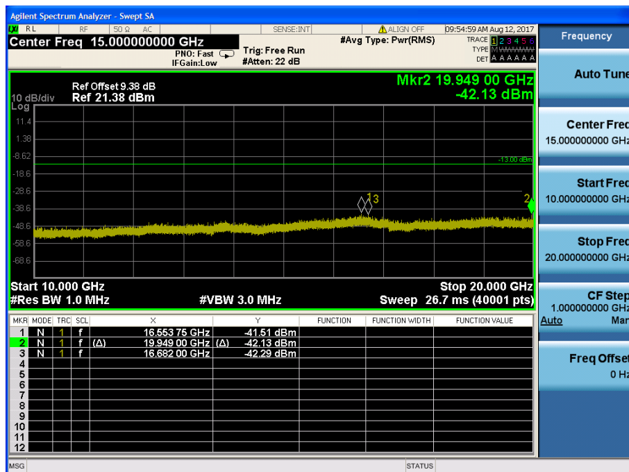
LTE Band 2 / 1.4MHz / 16QAM - RB Size/Offset (1/3) – Low Channel
