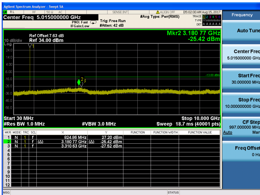
LTE Band 5 / 1.4MHz / 16QAM - RB Size/Offset (3/1) – Low Channel
