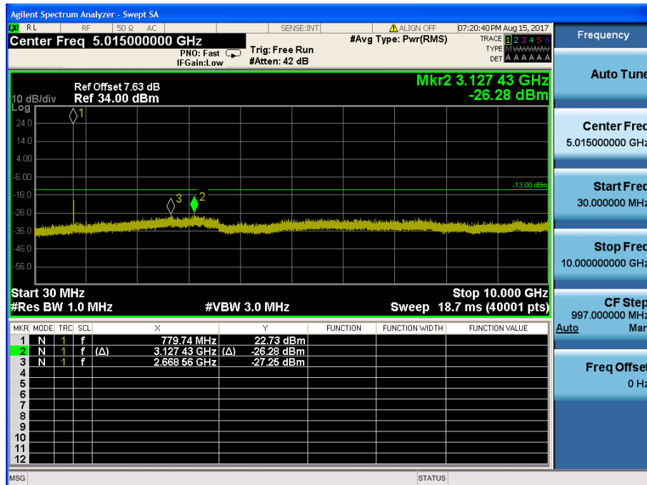
LTE Band 13 / 5MHz / 16QAM - RB Size/Offset (25/0) – Low Channel
