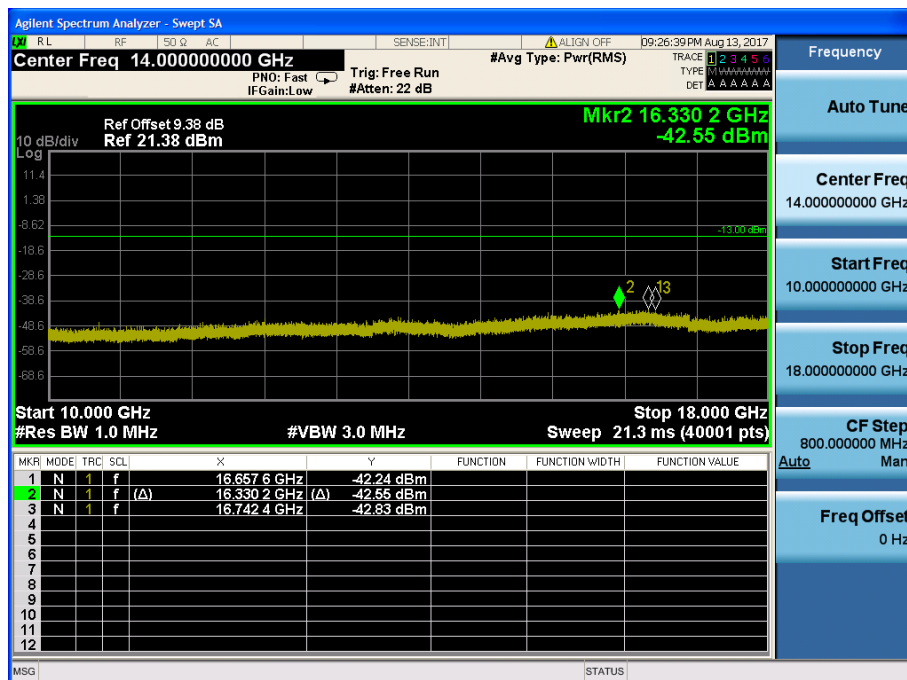
LTE Band 4 / 15MHz / QPSK - RB Size/Offset (1/37) – Mid Channel
