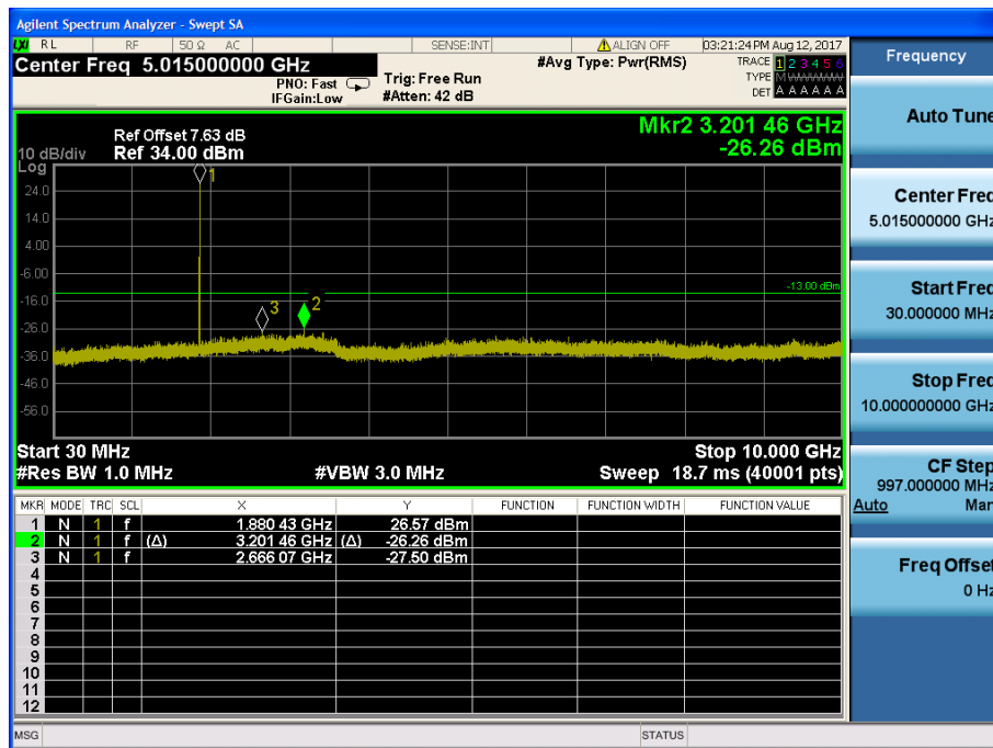
LTE Band 2 / 15MHz / 16QAM - RB Size/Offset (1/37) – Mid Channel
