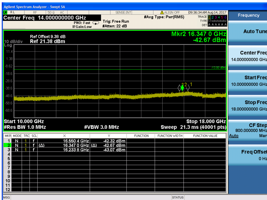
LTE Band 4 / 20MHz / QPSK - RB Size/Offset (50/25) – High Channel
