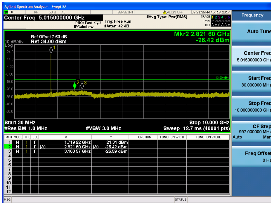
LTE Band 4 / 15MHz / QPSK - RB Size/Offset (36/39)–Low Channel
