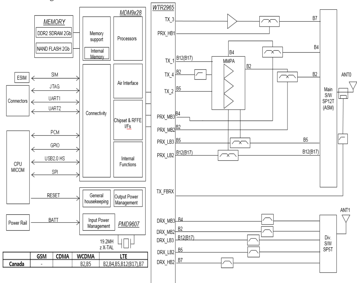
Figure 1.1. TM13LNCAHK1 Block diagram
