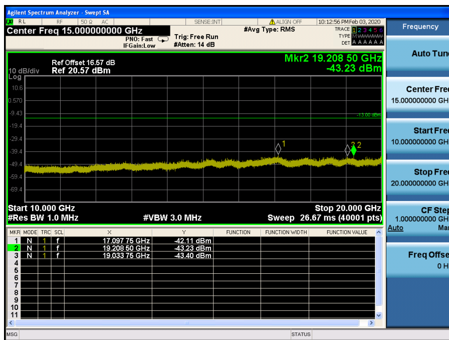
LTE Band 2 / 1.4MHz / 16QAM - RB Size/Offset (1/5) – Mid Channel
