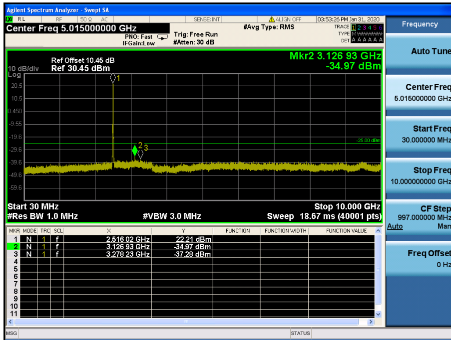
LTE Band 7 / 20MHz / 16QAM - RB Size/Offset (50/50) –Low Channel
