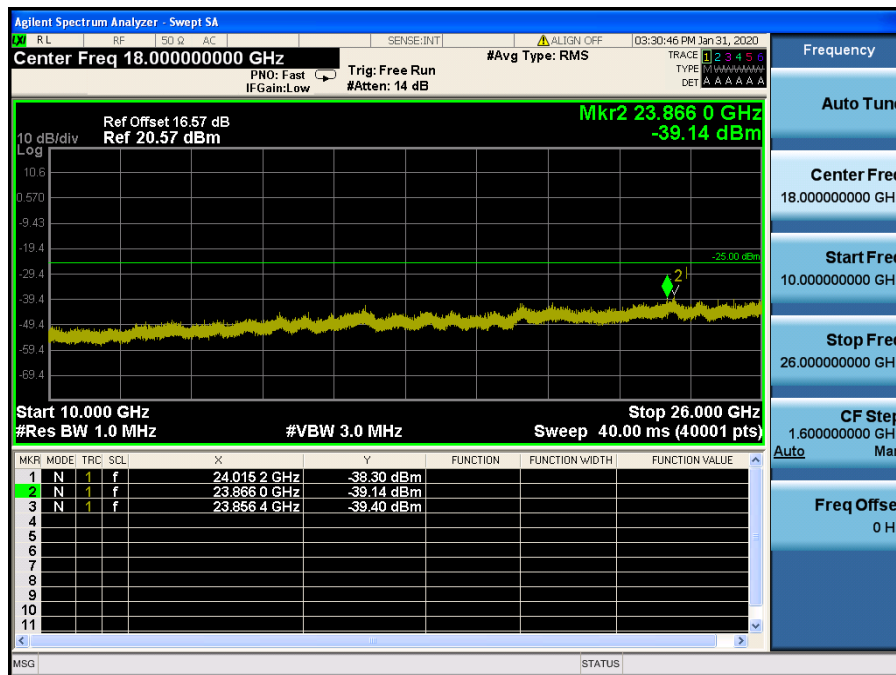
LTE Band 7 / 15MHz / 16QAM - RB Size/Offset (1/36) – High Channel
