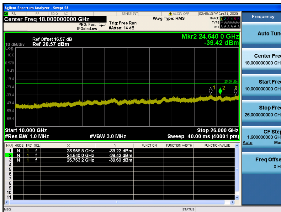
LTE Band 7 / 10MHz / 16QAM - RB Size/Offset (1/25) – High Channel
