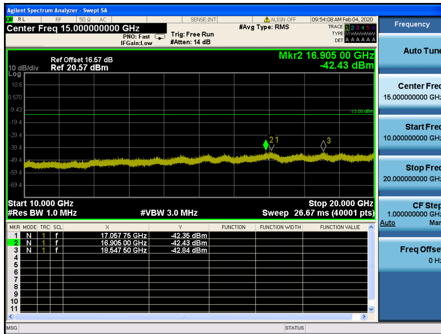
LTE Band 4 / 5MHz / 16QAM - RB Size/Offset (12/13) – Low Channel
