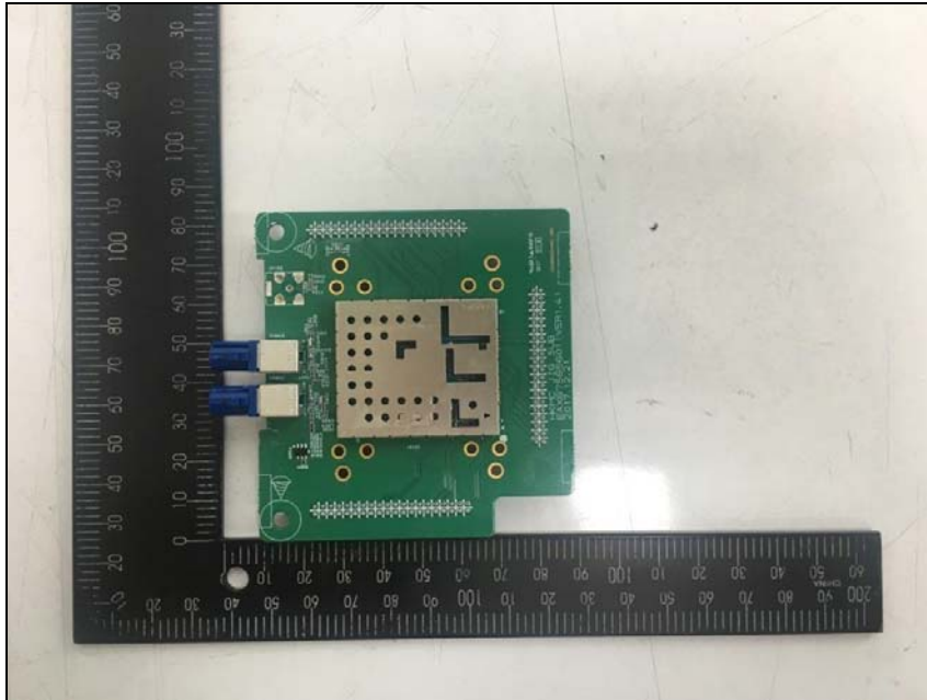
Top view of Module
