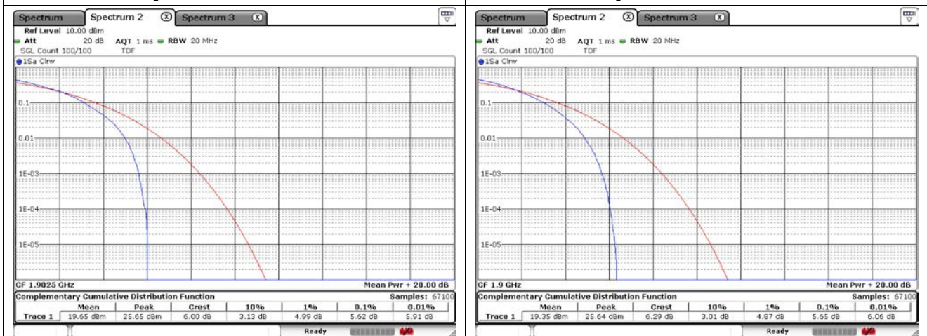
15 MHz 16QAM High Channel - Full RB
