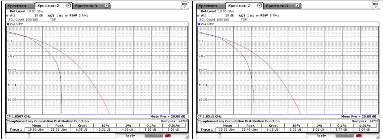
1.4 MHz 16QAM Low Channel - Full RB
