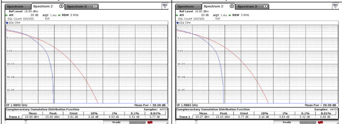
1.4 MHz 16QAM High Channel - Full RB
