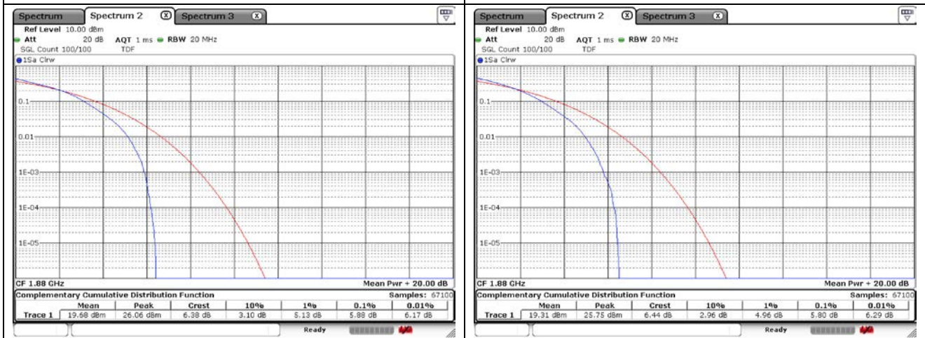
15 MHz 16QAM Middle Channel - Full RB
