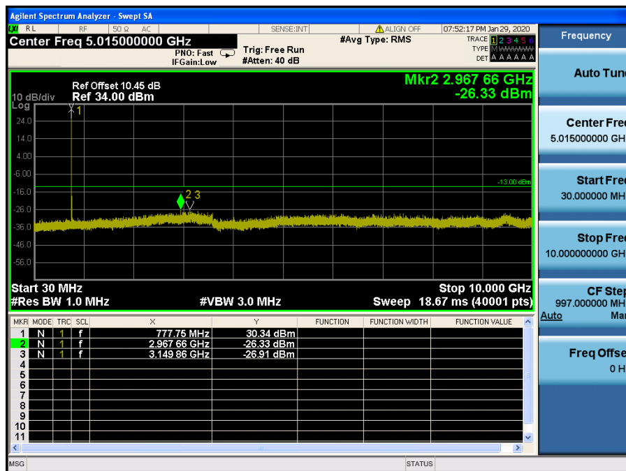
LTE Band 13 / 10MHz / QPSK - RB Size/Offset (1/0) – Low Channel
