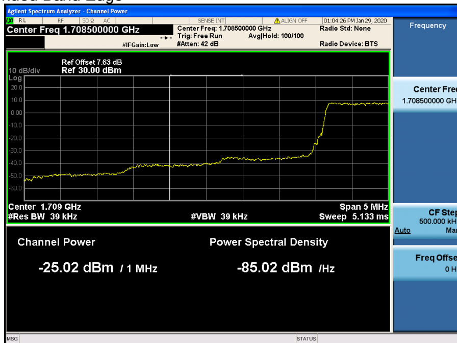
LTE Band 4 / 3MHz / QPSK - RB Size/Offset (8/0)
