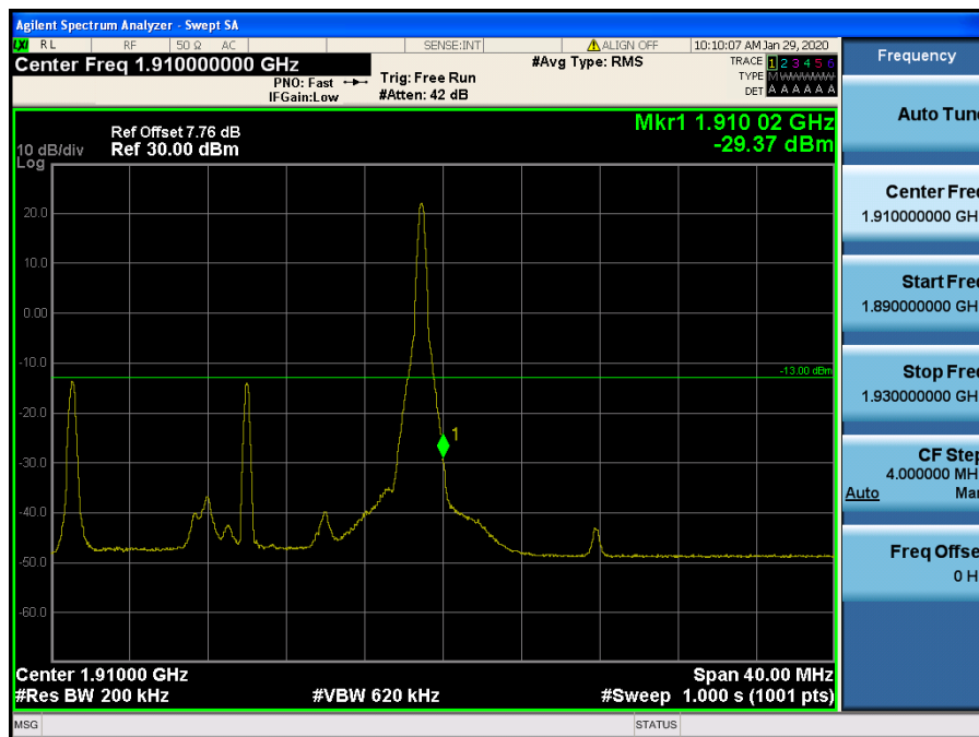
LTE Band 2 / 2MHz / 16QAM - RB Size/Offset (1/99)
