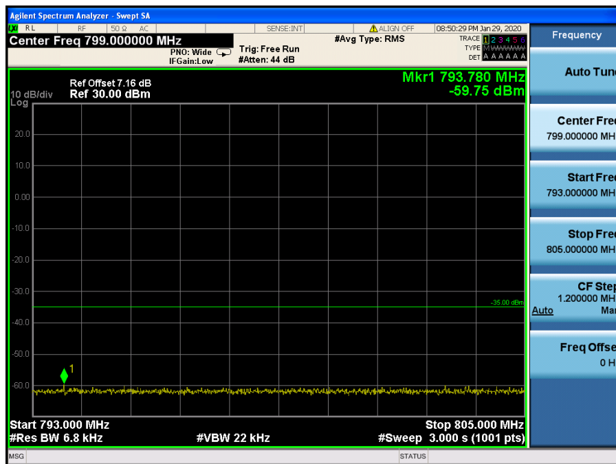
LTE Band 13 / 5MHz / 16QAM - RB Size/Offset (1/12)
