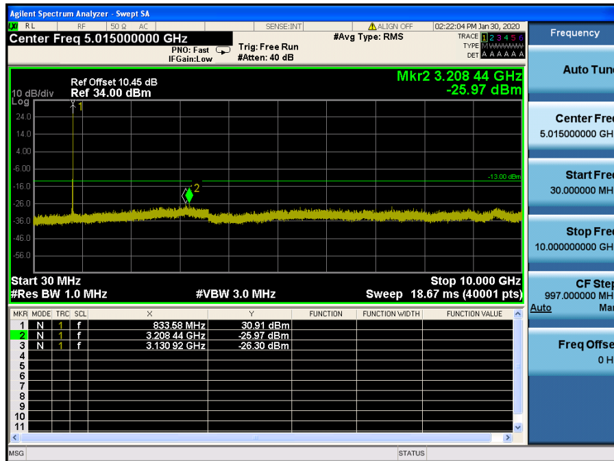
LTE Band 5 / 10MHz / 16QAM - RB Size/Offset (1/49) – Low Channel
