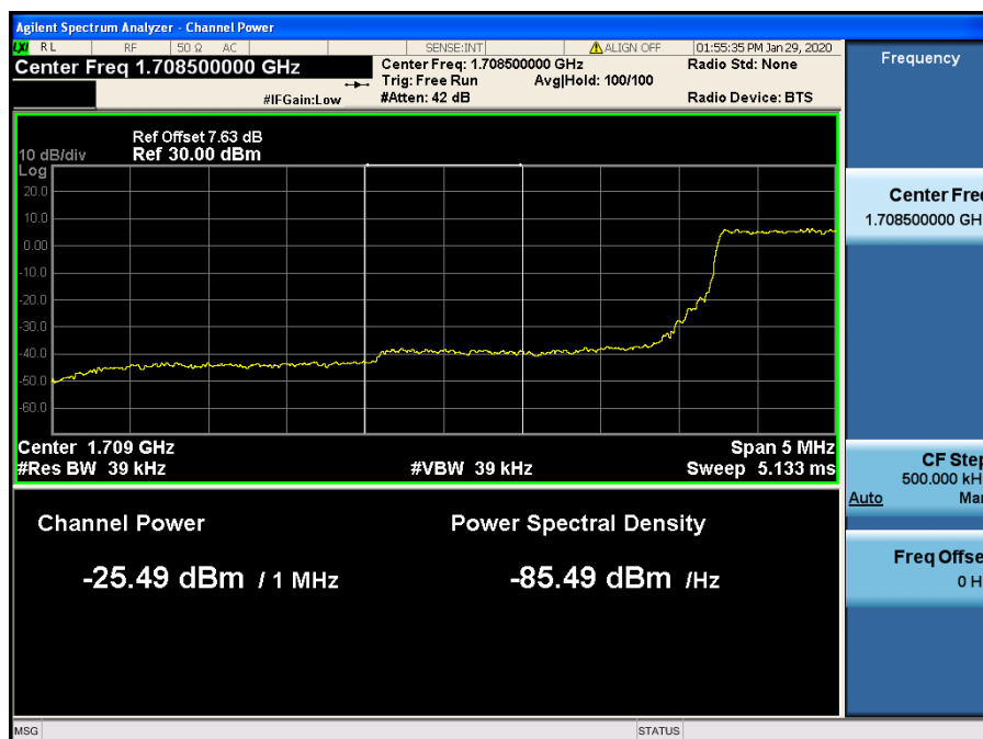
LTE Band 4 / 5MHz / QPSK - RB Size/Offset (12/0)
