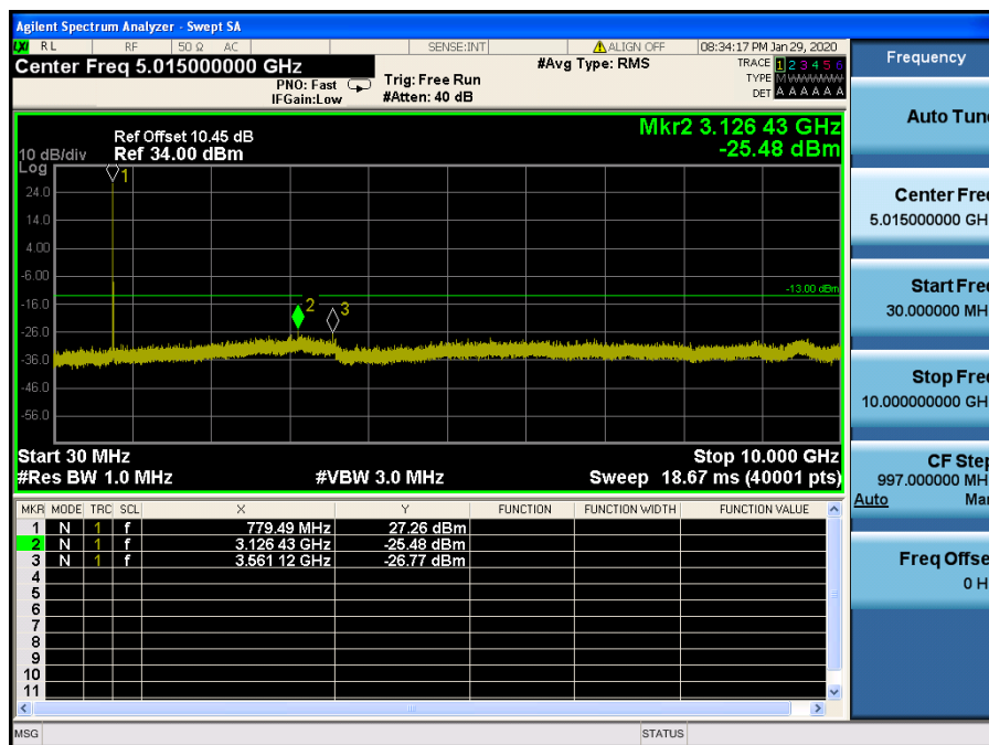
LTE Band 13 / 5MHz / 16QAM - RB Size/Offset (12/0) – Low Channel
