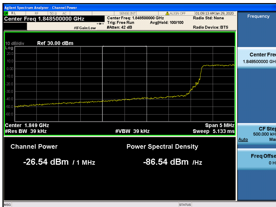
LTE Band 2 / 5MHz / 16QAM - RB Size/Offset (12/0)
