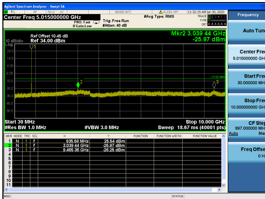
LTE Band 5 / 10MHz / QPSK - RB Size/Offset (25/0) – Mid Channel
