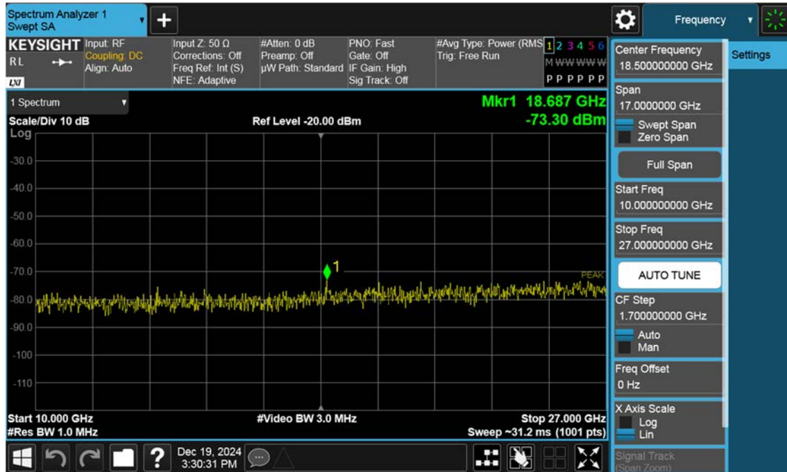
LTE B41_15 M_Conducted Spurious(Above10 G)_Low_QPSK_1RB
