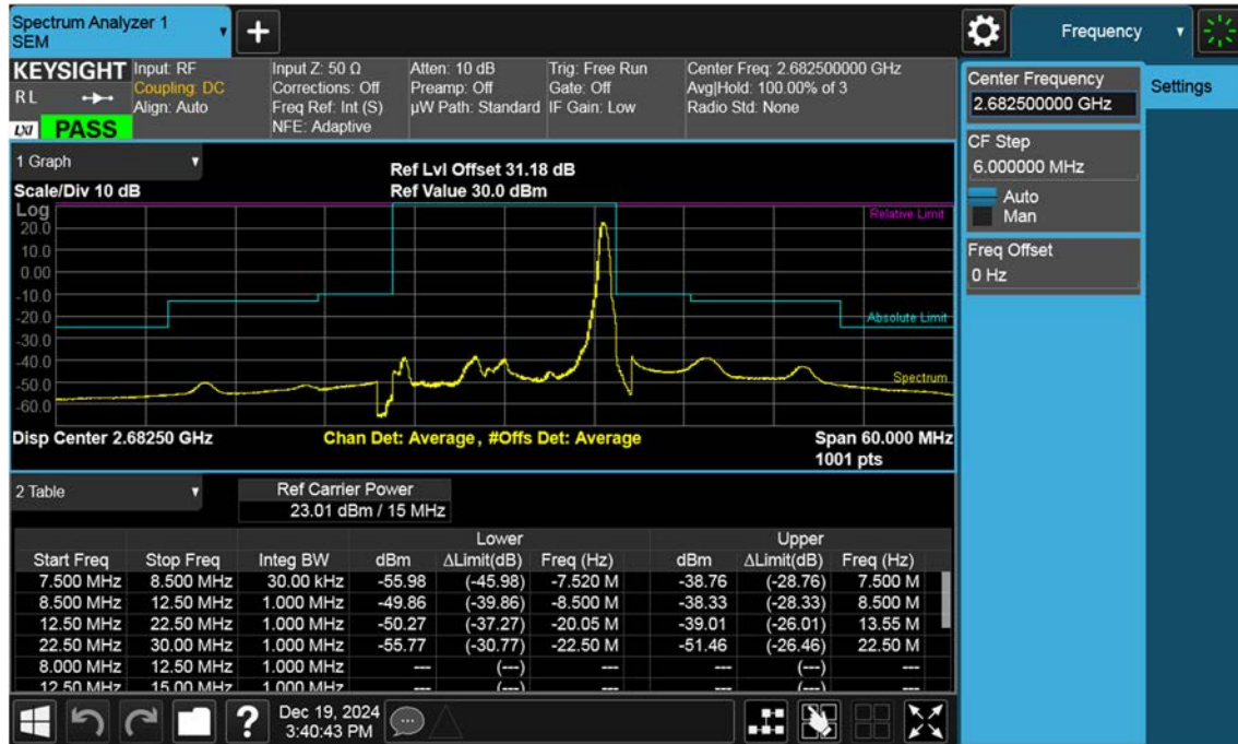
LTE B41_15 M_Channel Edge_High_QPSK_1RB
