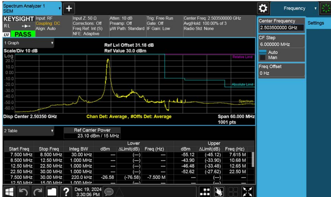
LTE B41_15 M_Channel Edge_Upper_Low_QPSK_1RB
