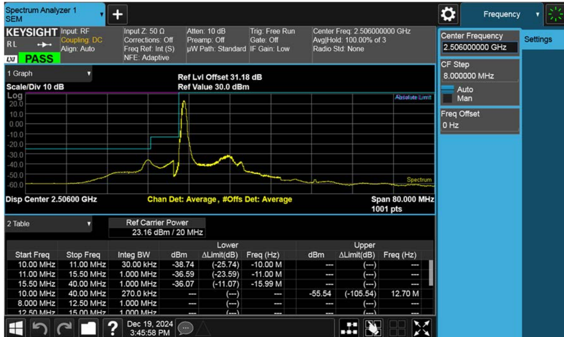
LTE B41_20 M_Channel Edge_Lower_Low_QPSK_1RB
