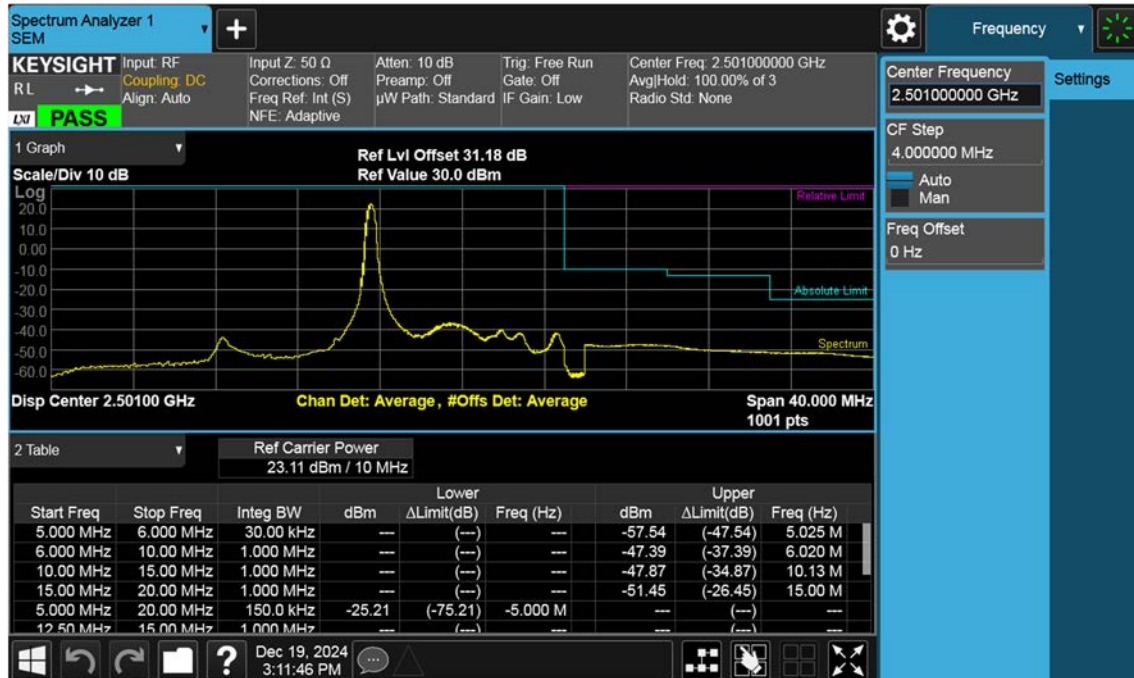
LTE B41_10 M_Channel Edge_Upper_Low_QPSK_1RB
