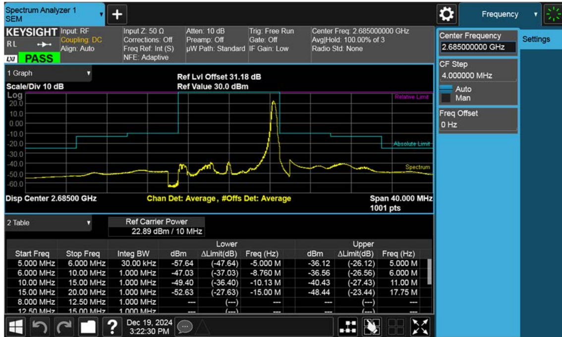
LTE B41_10 M_Channel Edge_High_QPSK_1RB
