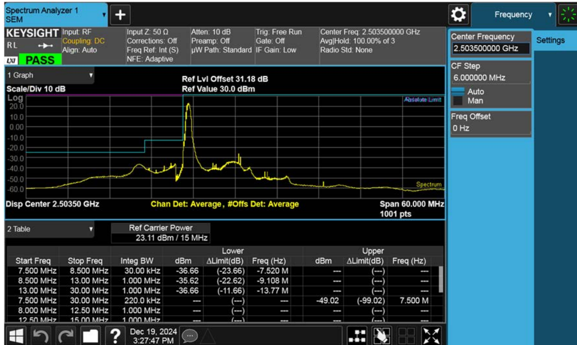
LTE B41_15 M_Channel Edge_Lower_Low_QPSK_1RB
