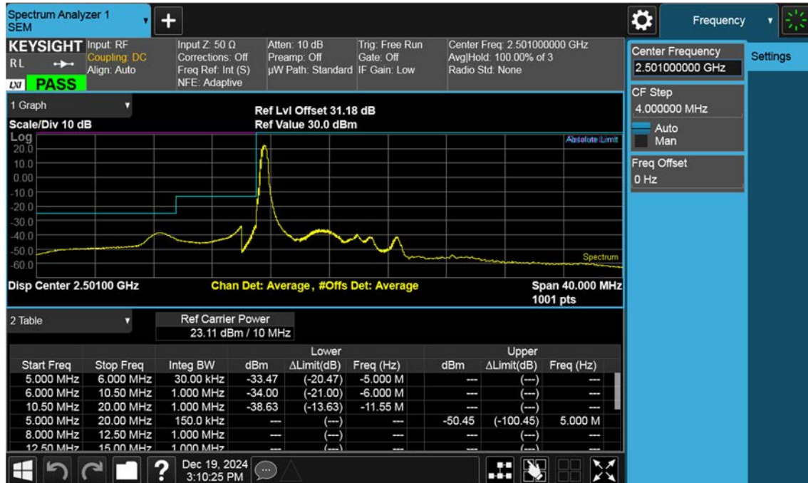
LTE B41_10 M_Channel Edge_Lower_Low_QPSK_1RB
