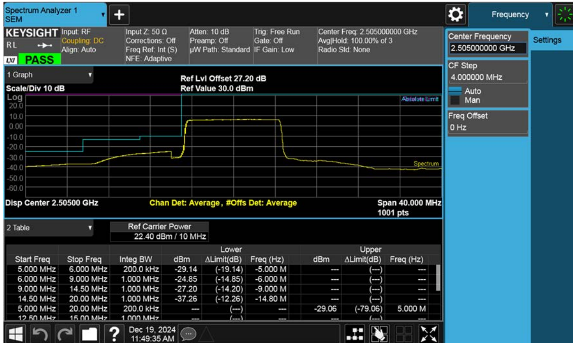
LTE B7_10 M_Channel Edge_Lower_Low_QPSK_FullIRB
