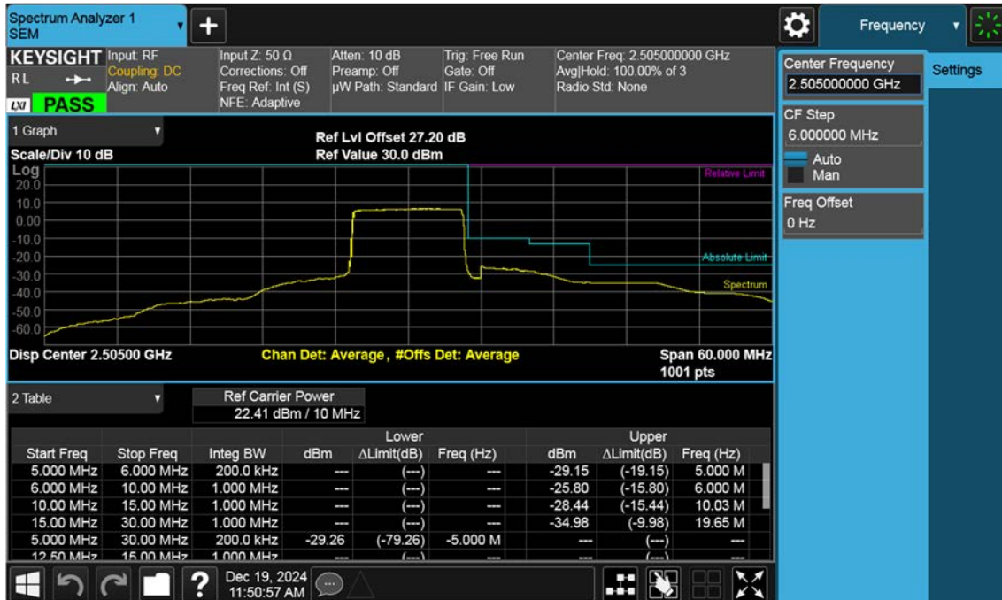
LTE B7_10 M_Channel Edge_Upper_Low_QPSK_FullRB
