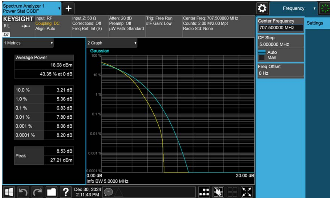
NR12_5 M_PAR_Mid_256QAM_FullRB
