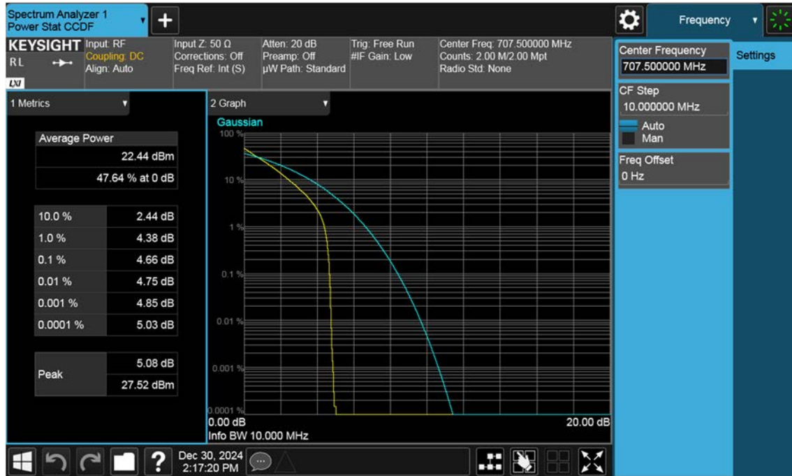
NR12_10 M_PAR_Mid_QPSK_FullRB
