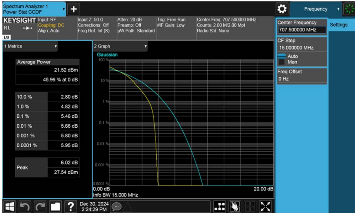
NR12_15 M_PAR_Mid_16QAM_FullRB
