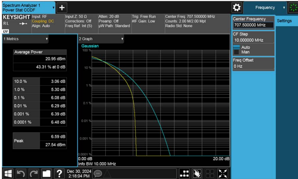
NR12_10 M_PAR_Mid_64QAM_FullRB
