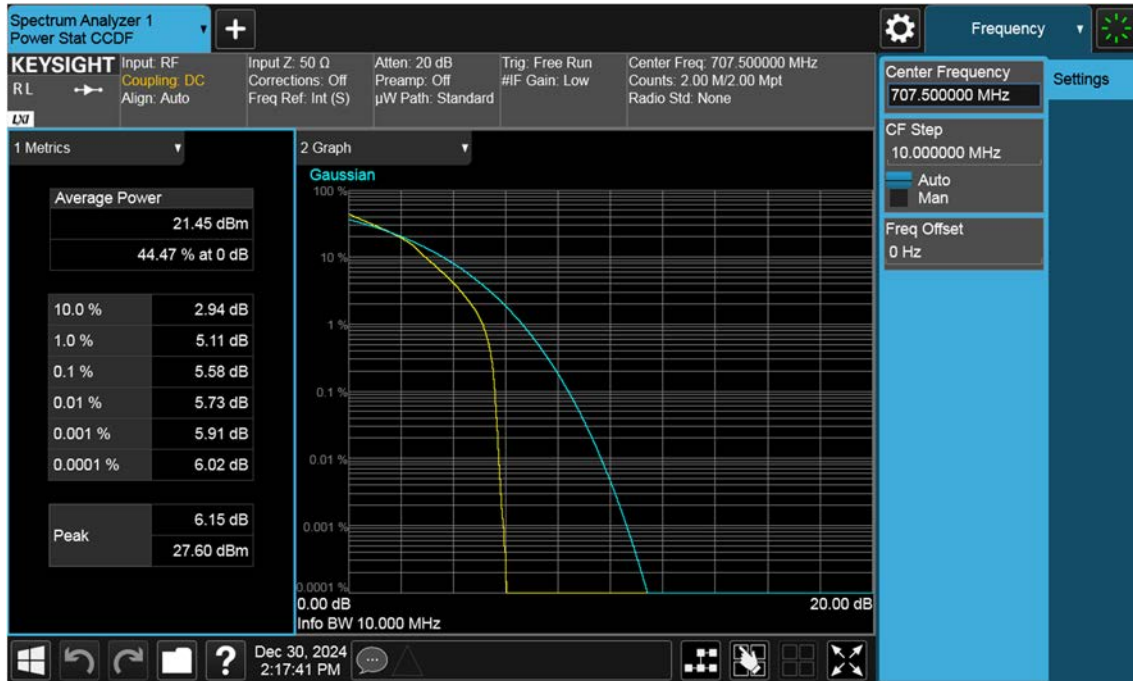
NR12_10 M_PAR_Mid_16QAM_FullRB
