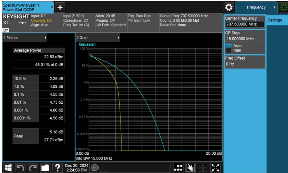
NR12_15 M_PAR_Mid_QPSK_FullRB
