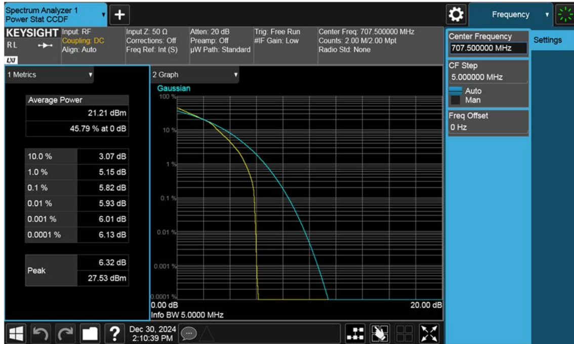
NR12_5 M_PAR_Mid_16QAM_FullRB
