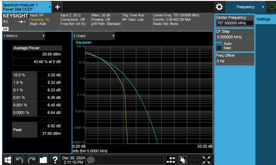
NR12_5 M_PAR_Mid_64QAM_FullRB
