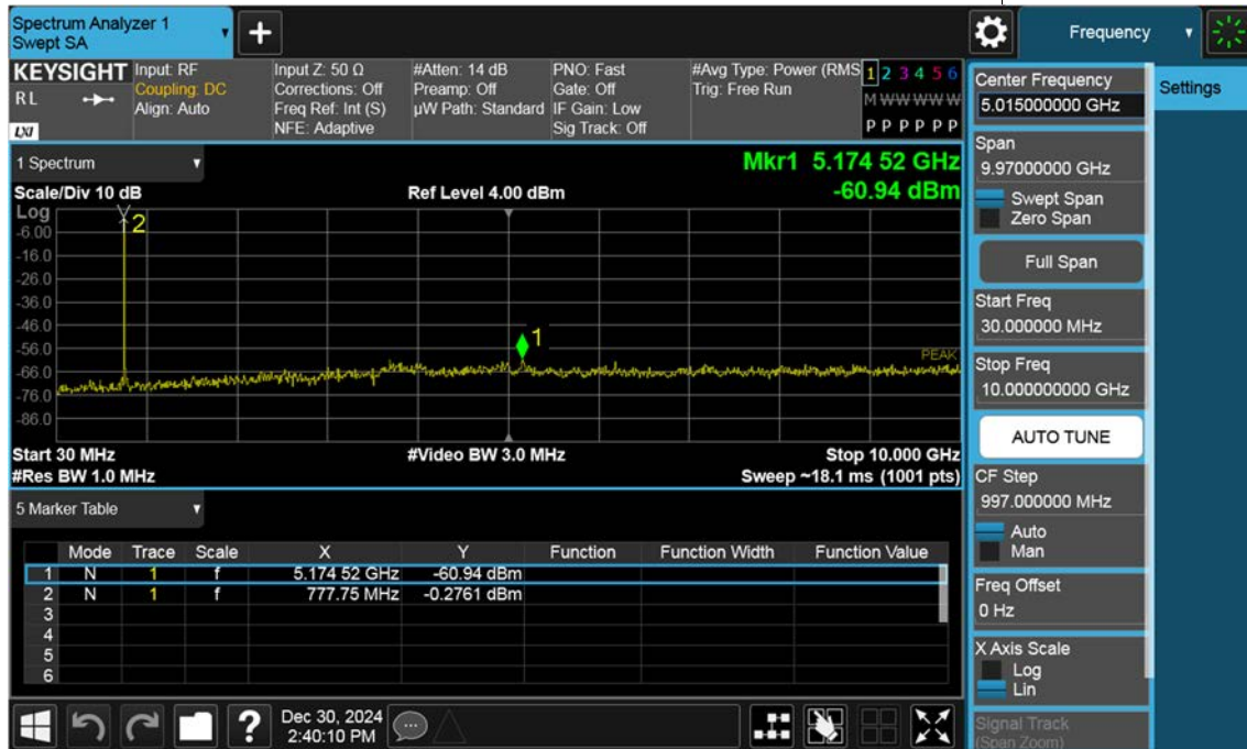
Sub6 n13_10 M_Conducted Spurious(30 M-10 G)_ BPSK_1RB
