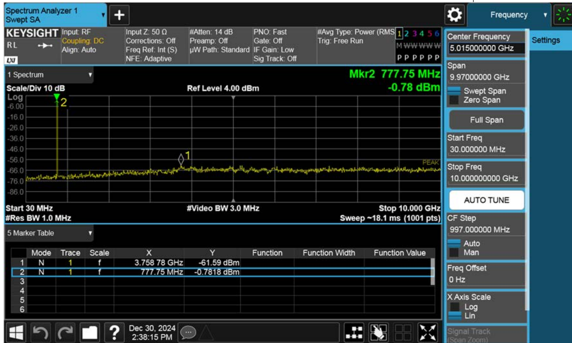
Sub6 n13_5 M_Conducted Spurious(30 M-10 G)_High_ BPSK_1RB
