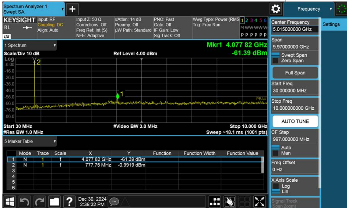
Sub6 n13_5 M_Conducted Spurious(30 M-10 G)_Mid_ BPSK_1RB
