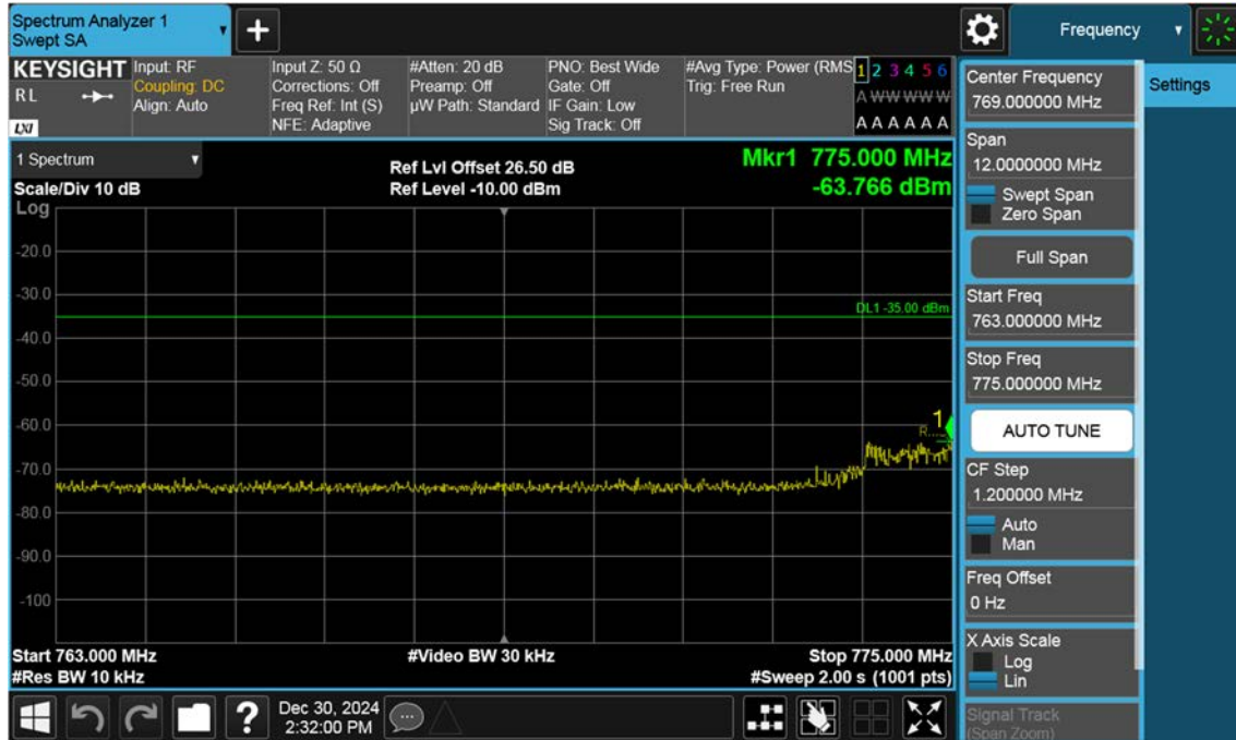
Sub6 n13_5 M_Extended Band Edge_Low_BPSK_FullRB
