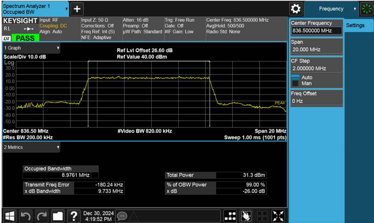
Occupied Bandwidth Plot (10 M BW Ch.167300 BPSK_RB 50_0)
