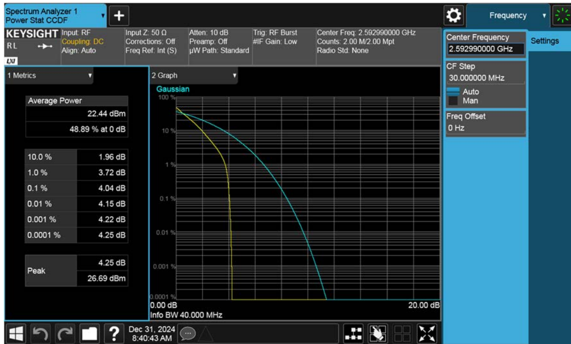
NR41_40 M_PAR_Mid_BPSK_FullIRB
