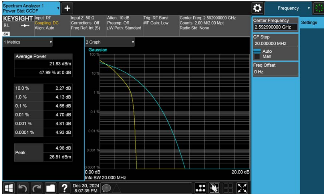
NR41_20 M_PAR_Mid_QPSK_FullRB
