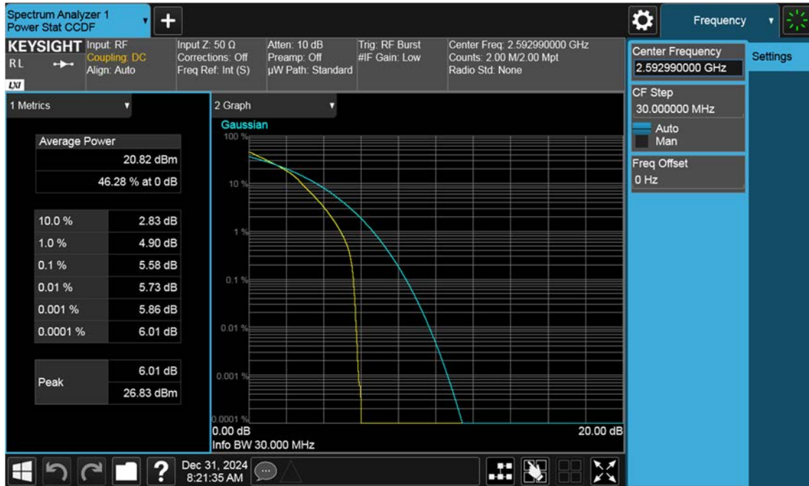
NR41_30 M_PAR_Mid_16QAM_FullRB
