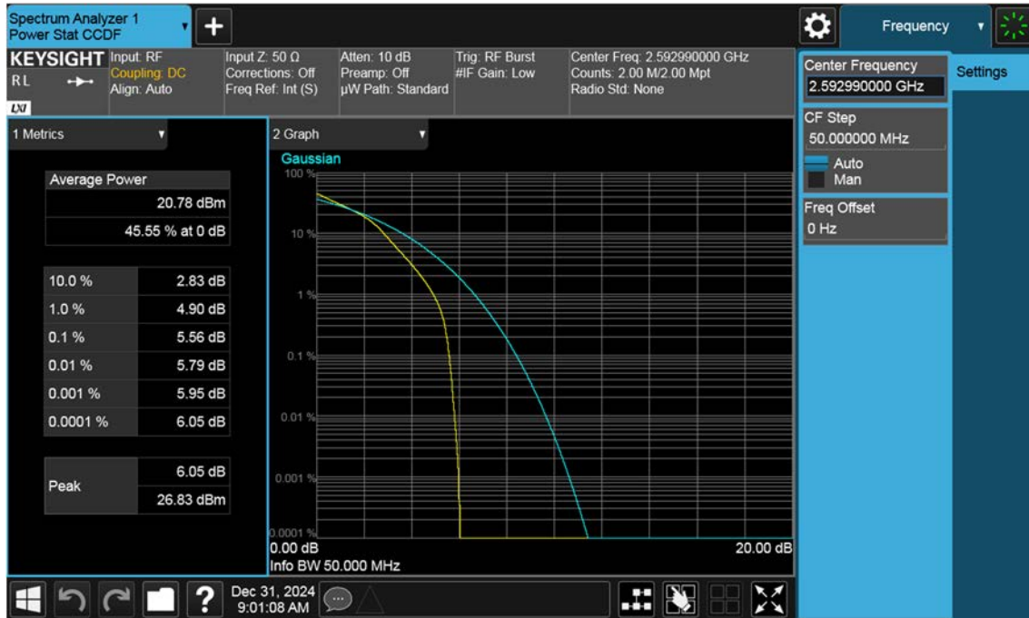
NR41_50 M_PAR_Mid_16QAM_FullRB
