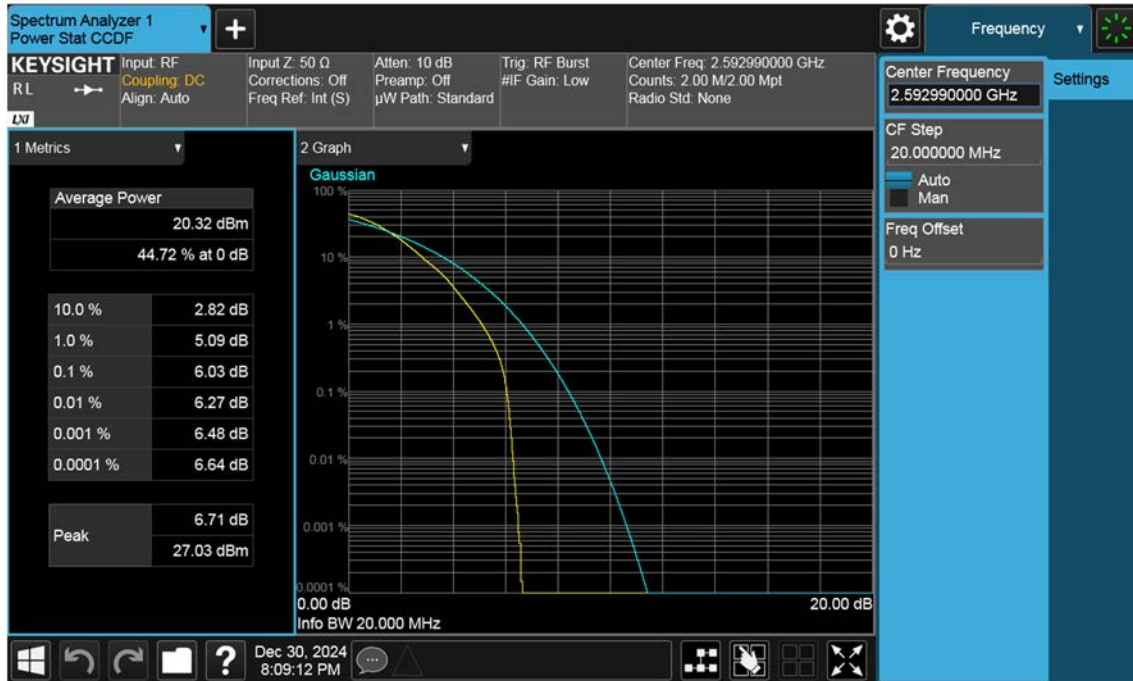
NR41_20 M_PAR_Mid_64QAM_FullRB
