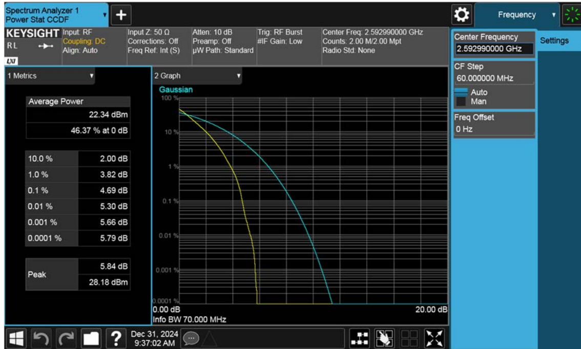
NR41_70 M_PAR_Mid_BPSK_FullIRB
