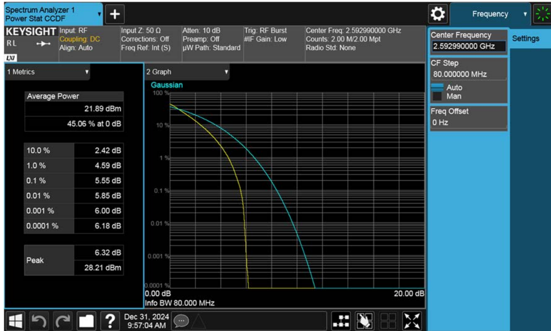
NR41_80 M_PAR_Mid_QPSK_FullRB
