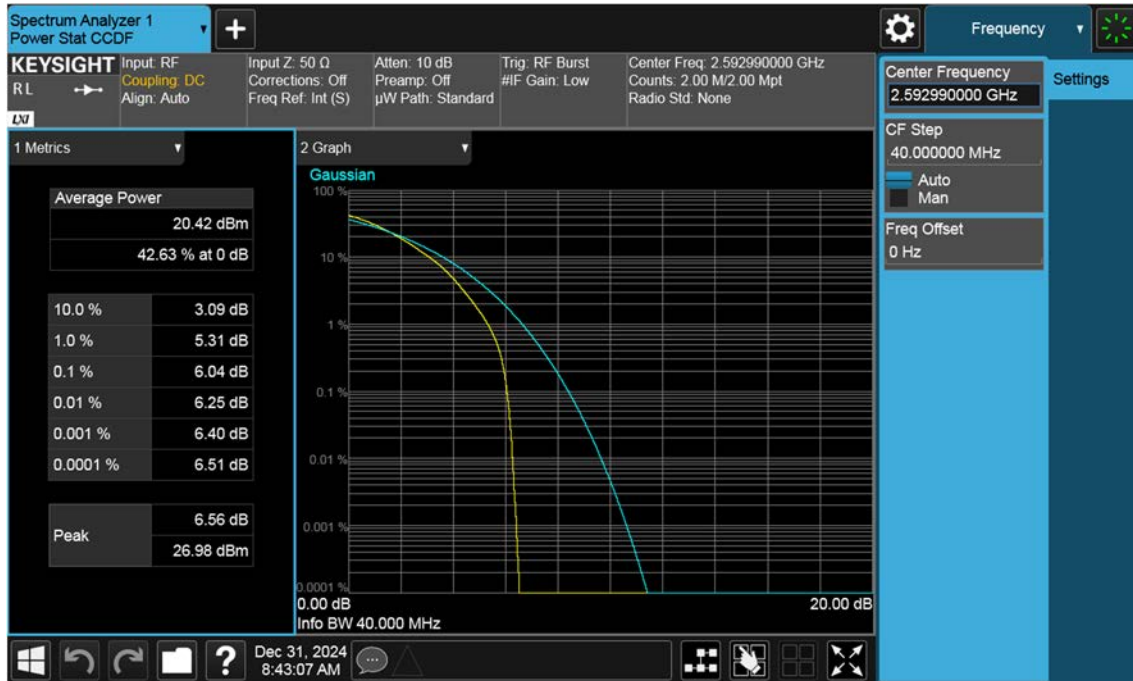
NR41_40 M_PAR_Mid_64QAM_FullRB
