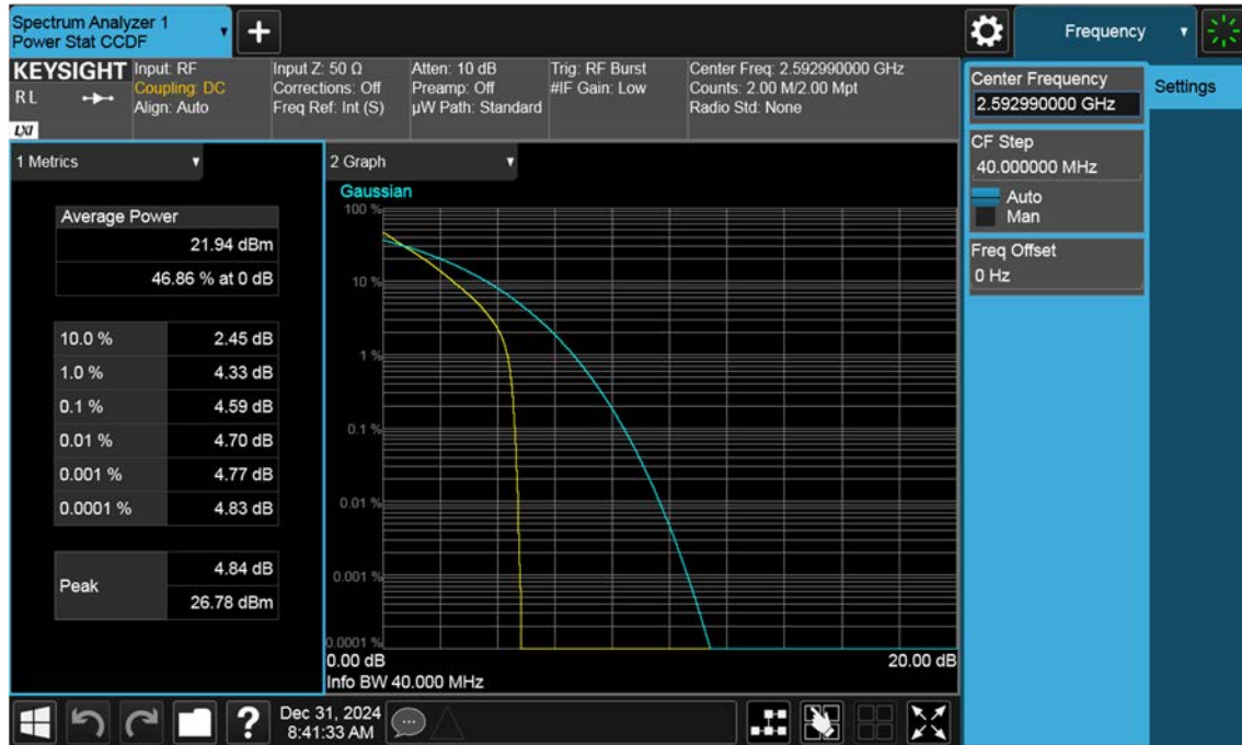
NR41_40 M_PAR_Mid_QPSK_FullRB
