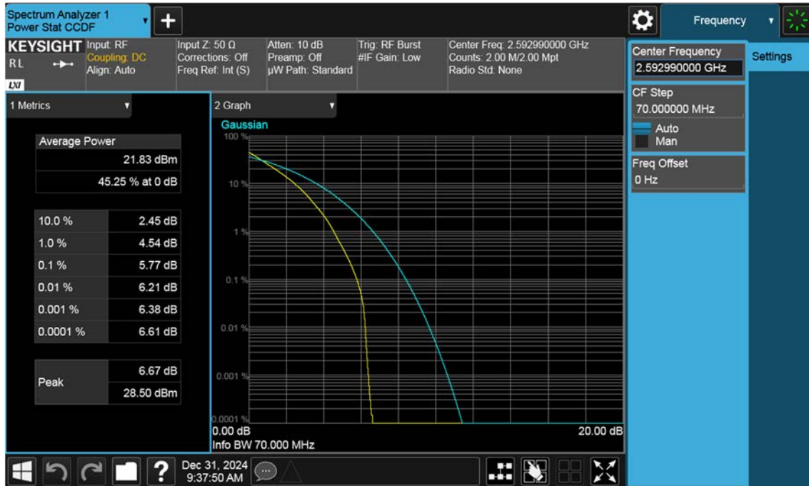
NR41_70 M_PAR_Mid_QPSK_FullRB
