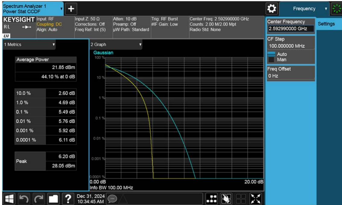
NR41_100 M_PAR_Mid_QPSK_FullRB
