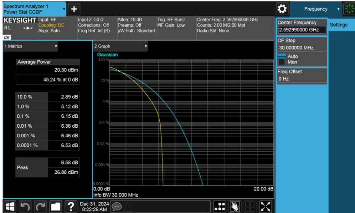
NR41_30 M_PAR_Mid_64QAM_FullRB
