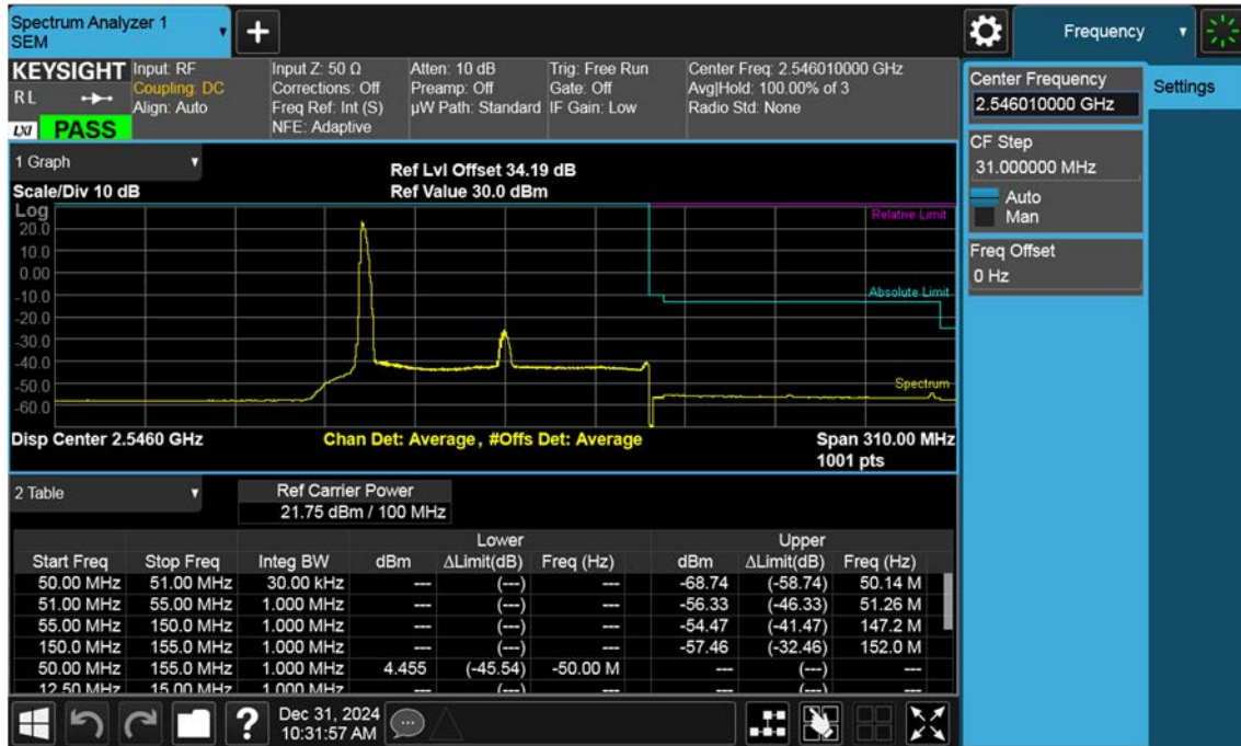
NR41_100 M_Band Edge_Upper_Low_BPSK_1RB
