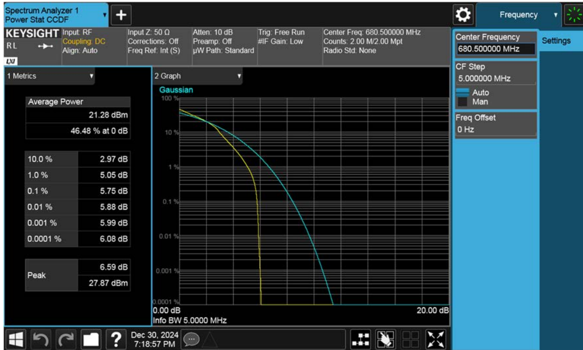
NR71_5 M_PAR_Mid_16QAM_FullRB
