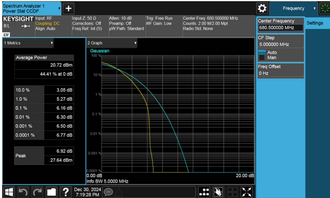
NR71_5 M_PAR_Mid_64QAM_FullRB
