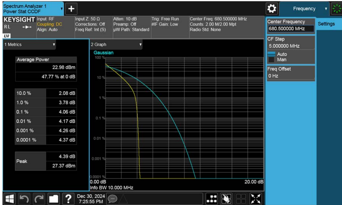
NR71_10 M_PAR_Mid_BPSK_FullIRB
