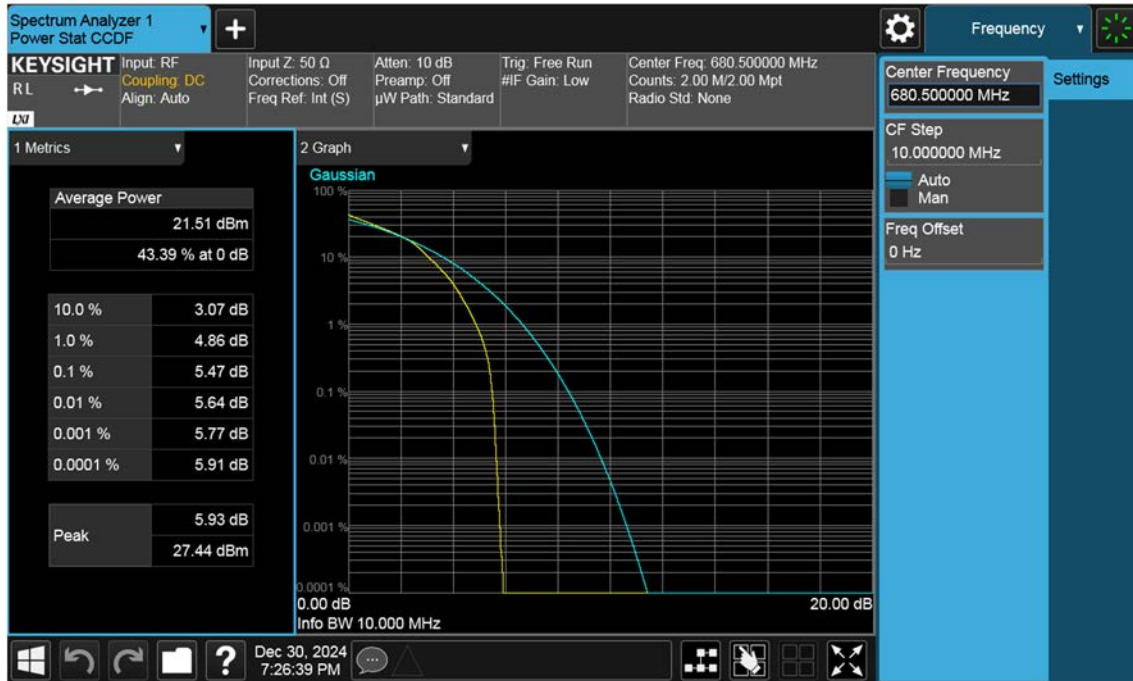
NR71_10 M_PAR_Mid_16QAM_FullRB
