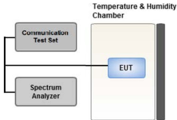
Test setup
